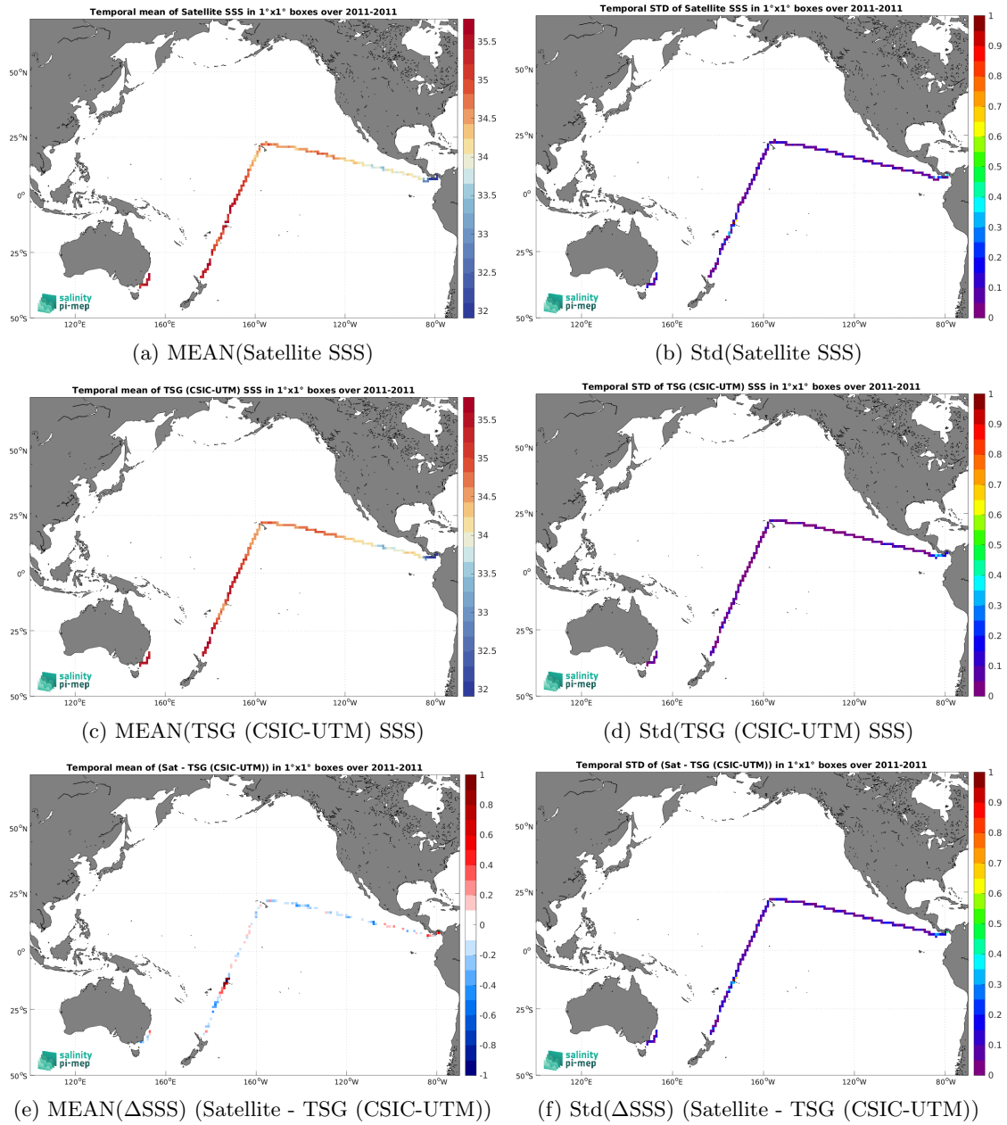
Figure 6: Temporal mean (left) and Std (right) of SSS from SMOS SSS L3 v8 - 9 Days (CATDS-CEC-LOCEAN) (top), TSG (CSIC-UTM) (middle), and of \Delta SSS (Satellite - TSG (CSIC-UTM)). Only match-up pairs are used to generate these maps.
