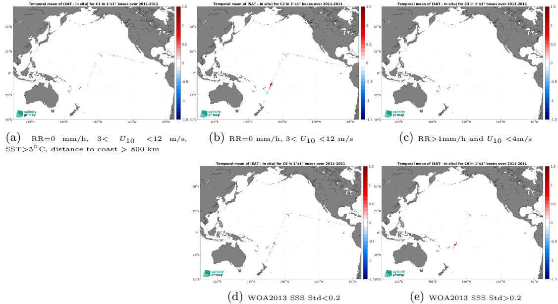
Figure 12: Temporal mean gridded over spatial boxes of size 1^{\circ}\times 1^{\circ} of \Delta\text{SSS} (SMOS SSS L3 v8 - 9 Days (CATDS-CEC-LOCEAN) - TSG (CSIC-UTM)) for 5 different subdatasets corresponding to:RR=0 mm/h, 3 < U_{10} < 12 m/s, SST >5^{\circ}\text{C} , distance to coast > 800 km (a), RR=0 mm/h, 3 < U_{10} < 12 m/s (b), RR >1 mm/h and U_{10} < 4 m/s (c), WOA2013 SSS Std <0.2 (d), WOA2013 SSS Std >0.2 (e).
