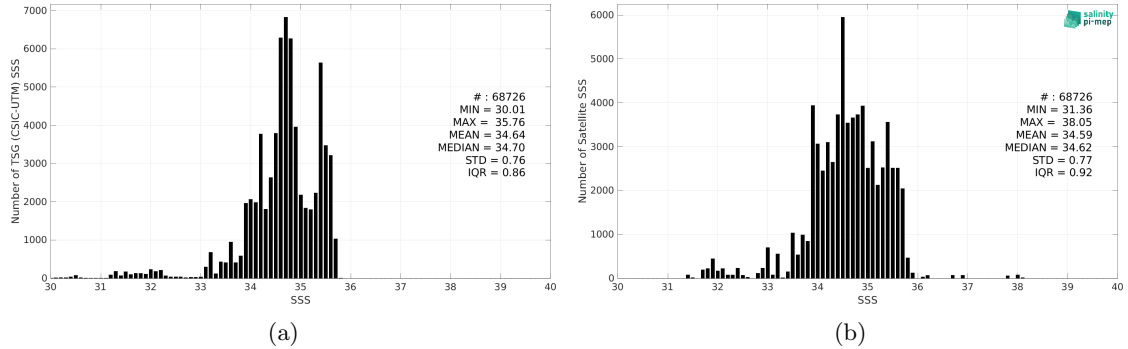
Figure 2: Histograms of SSS from TSG (CSIC-UTM) (a) and SMOS SSS L3 v8 - 9 Days (CATDS-CEC-LOCEAN) (b) considering all match-up pairs per bins of 0.1 over the Pacific Ocean Pi-MEP region and for the full satellite product period.
