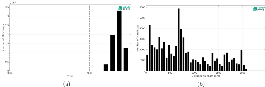
Figure 1: Number of match-ups between TSG (CSIC-UTM) and SMOS SSS L3 v8 - 9 Days (CATDS-CEC-LOCEAN) SSS as a function of time (a) and as function of the distance to coast (b) over the Pacific Ocean Pi-MEP region and for the full satellite product period.
