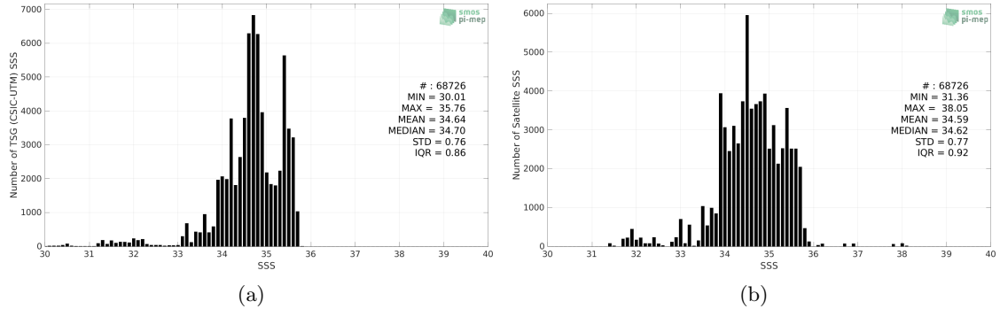
Figure 2: Histograms of SSS from TSG (CSIC-UTM) (a) and SMOS SSS L3 v8 - 9 Days (CATDS-CECOS-LOCEAN) (b) considering all match-up pairs per bins of 0.1 over the Pacific Ocean Pi-MEP region and for the full satellite product period.
