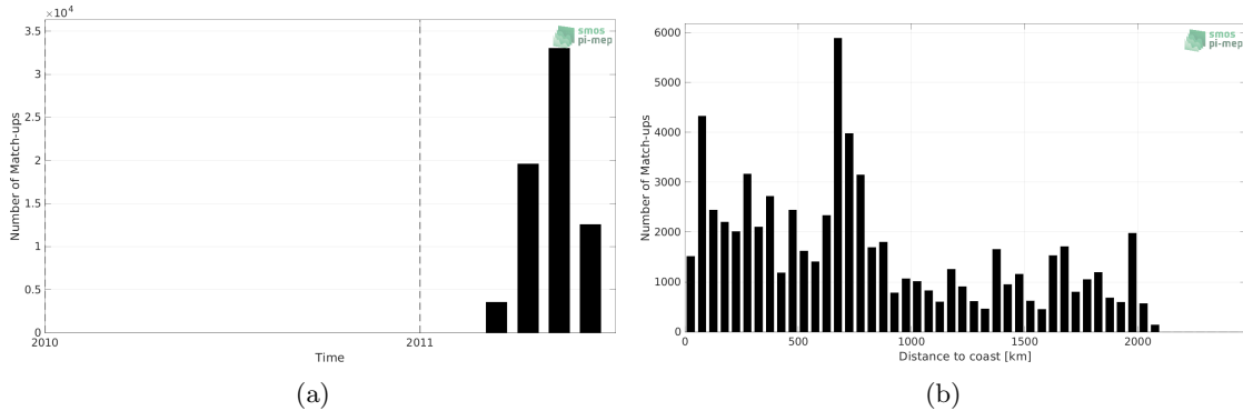
Figure 1: Number of match-ups between TSG (CSIC-UTM) and SMOS SSS L3 v8 - 9 Days (CATDS-CECOS-LOCEAN) SSS as a function of time (a) and as function of the distance to coast (b) over the Pacific Ocean Pi-MEP region and for the full satellite product period.
