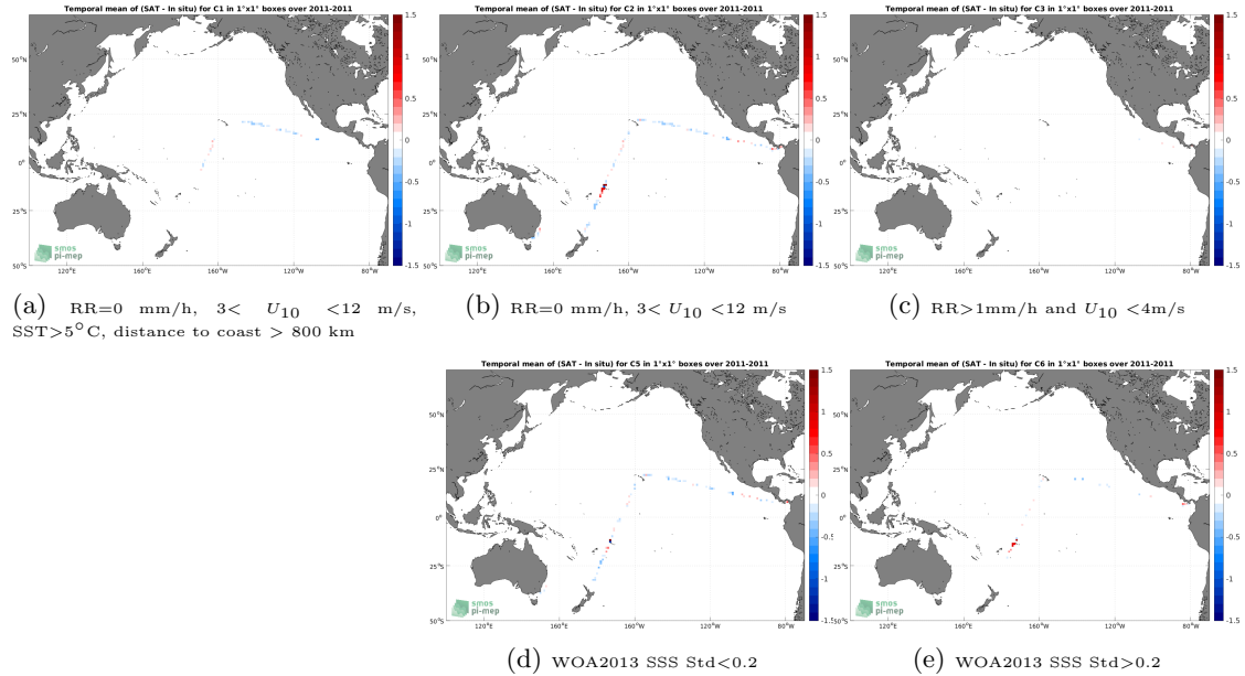
Figure 12: Temporal mean gridded over spatial boxes of size 1^{\circ}\times 1^{\circ} of \Delta\text{SSS} (SMOS SSS L3 v8 - 9 Days (CATDS-CECOS-LOCEAN) - TSG (CSIC-UTM)) for 5 different subdatasets corresponding to:RR=0 mm/h, 3 < U_{10} < 12 m/s, SST >5^{\circ}\text{C} , distance to coast > 800 km (a), RR=0 mm/h, 3 < U_{10} < 12 m/s (b), RR >1 mm/h and U_{10} < 4 m/s (c), WOA2013 SSS Std <0.2 (d), WOA2013 SSS Std >0.2 (e).
