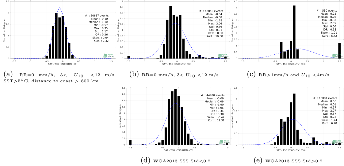
Figure 13: Normalized histogram of \Delta SSS (SMOS SSS L3 v8 - 9 Days (CATDS-CECOS-LOCEAN) - TSG (CSIC-UTM)) for 5 different subdatasets corresponding to: RR=0 mm/h, 3 < U_{10} < 12 m/s, SST>5°C, distance to coast > 800 km (a), RR=0 mm/h, 3 < U_{10} < 12 m/s (b), RR>1mm/h and U_{10} < 4 m/s (c), WOA2013 SSS Std<0.2 (d), WOA2013 SSS Std>0.2 (e).
