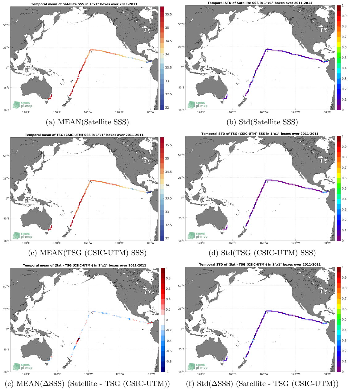
Figure 6: Temporal mean (left) and Std (right) of SSS from SMOS SSS L3 v8 - 9 Days (CATDS-CECOS-LOCEAN) (top), TSG (CSIC-UTM) (middle), and of \Delta SSS (Satellite - TSG (CSIC-UTM)). Only match-up pairs are used to generate these maps.
