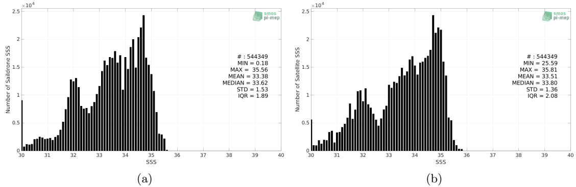
Figure 2: Histograms of SSS from Saildrone (a) and SMOS SSS L3 v8 - 9 Days (CATDS-CECOS-LOCEAN) (b) considering all match-up pairs per bins of 0.1 over the Pacific Ocean Pi-MEP region and for the full satellite product period.
