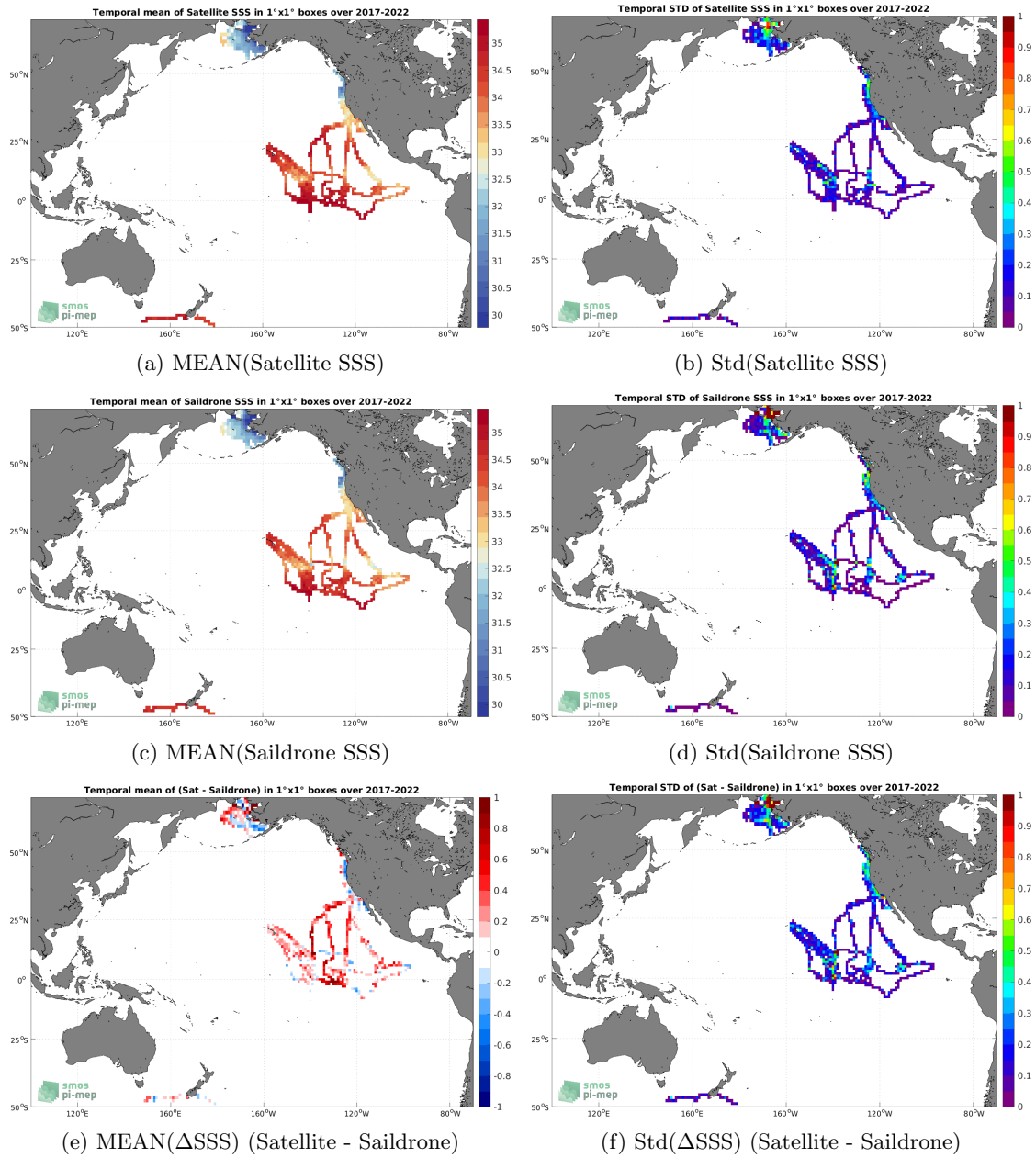
Figure 6: Temporal mean (left) and Std (right) of SSS from SMOS SSS L3 v8 - 9 Days (CATDS-CECOS-LOCEAN) (top), Saildrone (middle), and of \Delta SSS (Satellite - Saildrone). Only match-up pairs are used to generate these maps.
