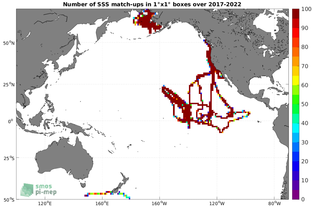
Figure 4: Number of SSS match-ups between Saildrone SSS and the SMOS SSS L3 v8 - 9 Days (CATDS-CECOS-LOCEAN) SSS product for the Pacific Ocean Pi-MEP region over 1^\circ \times 1^\circ boxes and for the full satellite product period.
