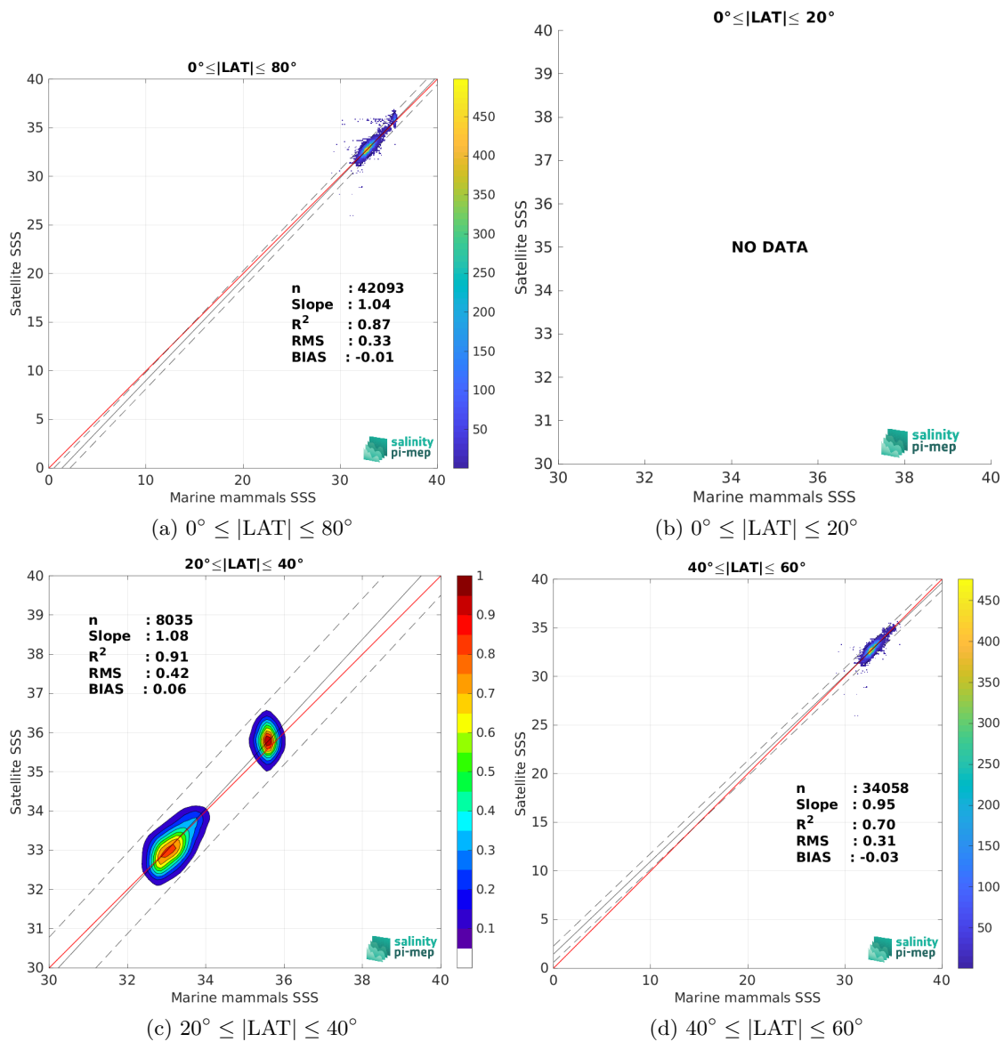
Figure 9: Contour maps of the concentration of SMOS SSS L3 v8 - 9 Days (CATDS-CEC-LOCEAN) SSS ( y -axis) versus Marine mammals SSS ( x -axis) at match-up pairs for different latitude bands. For each plot, the red line shows x=y . The black thin and dashed lines indicate a linear fit through the data cloud and the \pm 95\% confidence levels, respectively. The number match-up pairs n , the slope and R^2 coefficient of the linear fit, the root mean square (RMS) and the mean bias between satellite and in situ data are indicated for each latitude band in each plots.
