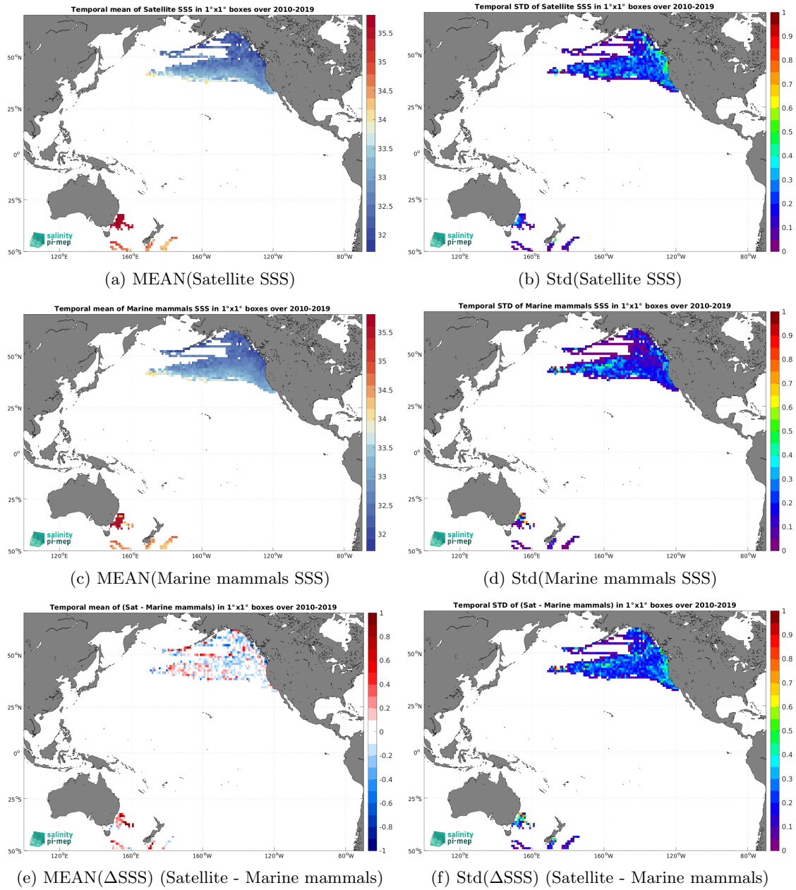
Figure 6: Temporal mean (left) and Std (right) of SSS from SMOS SSS L3 v8 - 9 Days (CATDS-CEC-LOCEAN) (top), Marine mammals (middle), and of \Delta SSS (Satellite - Marine mammals). Only match-up pairs are used to generate these maps.
