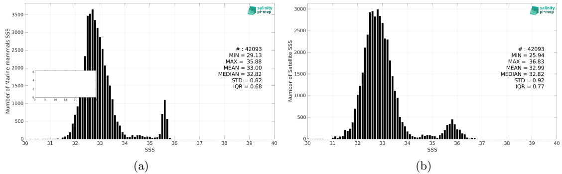
Figure 2: Histograms of SSS from Marine mammals (a) and SMOS SSS L3 v8 - 9 Days (CATDS-CEC-LOCEAN) (b) considering all match-up pairs per bins of 0.1 over the Pacific Ocean Pi-MEP region and for the full satellite product period.
