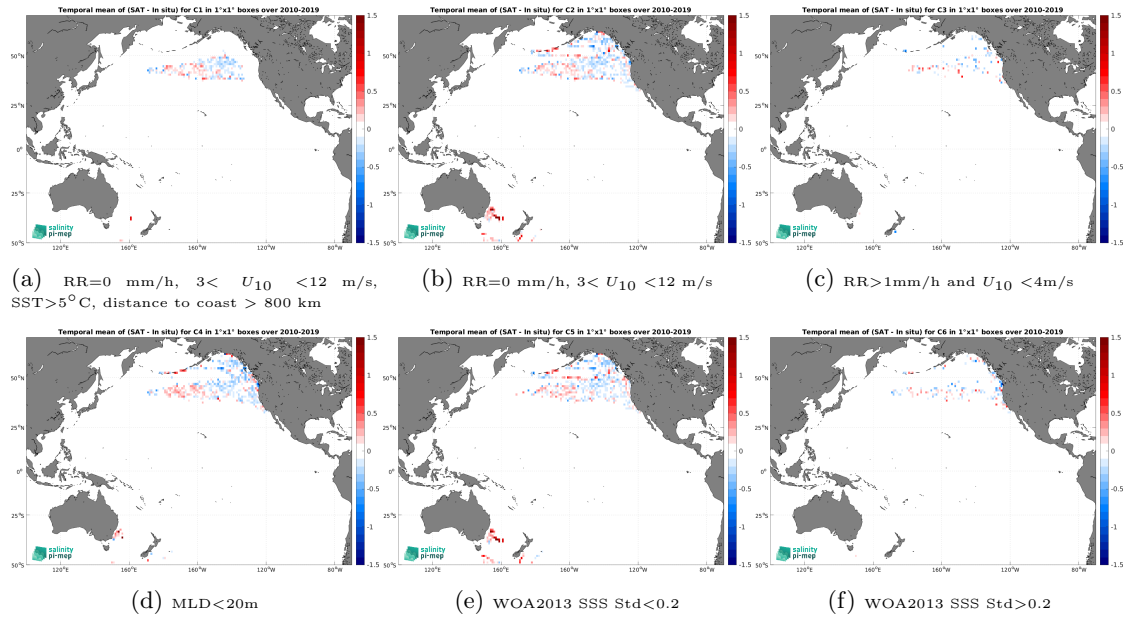
Figure 12: Temporal mean gridded over spatial boxes of size 1^{\circ}\times 1^{\circ} of \Delta\text{SSS} (SMOS SSS L3 v8 - 9 Days (CATDS-CEC-LOCEAN) - Marine mammals) for 6 different subdatasets corresponding to: RR=0 mm/h, 3 < U_{10} < 12 m/s, SST > 5^{\circ}\text{C} , distance to coast > 800 km (a), RR=0 mm/h, 3 < U_{10} < 12 m/s (b), RR > 1\text{mm/h} and U_{10} < 4\text{m/s} (c), MLD < 20\text{m} (d), WOA2013 SSS Std < 0.2 (e), WOA2013 SSS Std > 0.2 (f).
