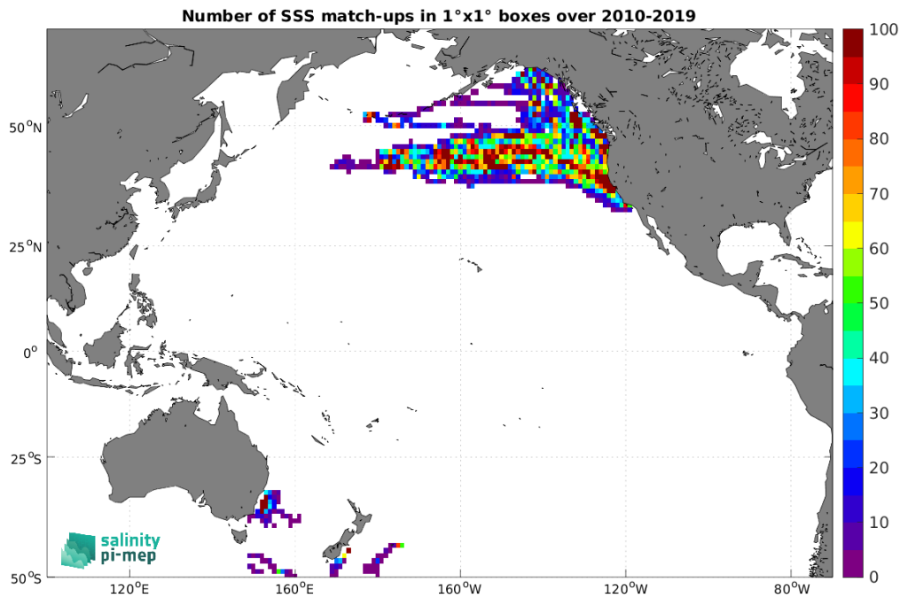
Figure 4: Number of SSS match-ups between Marine mammals SSS and the SMOS SSS L3 v8 - 9 Days (CATDS-CEC-LOCEAN) SSS product for the Pacific Ocean Pi-MEP region over 1^\circ \times 1^\circ boxes and for the full satellite product period.
