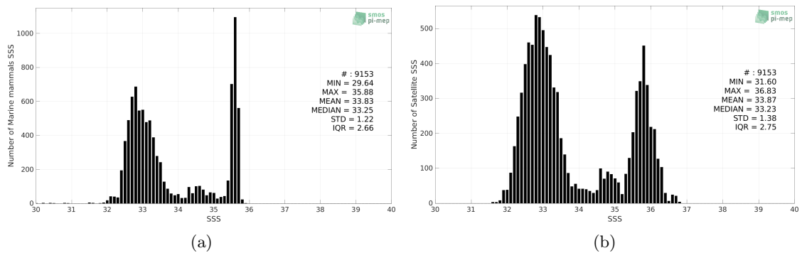
Figure 2: Histograms of SSS from Marine mammals (a) and SMOS SSS L3 v8 - 9 Days (CATDS-CECOS-LOCEAN) (b) considering all match-up pairs per bins of 0.1 over the Pacific Ocean Pi-MEP region and for the full satellite product period.
