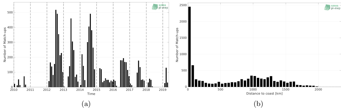
Figure 1: Number of match-ups between Marine mammals and SMOS SSS L3 v8 - 9 Days (CATDS-CECOS-LOCEAN) SSS as a function of time (a) and as function of the distance to coast (b) over the Pacific Ocean Pi-MEP region and for the full satellite product period.
