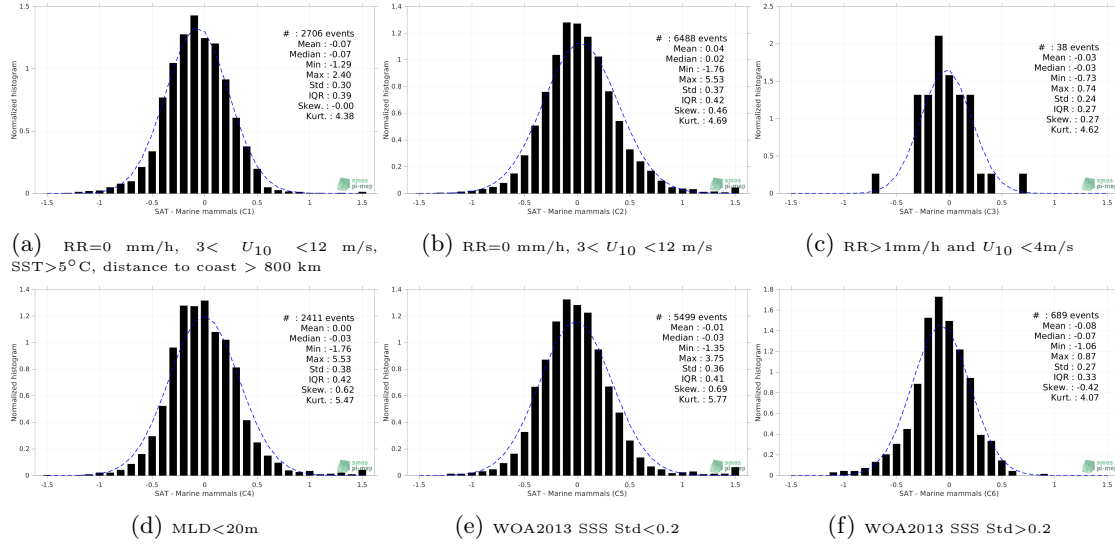
Figure 13: Normalized histogram of \Delta SSS (SMOS SSS L3 v8 - 9 Days (CATDS-CECOS-LOCEAN) - Marine mammals) for 6 different subdatasets corresponding to: RR=0 mm/h, 3 < U_{10} < 12 m/s, SST > 5°C, distance to coast > 800 km (a), RR=0 mm/h, 3 < U_{10} < 12 m/s (b), RR > 1mm/h and U_{10} < 4 m/s (c), MLD < 20m (d), WOA2013 SSS Std < 0.2 (e), WOA2013 SSS Std > 0.2 (f).
