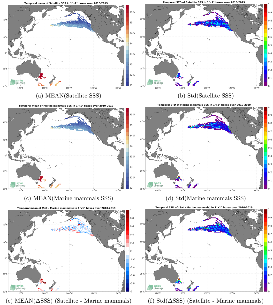
Figure 6: Temporal mean (left) and Std (right) of SSS from SMOS SSS L3 v8 - 9 Days (CATDS-CECOS-LOCEAN) (top), Marine mammals (middle), and of \Delta SSS (Satellite - Marine mammals). Only match-up pairs are used to generate these maps.
