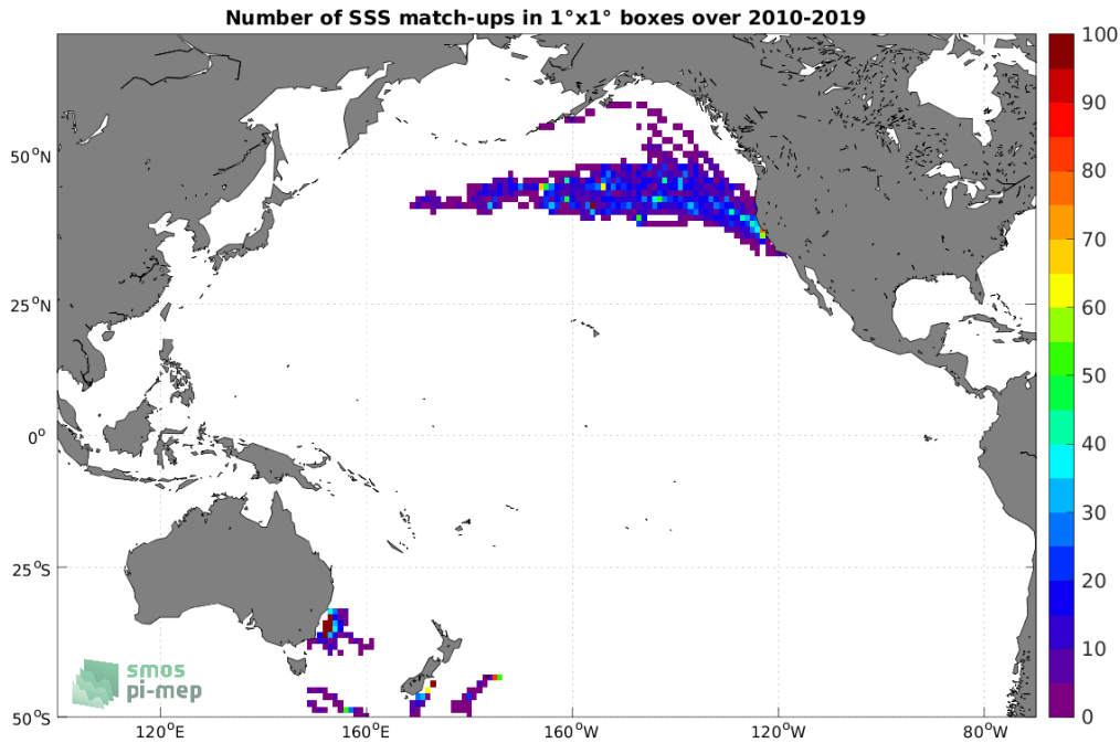
Figure 4: Number of SSS match-ups between Marine mammals SSS and the SMOS SSS L3 v8 - 9 Days (CATDS-CECOS-LOCEAN) SSS product for the Pacific Ocean Pi-MEP region over 1^\circ \times 1^\circ boxes and for the full satellite product period.
