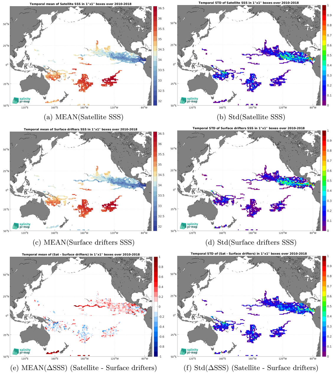
Figure 5: Temporal mean (left) and Std (right) of SSS from SMOS SSS L3 v8 - 9 Days (CATDS-CEC-LOCEAN) (top), Surface drifters (middle), and of \Delta SSS (Satellite - Surface drifters). Only match-up pairs are used to generate these maps.
