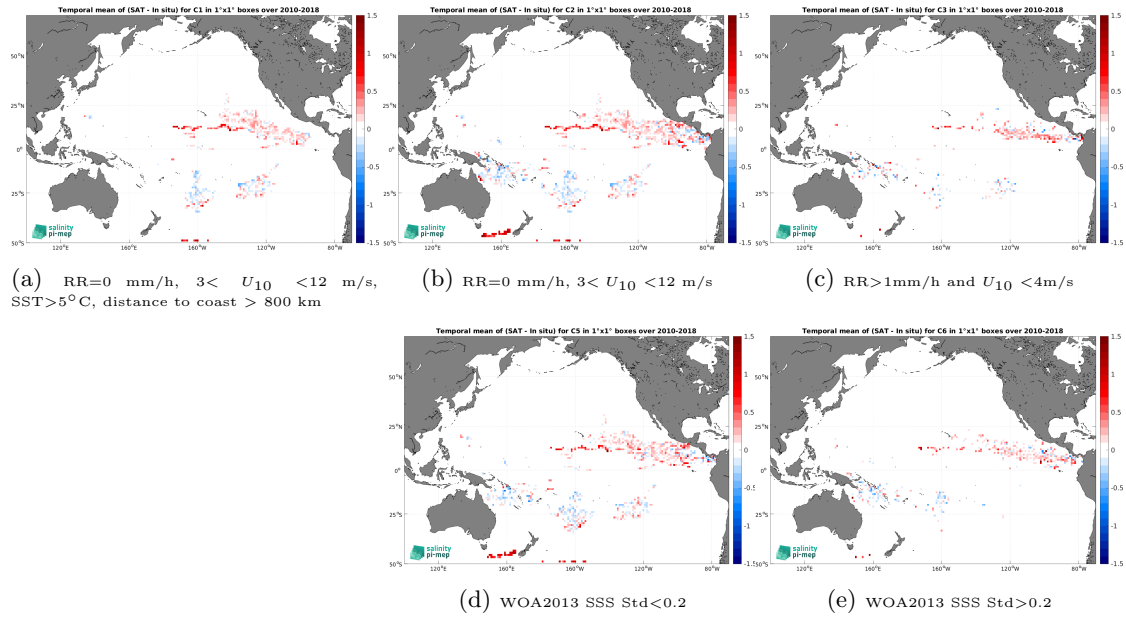
Figure 11: Temporal mean gridded over spatial boxes of size 1^\circ \times 1^\circ of \Delta SSS (SMOS SSS L3 v8 - 9 Days (CATDS-CEC-LOCEAN) - Surface drifters) for 5 different subdatasets corresponding to:RR=0 mm/h, 3 < U_{10} < 12 m/s, SST >5^\circ C, distance to coast > 800 km (a), RR=0 mm/h, 3 < U_{10} < 12 m/s (b), RR >1 mm/h and U_{10} < 4 m/s (c), WOA2013 SSS Std <0.2 (d), WOA2013 SSS Std >0.2 (e).
