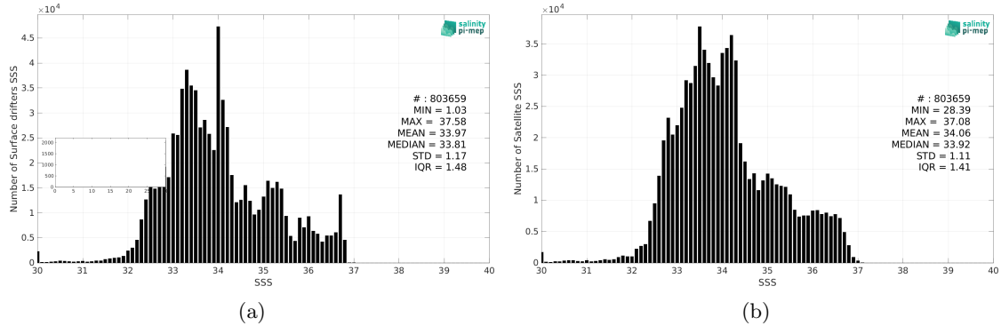
Figure 2: Histograms of SSS from Surface drifters (a) and SMOS SSS L3 v8 - 9 Days (CATDS-CEC-LOCEAN) (b) considering all match-up pairs per bins of 0.1 over the Pacific Ocean Pi-MEP region and for the full satellite product period.
