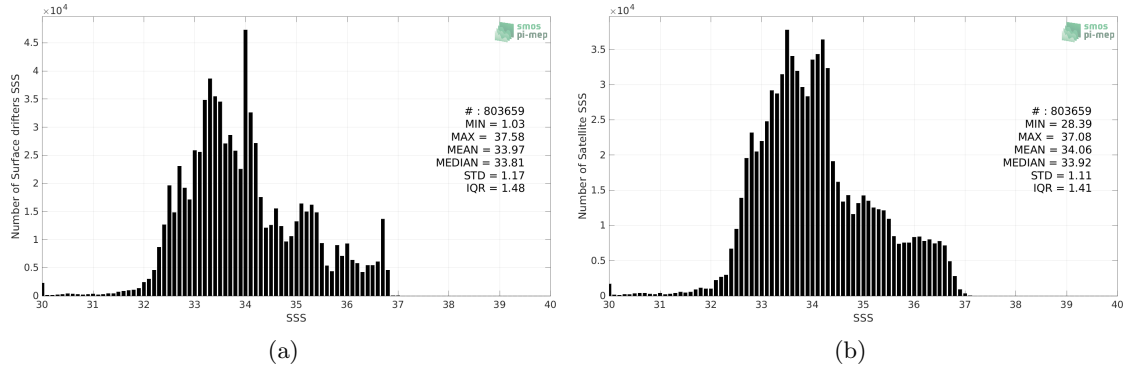
Figure 2: Histograms of SSS from Surface drifters (a) and SMOS SSS L3 v8 - 9 Days (CATDS-CECOS-LOCEAN) (b) considering all match-up pairs per bins of 0.1 over the Pacific Ocean Pi-MEP region and for the full satellite product period.
