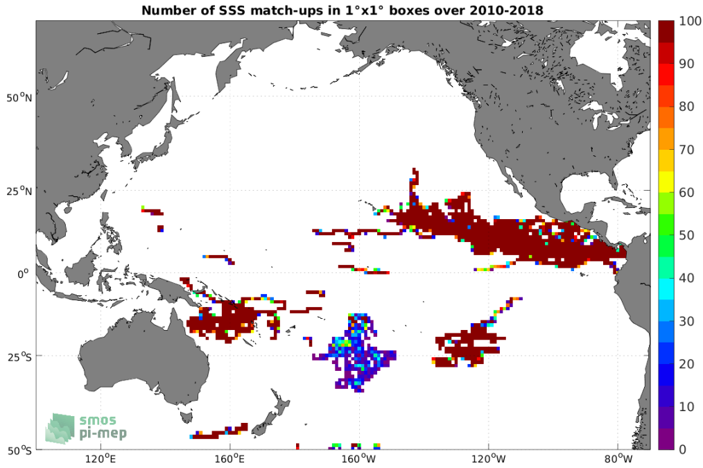
Figure 3: Number of SSS match-ups between Surface drifters SSS and the SMOS SSS L3 v8 - 9 Days (CATDS-CECOS-LOCEAN) SSS product for the Pacific Ocean Pi-MEP region over 1^\circ \times 1^\circ boxes and for the full satellite product period.
