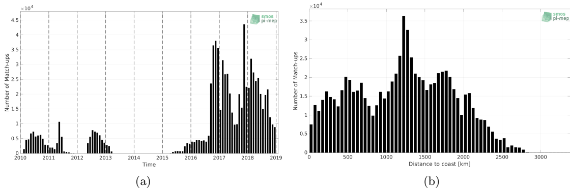
Figure 1: Number of match-ups between Surface drifters and SMOS SSS L3 v8 - 9 Days (CATDS-CECOS-LOCEAN) SSS as a function of time (a) and as function of the distance to coast (b) over the Pacific Ocean Pi-MEP region and for the full satellite product period.
