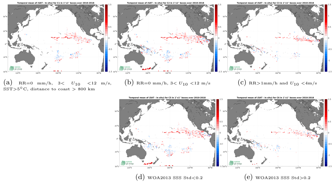
Figure 11: Temporal mean gridded over spatial boxes of size 1^\circ \times 1^\circ of \Delta SSS (SMOS SSS L3 v8 - 9 Days (CATDS-CECOS-LOCEAN) - Surface drifters) for 5 different subdatasets corresponding to:RR=0 mm/h, 3 < U_{10} < 12 m/s, SST >5^\circ C, distance to coast > 800 km (a), RR=0 mm/h, 3 < U_{10} < 12 m/s (b), RR >1 mm/h and U_{10} < 4 m/s (c), WOA2013 SSS Std <0.2 (d), WOA2013 SSS Std >0.2 (e).
