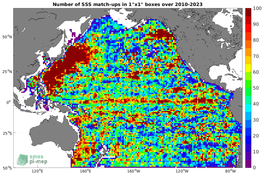
Figure 4: Number of SSS match-ups between Argo SSS and the SMOS SSS L3 v8 - 9 Days (CATDS-CECOS-LOCEAN) SSS product for the Pacific Ocean Pi-MEP region over 1^\circ \times 1^\circ boxes and for the full satellite product period.
