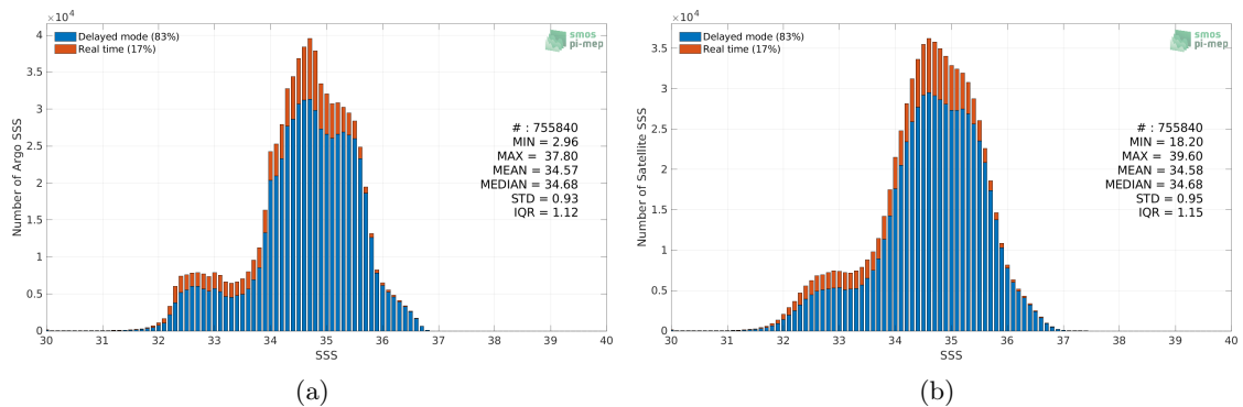
Figure 2: Histograms of SSS from Argo (a) and SMOS SSS L3 v8 - 9 Days (CATDS-CECOS-LOCEAN) (b) considering all match-up pairs per bins of 0.1 over the Pacific Ocean Pi-MEP region and for the full satellite product period.
