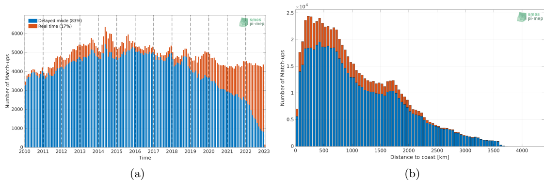
Figure 1: Number of match-ups between Argo and SMOS SSS L3 v8 - 9 Days (CATDS-CECOS-LOCEAN) SSS as a function of time (a) and as function of the distance to coast (b) over the Pacific Ocean Pi-MEP region and for the full satellite product period.
