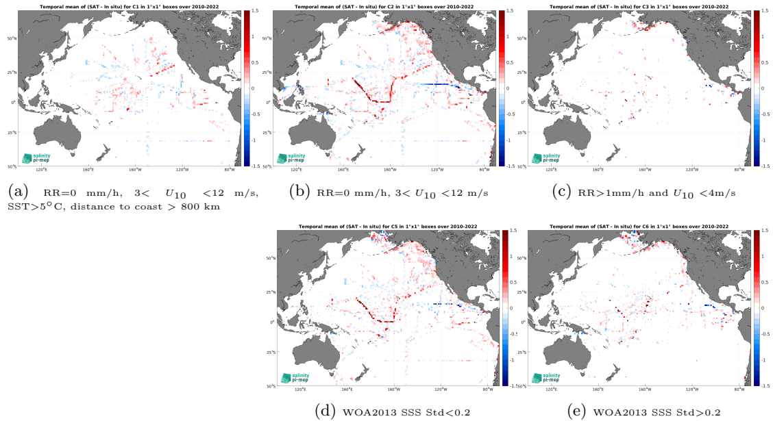
Figure 12: Temporal mean gridded over spatial boxes of size 1^\circ \times 1^\circ of \Delta SSS (SMOS SSS L3 v8 - 18 Days (CATDS-CEC-LOCEAN) - TSG (SAMOS)) for 5 different subdatasets corresponding to:RR=0 mm/h, 3 < U_{10} < 12 m/s, SST >5^\circ C, distance to coast > 800 km (a), RR=0 mm/h, 3 < U_{10} < 12 m/s (b), RR >1 mm/h and U_{10} < 4 m/s (c), WOA2013 SSS Std <0.2 (d), WOA2013 SSS Std >0.2 (e).
