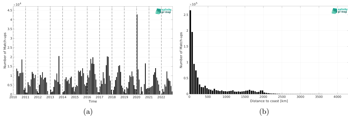
Figure 1: Number of match-ups between TSG (SAMOS) and SMOS SSS L3 v8 - 18 Days (CATDS-CEC-LOCEAN) SSS as a function of time (a) and as function of the distance to coast (b) over the Pacific Ocean Pi-MEP region and for the full satellite product period.
