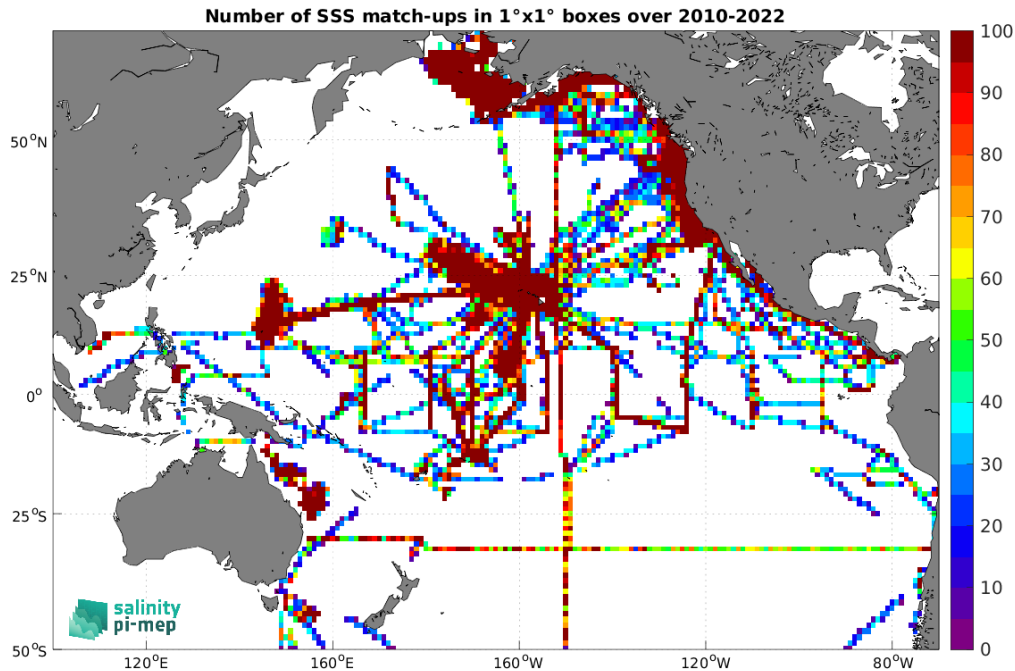
Figure 4: Number of SSS match-ups between TSG (SAMOS) SSS and the SMOS SSS L3 v8 - 18 Days (CATDS-CEC-LOCEAN) SSS product for the Pacific Ocean Pi-MEP region over 1^\circ \times 1^\circ boxes and for the full satellite product period.
