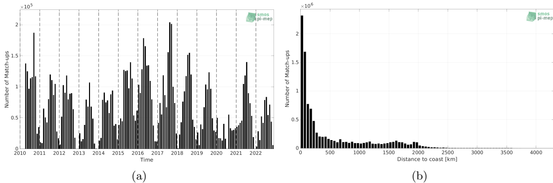
Figure 1: Number of match-ups between TSG (SAMOS) and SMOS SSS L3 v8 - 18 Days (CATDS-CECOS-LOCEAN) SSS as a function of time (a) and as function of the distance to coast (b) over the Pacific Ocean Pi-MEP region and for the full satellite product period.
