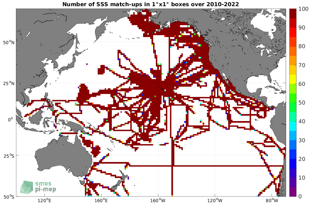
Figure 4: Number of SSS match-ups between TSG (SAMOS) SSS and the SMOS SSS L3 v8 - 18 Days (CATDS-CECOS-LOCEAN) SSS product for the Pacific Ocean Pi-MEP region over 1^\circ \times 1^\circ boxes and for the full satellite product period.
