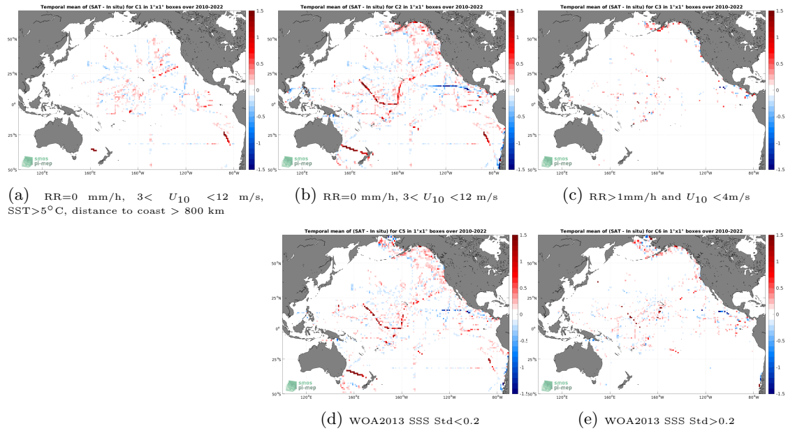
Figure 12: Temporal mean gridded over spatial boxes of size 1^\circ \times 1^\circ of \Delta SSS (SMOS SSS L3 v8 - 18 Days (CATDS-CECOS-LOCEAN) - TSG (SAMOS)) for 5 different subdatasets corresponding to:RR=0 mm/h, 3 < U_{10} < 12 m/s, SST >5^\circ C, distance to coast > 800 km (a), RR=0 mm/h, 3 < U_{10} < 12 m/s (b), RR >1 mm/h and U_{10} < 4 m/s (c), WOA2013 SSS Std <0.2 (d), WOA2013 SSS Std >0.2 (e).
