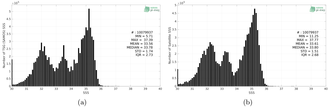
Figure 2: Histograms of SSS from TSG (SAMOS) (a) and SMOS SSS L3 v8 - 18 Days (CATDS-CECOS-LOCEAN) (b) considering all match-up pairs per bins of 0.1 over the Pacific Ocean Pi-MEP region and for the full satellite product period.
