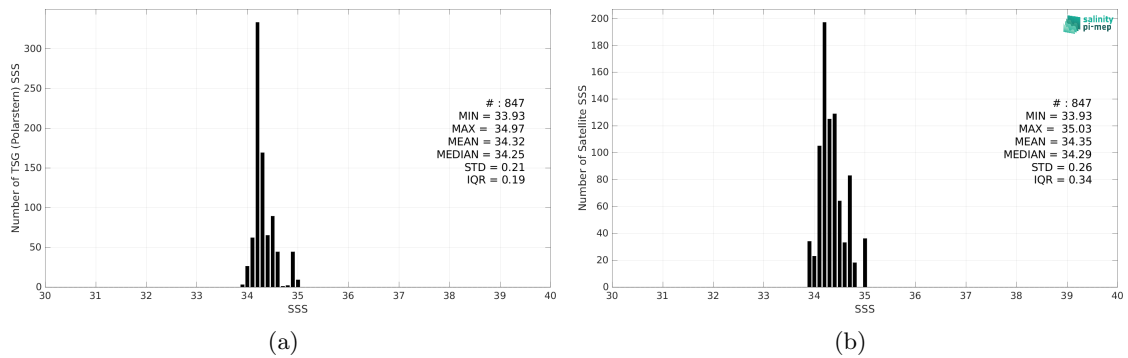
Figure 2: Histograms of SSS from TSG (Polarstern) (a) and SMOS SSS L3 v8 - 18 Days (CATDS-CEC-LOCEAN) (b) considering all match-up pairs per bins of 0.1 over the Pacific Ocean Pi-MEP region and for the full satellite product period.
