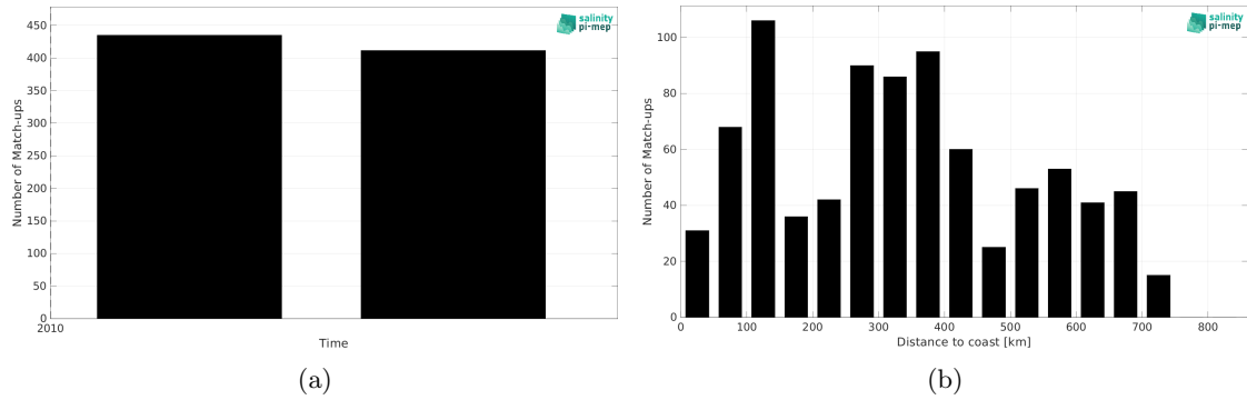
Figure 1: Number of match-ups between TSG (Polarstern) and SMOS SSS L3 v8 - 18 Days (CATDS-CEC-LOCEAN) SSS as a function of time (a) and as function of the distance to coast (b) over the Pacific Ocean Pi-MEP region and for the full satellite product period.
