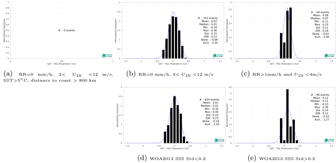
Figure 13: Normalized histogram of \Delta SSS (SMOS SSS L3 v8 - 18 Days (CATDS-CEC-LOCEAN) - TSG (Polarstern)) for 5 different subdatasets corresponding to: RR=0 mm/h, 3 < U_{10} < 12 m/s, SST > 5°C, distance to coast > 800 km (a), RR=0 mm/h, 3 < U_{10} < 12 m/s (b), RR > 1mm/h and U_{10} < 4 m/s (c), WOA2013 SSS Std < 0.2 (d), WOA2013 SSS Std > 0.2 (e).
