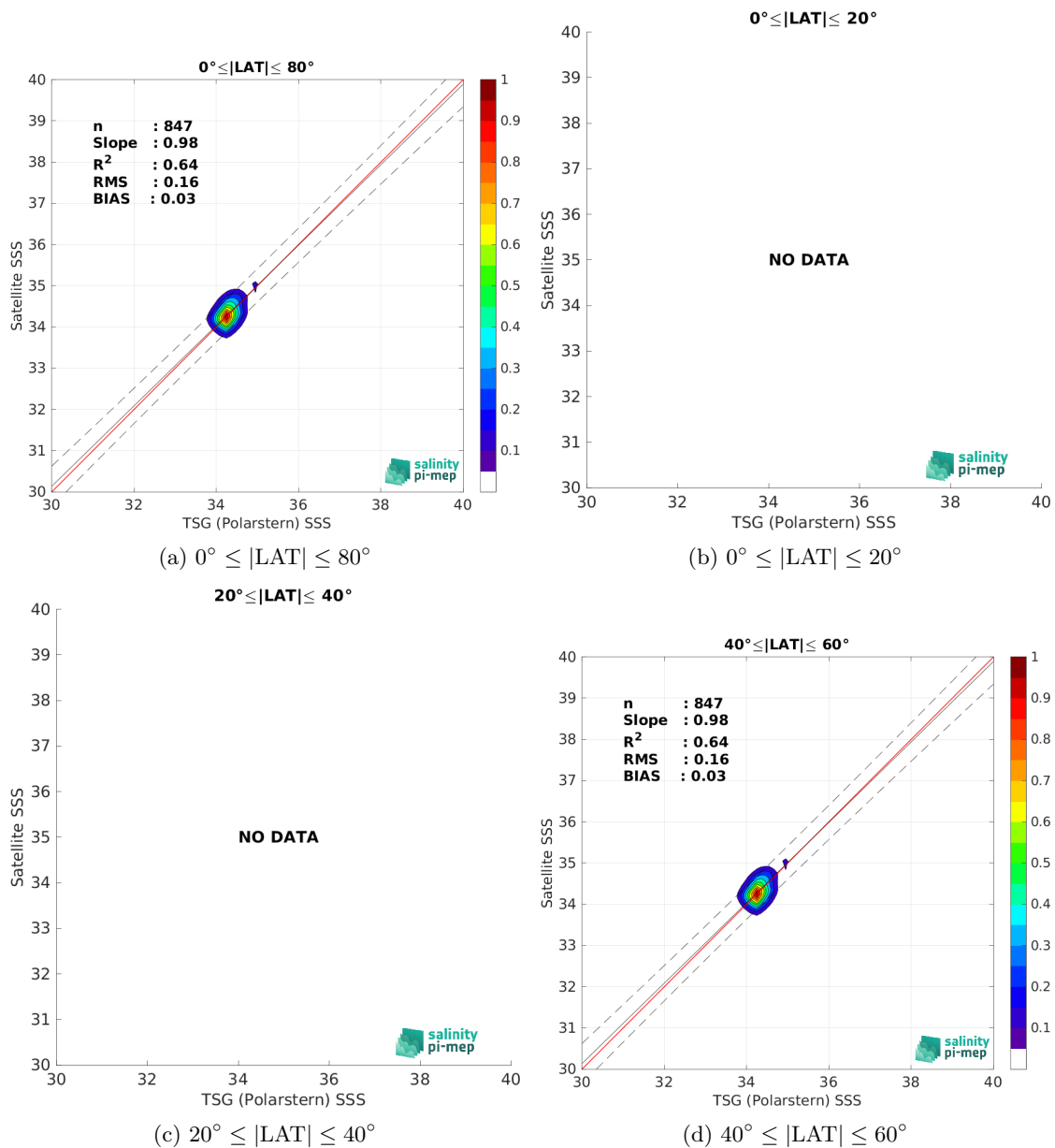
Figure 9: Contour maps of the concentration of SMOS SSS L3 v8 - 18 Days (CATDS-CEC-LOCEAN) SSS (y-axis) versus TSG (Polarstern) SSS (x-axis) at match-up pairs for different latitude bands. For each plot, the red line shows x=y . The black thin and dashed lines indicate a linear fit through the data cloud and the \pm 95\% confidence levels, respectively. The number match-up pairs n , the slope and R^2 coefficient of the linear fit, the root mean square (RMS) and the mean bias between satellite and in situ data are indicated for each latitude band in each plots.
