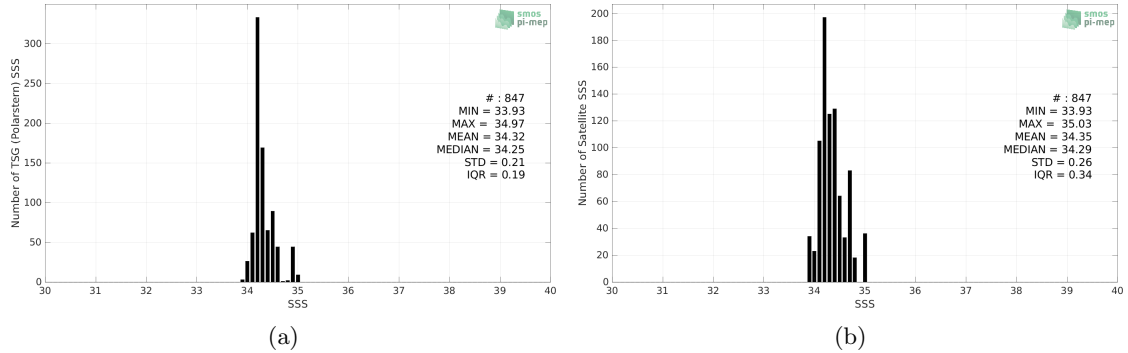
Figure 2: Histograms of SSS from TSG (Polarstern) (a) and SMOS SSS L3 v8 - 18 Days (CATDS-CECOS-LOCEAN) (b) considering all match-up pairs per bins of 0.1 over the Pacific Ocean Pi-MEP region and for the full satellite product period.
