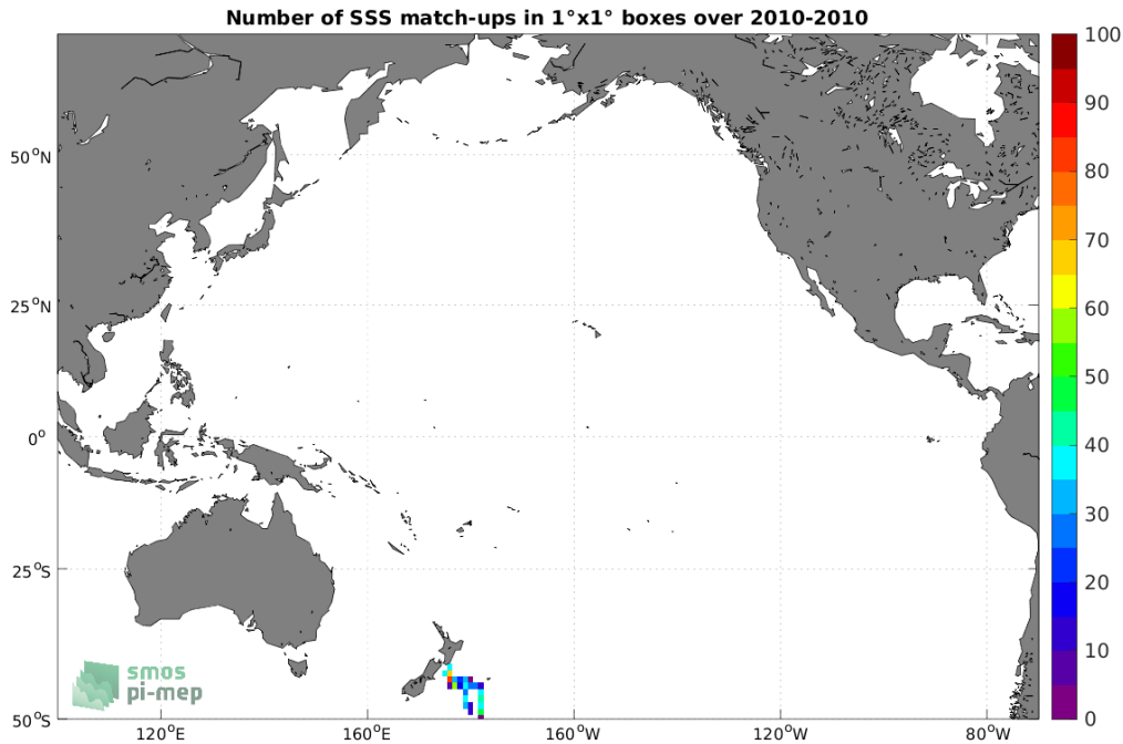
Figure 4: Number of SSS match-ups between TSG (Polarstern) SSS and the SMOS SSS L3 v8 - 18 Days (CATDS-CECOS-LOCEAN) SSS product for the Pacific Ocean Pi-MEP region over 1^\circ \times 1^\circ boxes and for the full satellite product period.
