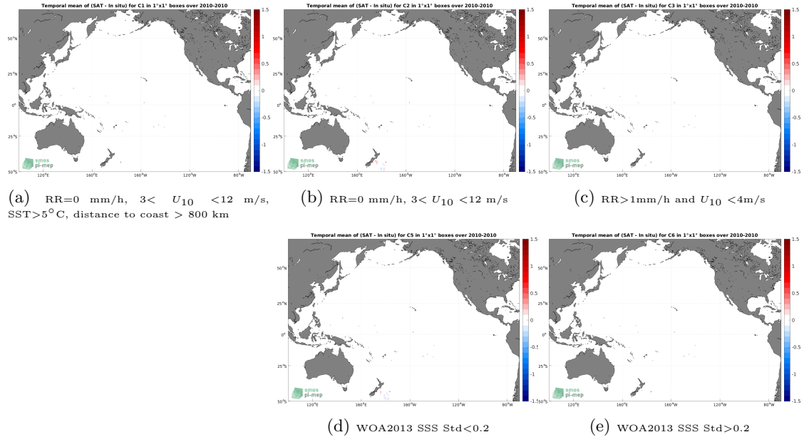
Figure 12: Temporal mean gridded over spatial boxes of size 1^{\circ}\times 1^{\circ} of \Delta\text{SSS} (SMOS SSS L3 v8 - 18 Days (CATDS-CECOS-LOCEAN) - TSG (Polarstern)) for 5 different subdatasets corresponding to:RR=0 mm/h, 3 < U_{10} < 12 m/s, SST >5^{\circ}\text{C} , distance to coast > 800 km (a), RR=0 mm/h, 3 < U_{10} < 12 m/s (b), RR >1 mm/h and U_{10} < 4 m/s (c), WOA2013 SSS Std <0.2 (d), WOA2013 SSS Std >0.2 (e).
