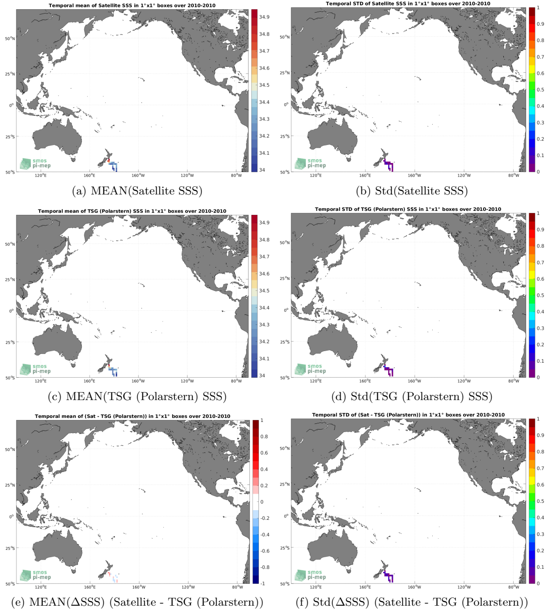
Figure 6: Temporal mean (left) and Std (right) of SSS from SMOS SSS L3 v8 - 18 Days (CATDS-CECOS-LOCEAN) (top), TSG (Polarstern) (middle), and of \Delta SSS (Satellite - TSG (Polarstern)). Only match-up pairs are used to generate these maps.
