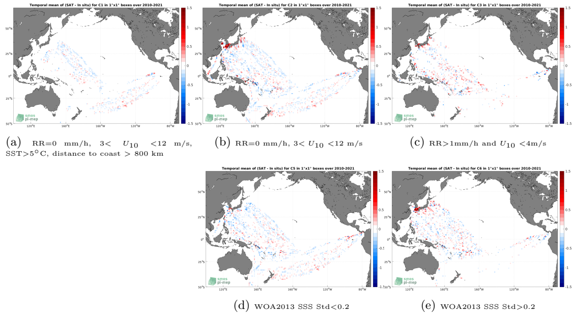
Figure 12: Temporal mean gridded over spatial boxes of size 1^\circ \times 1^\circ of \Delta SSS (SMOS SSS L3 v8 - 18 Days (CATDS-CECOS-LOCEAN) - TSG (LEGOS-DM)) for 5 different subdatasets corresponding to:RR=0 mm/h, 3 < U_{10} < 12 m/s, SST >5^\circ C, distance to coast > 800 km (a), RR=0 mm/h, 3 < U_{10} < 12 m/s (b), RR >1 mm/h and U_{10} < 4 m/s (c), WOA2013 SSS Std <0.2 (d), WOA2013 SSS Std >0.2 (e).
