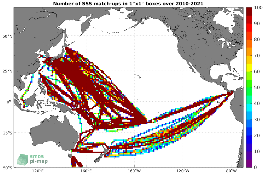
Figure 4: Number of SSS match-ups between TSG (LEGOS-DM) SSS and the SMOS SSS L3 v8 - 18 Days (CATDS-CECOS-LOCEAN) SSS product for the Pacific Ocean Pi-MEP region over 1^\circ \times 1^\circ boxes and for the full satellite product period.
