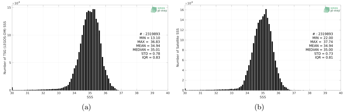
Figure 2: Histograms of SSS from TSG (LEGOS-DM) (a) and SMOS SSS L3 v8 - 18 Days (CATDS-CECOS-LOCEAN) (b) considering all match-up pairs per bins of 0.1 over the Pacific Ocean Pi-MEP region and for the full satellite product period.
