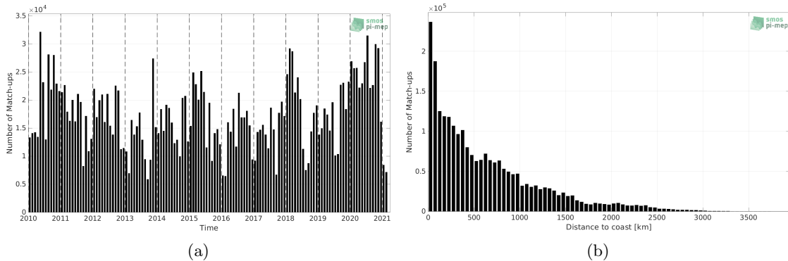
Figure 1: Number of match-ups between TSG (LEGOS-DM) and SMOS SSS L3 v8 - 18 Days (CATDS-CECOS-LOCEAN) SSS as a function of time (a) and as function of the distance to coast (b) over the Pacific Ocean Pi-MEP region and for the full satellite product period.
