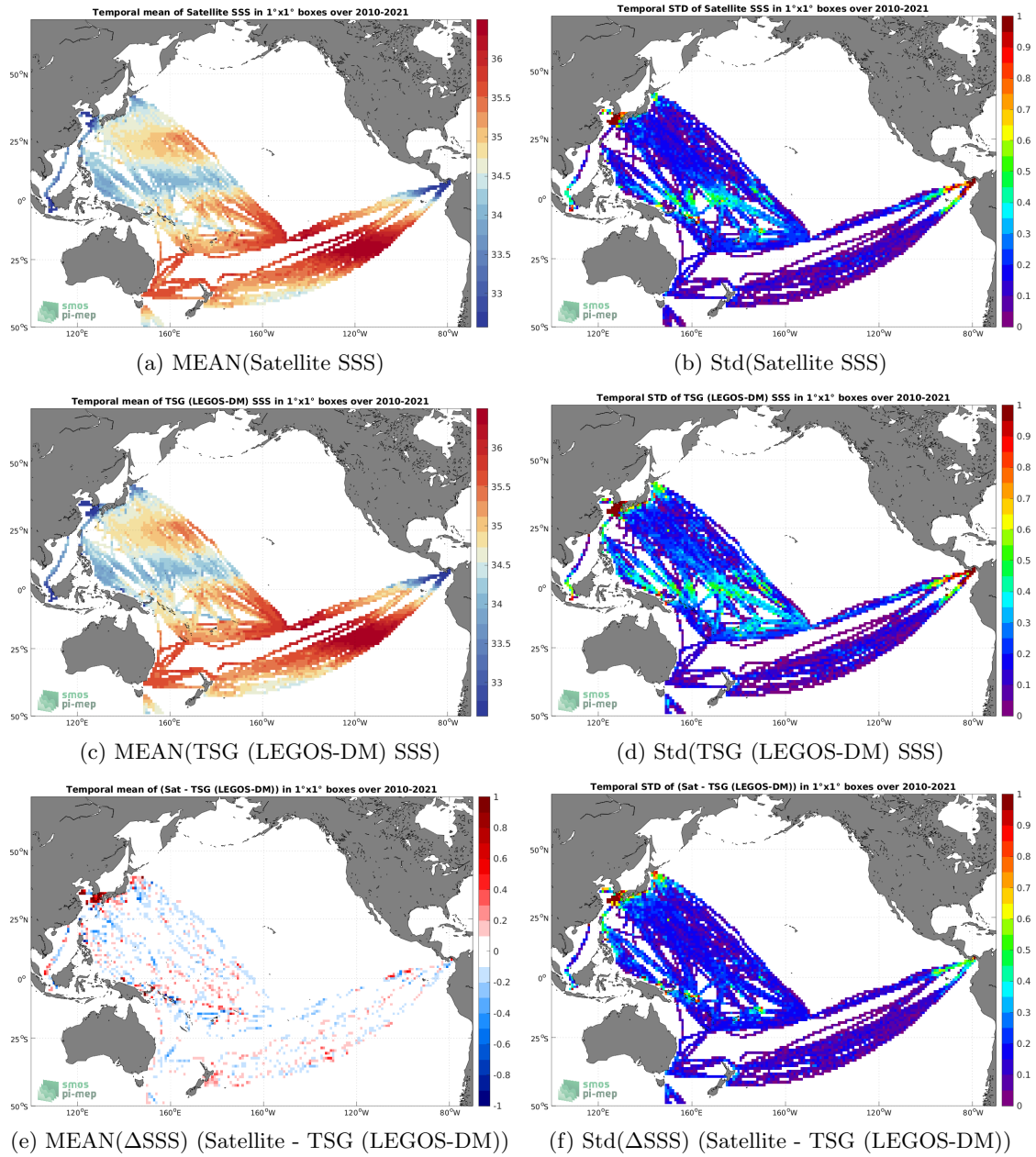
Figure 6: Temporal mean (left) and Std (right) of SSS from SMOS SSS L3 v8 - 18 Days (CATDS-CECOS-LOCEAN) (top), TSG (LEGOS-DM) (middle), and of \Delta SSS (Satellite - TSG (LEGOS-DM)). Only match-up pairs are used to generate these maps.
