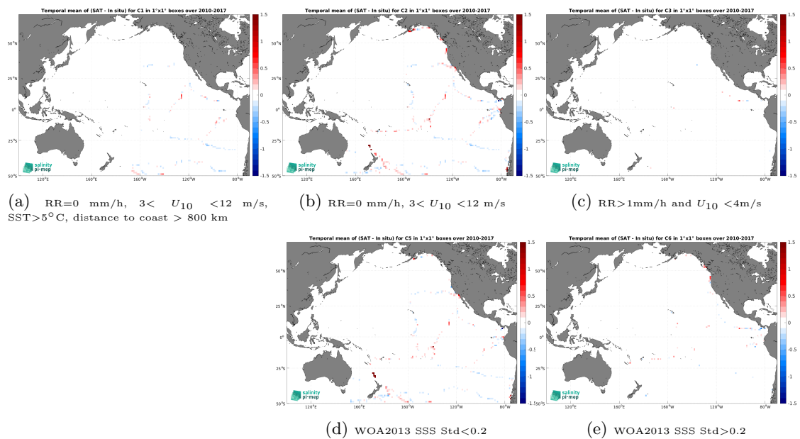
Figure 12: Temporal mean gridded over spatial boxes of size 1^\circ \times 1^\circ of \Delta SSS (SMOS SSS L3 v8 - 18 Days (CATDS-CEC-LOCEAN) - TSG (GOSUD-Sailing-ship)) for 5 different subdatasets corresponding to:RR=0 mm/h, 3 < U_{10} < 12 m/s, SST >5^\circ\text{C} , distance to coast > 800 km (a), RR=0 mm/h, 3 < U_{10} < 12 m/s (b), RR >1 mm/h and U_{10} < 4 m/s (c), WOA2013 SSS Std <0.2 (d), WOA2013 SSS Std >0.2 (e).
