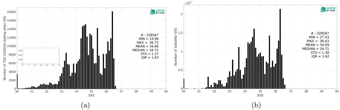
Figure 2: Histograms of SSS from TSG (GOSUD-Sailing-ship) (a) and SMOS SSS L3 v8 - 18 Days (CATDS-CEC-LOCEAN) (b) considering all match-up pairs per bins of 0.1 over the Pacific Ocean Pi-MEP region and for the full satellite product period.
