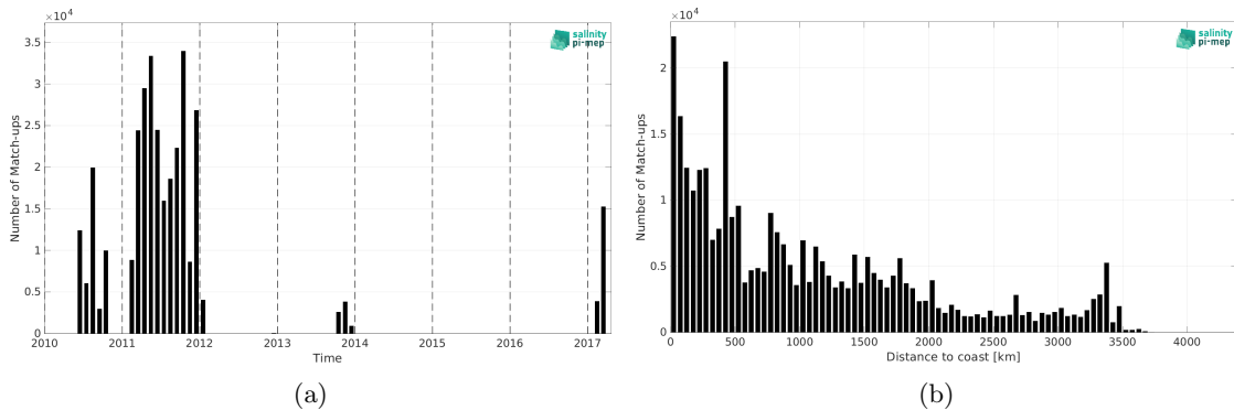
Figure 1: Number of match-ups between TSG (GOSUD-Sailing-ship) and SMOS SSS L3 v8 - 18 Days (CATDS-CEC-LOCEAN) SSS as a function of time (a) and as function of the distance to coast (b) over the Pacific Ocean Pi-MEP region and for the full satellite product period.
