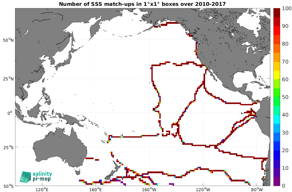
Figure 4: Number of SSS match-ups between TSG (GOSUD-Sailing-ship) SSS and the SMOS SSS L3 v8 - 18 Days (CATDS-CEC-LOCEAN) SSS product for the Pacific Ocean Pi-MEP region over 1^\circ \times 1^\circ boxes and for the full satellite product period.
