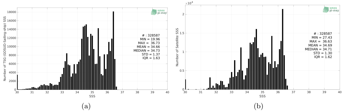
Figure 2: Histograms of SSS from TSG (GOSUD-Sailing-ship) (a) and SMOS SSS L3 v8 - 18 Days (CATDS-CECOS-LOCEAN) (b) considering all match-up pairs per bins of 0.1 over the Pacific Ocean Pi-MEP region and for the full satellite product period.
