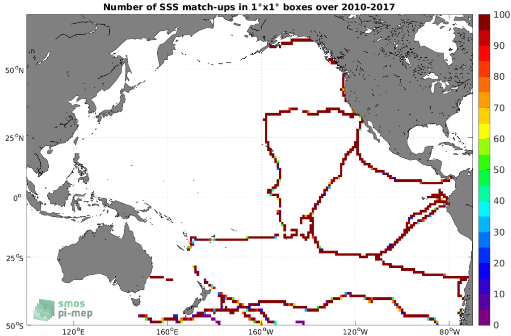
Figure 4: Number of SSS match-ups between TSG (GOSUD-Sailing-ship) SSS and the SMOS SSS L3 v8 - 18 Days (CATDS-CECOS-LOCEAN) SSS product for the Pacific Ocean Pi-MEP region over 1^\circ \times 1^\circ boxes and for the full satellite product period.
