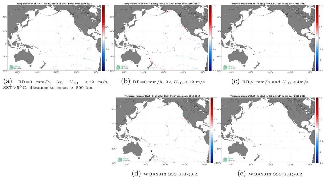
Figure 12: Temporal mean gridded over spatial boxes of size 1^\circ \times 1^\circ of \Delta SSS (SMOS SSS L3 v8 - 18 Days (CATDS-CECOS-LOCEAN) - TSG (GOSUD-Sailing-ship)) for 5 different subdatasets corresponding to:RR=0 mm/h, 3 < U_{10} < 12 m/s, SST>5°C, distance to coast > 800 km (a), RR=0 mm/h, 3 < U_{10} < 12 m/s (b), RR>1mm/h and U_{10} < 4 m/s (c), WOA2013 SSS Std<0.2 (d), WOA2013 SSS Std>0.2 (e).
