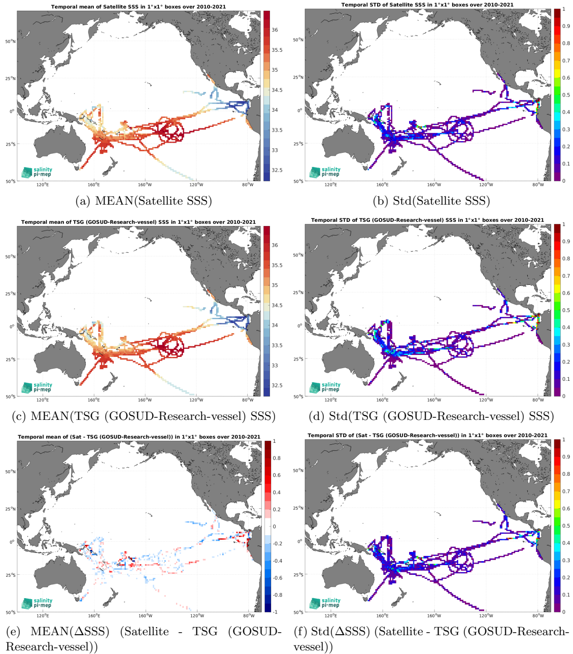
Figure 6: Temporal mean (left) and Std (right) of SSS from SMOS SSS L3 v8 - 18 Days (CATDS-CEC-LOCEAN) (top), TSG (GOSUD-Research-vessel) (middle), and of \Delta SSS (Satellite - TSG (GOSUD-Research-vessel)). Only match-up pairs are used to generate these maps.
