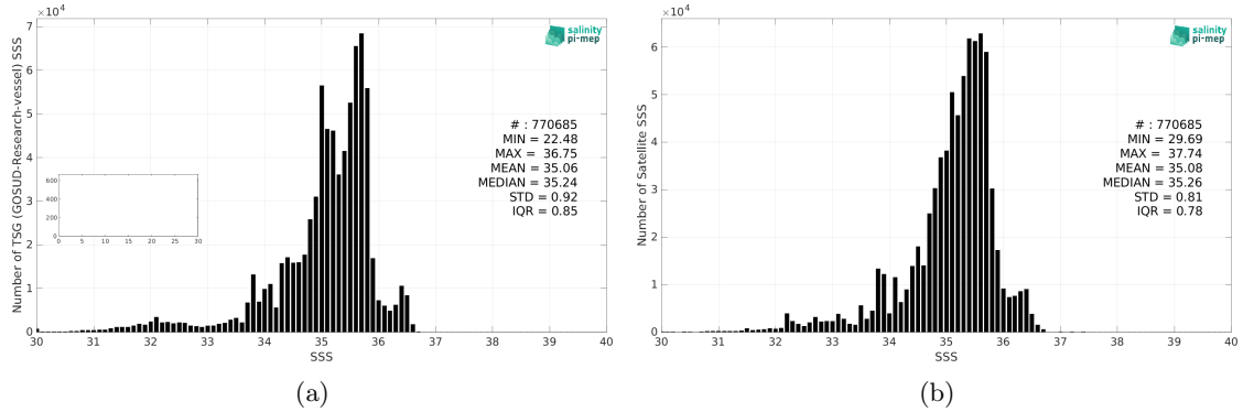
Figure 2: Histograms of SSS from TSG (GOSUD-Research-vessel) (a) and SMOS SSS L3 v8 - 18 Days (CATDS-CEC-LOCEAN) (b) considering all match-up pairs per bins of 0.1 over the Pacific Ocean Pi-MEP region and for the full satellite product period.
