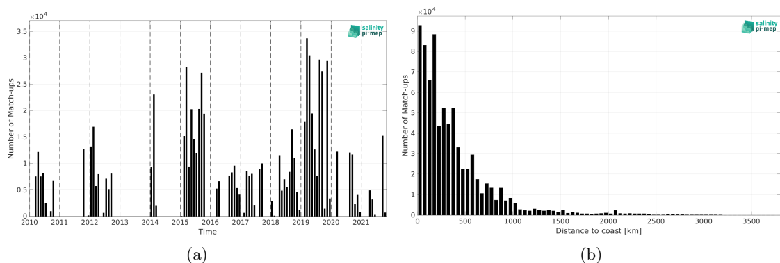
Figure 1: Number of match-ups between TSG (GOSUD-Research-vessel) and SMOS SSS L3 v8 - 18 Days (CATDS-CEC-LOCEAN) SSS as a function of time (a) and as function of the distance to coast (b) over the Pacific Ocean Pi-MEP region and for the full satellite product period.
