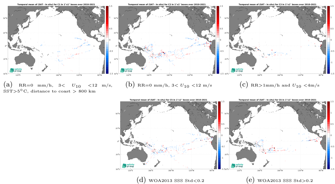
Figure 12: Temporal mean gridded over spatial boxes of size 1^\circ \times 1^\circ of \Delta SSS (SMOS SSS L3 v8 - 18 Days (CATDS-CEC-LOCEAN) - TSG (GOSUD-Research-vessel)) for 5 different subdatasets corresponding to:RR=0 mm/h, 3 < U_{10} < 12 m/s, SST >5^\circ\text{C} , distance to coast > 800 km (a), RR=0 mm/h, 3 < U_{10} < 12 m/s (b), RR >1 mm/h and U_{10} < 4 m/s (c), WOA2013 SSS Std <0.2 (d), WOA2013 SSS Std >0.2 (e).
