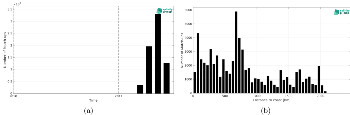
Figure 1: Number of match-ups between TSG (CSIC-UTM) and SMOS SSS L3 v8 - 18 Days (CATDS-CEC-LOCEAN) SSS as a function of time (a) and as function of the distance to coast (b) over the Pacific Ocean Pi-MEP region and for the full satellite product period.
