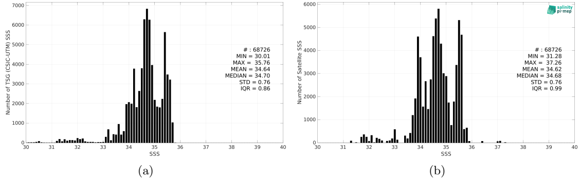
Figure 2: Histograms of SSS from TSG (CSIC-UTM) (a) and SMOS SSS L3 v8 - 18 Days (CATDS-CEC-LOCEAN) (b) considering all match-up pairs per bins of 0.1 over the Pacific Ocean Pi-MEP region and for the full satellite product period.
