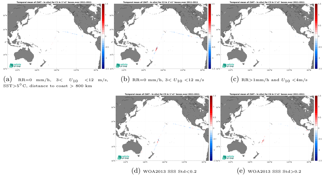
Figure 12: Temporal mean gridded over spatial boxes of size 1^{\circ}\times 1^{\circ} of \Delta\text{SSS} (SMOS SSS L3 v8 - 18 Days (CATDS-CEC-LOCEAN) - TSG (CSIC-UTM)) for 5 different subdatasets corresponding to: RR=0 mm/h, 3 < U_{10} < 12 m/s, SST > 5^{\circ}\text{C} , distance to coast > 800 km (a), RR=0 mm/h, 3 < U_{10} < 12 m/s (b), RR > 1 mm/h and U_{10} < 4 m/s (c), WOA2013 SSS Std < 0.2 (d), WOA2013 SSS Std > 0.2 (e).
