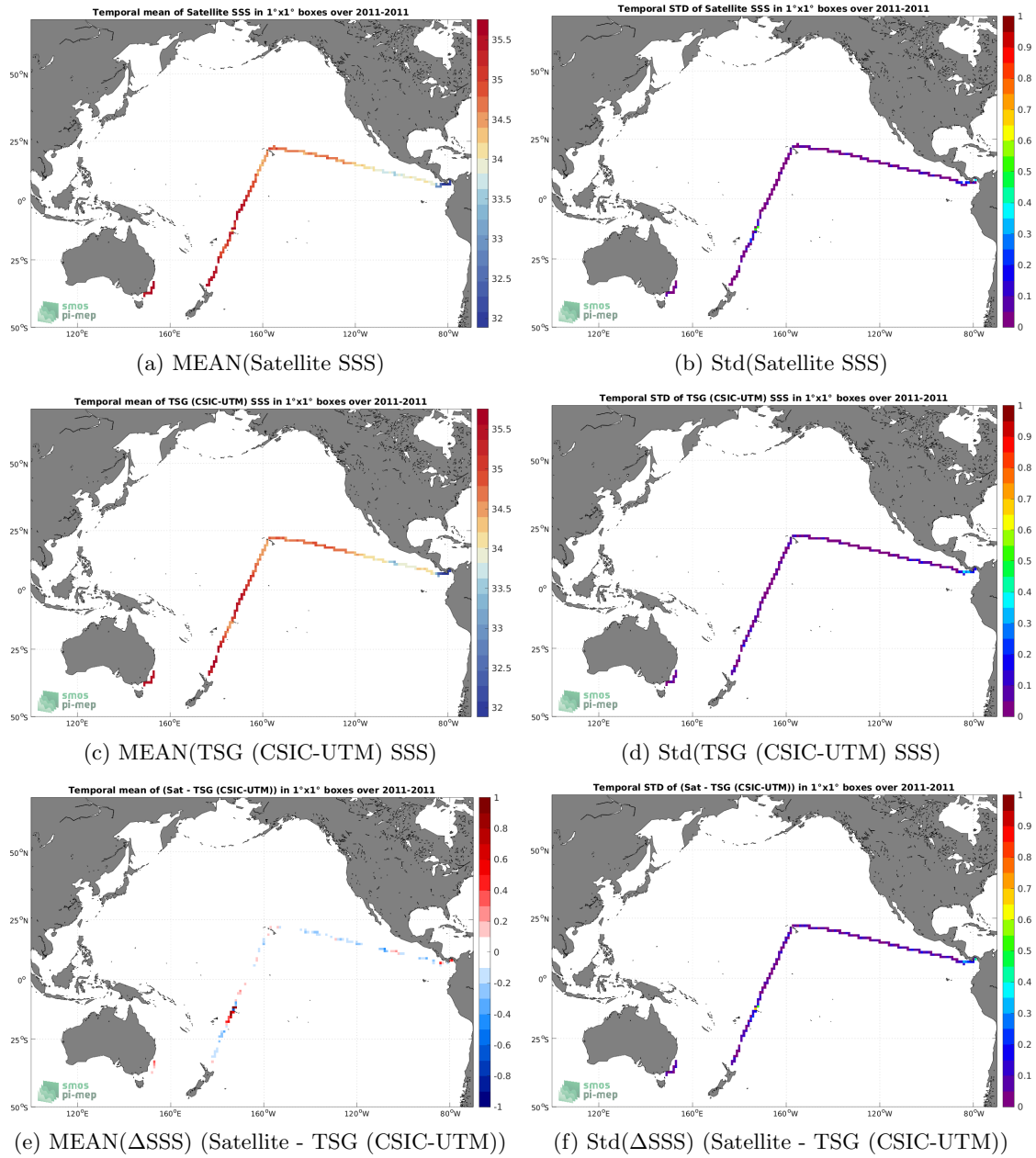
Figure 6: Temporal mean (left) and Std (right) of SSS from SMOS SSS L3 v8 - 18 Days (CATDS-CECOS-LOCEAN) (top), TSG (CSIC-UTM) (middle), and of \Delta SSS (Satellite - TSG (CSIC-UTM)). Only match-up pairs are used to generate these maps.
