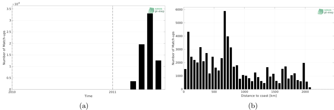
Figure 1: Number of match-ups between TSG (CSIC-UTM) and SMOS SSS L3 v8 - 18 Days (CATDS-CECOS-LOCEAN) SSS as a function of time (a) and as function of the distance to coast (b) over the Pacific Ocean Pi-MEP region and for the full satellite product period.
