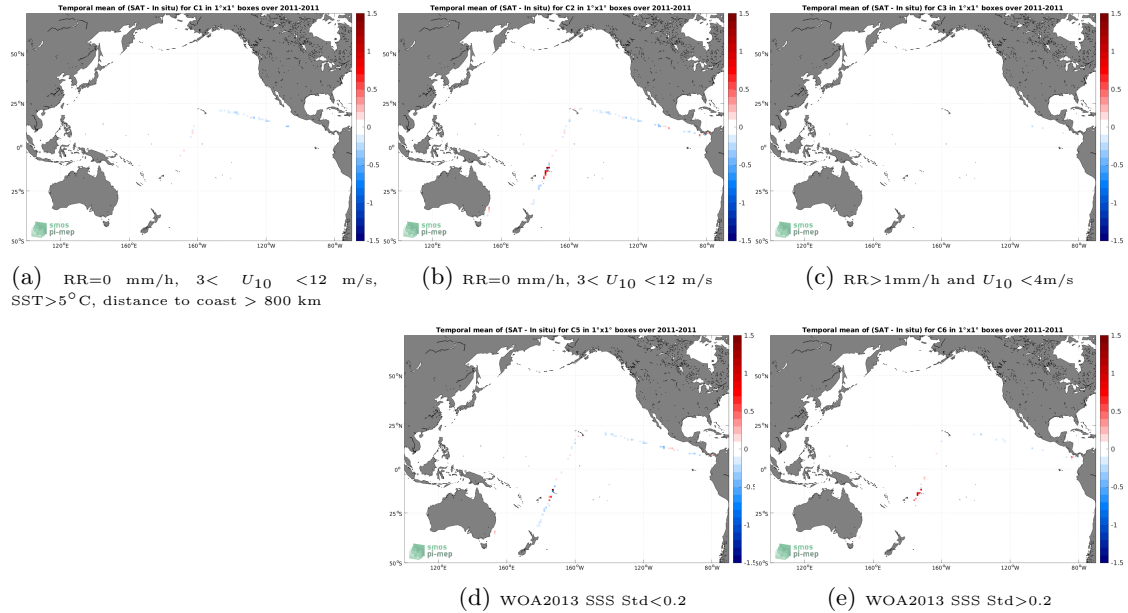
Figure 12: Temporal mean gridded over spatial boxes of size 1^{\circ}\times 1^{\circ} of \Delta\text{SSS} (SMOS SSS L3 v8 - 18 Days (CATDS-CECOS-LOCEAN) - TSG (CSIC-UTM)) for 5 different subdatasets corresponding to:RR=0 mm/h, 3 < U_{10} < 12 m/s, SST >5^{\circ}\text{C} , distance to coast > 800 km (a), RR=0 mm/h, 3 < U_{10} < 12 m/s (b), RR >1 mm/h and U_{10} < 4 m/s (c), WOA2013 SSS Std <0.2 (d), WOA2013 SSS Std >0.2 (e).
