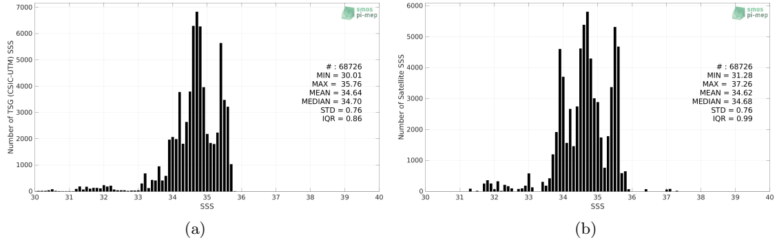
Figure 2: Histograms of SSS from TSG (CSIC-UTM) (a) and SMOS SSS L3 v8 - 18 Days (CATDS-CECOS-LOCEAN) (b) considering all match-up pairs per bins of 0.1 over the Pacific Ocean Pi-MEP region and for the full satellite product period.
