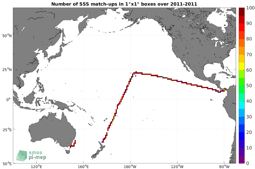
Figure 4: Number of SSS match-ups between TSG (CSIC-UTM) SSS and the SMOS SSS L3 v8 - 18 Days (CATDS-CECOS-LOCEAN) SSS product for the Pacific Ocean Pi-MEP region over 1^\circ \times 1^\circ boxes and for the full satellite product period.
