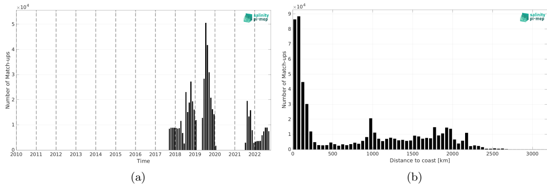
Figure 1: Number of match-ups between Saildrone and SMOS SSS L3 v8 - 18 Days (CATDS-CEC-LOCEAN) SSS as a function of time (a) and as function of the distance to coast (b) over the Pacific Ocean Pi-MEP region and for the full satellite product period.
