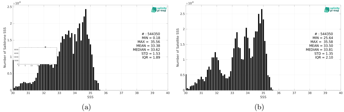
Figure 2: Histograms of SSS from Saildrone (a) and SMOS SSS L3 v8 - 18 Days (CATDS-CEC-LOCEAN) (b) considering all match-up pairs per bins of 0.1 over the Pacific Ocean Pi-MEP region and for the full satellite product period.
