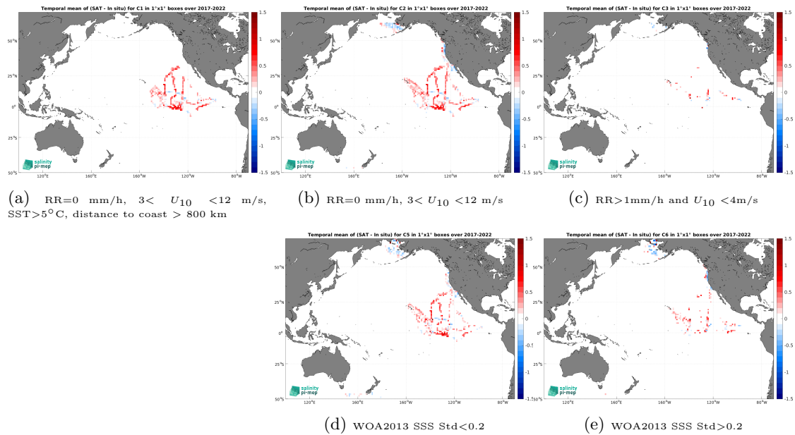
Figure 12: Temporal mean gridded over spatial boxes of size 1^\circ \times 1^\circ of \Delta SSS (SMOS SSS L3 v8 - 18 Days (CATDS-CEC-LOCEAN) - Saildrone) for 5 different subdatasets corresponding to:RR=0 mm/h, 3 < U_{10} < 12 m/s, SST >5^\circ C, distance to coast > 800 km (a), RR=0 mm/h, 3 < U_{10} < 12 m/s (b), RR >1 mm/h and U_{10} < 4 m/s (c), WOA2013 SSS Std <0.2 (d), WOA2013 SSS Std >0.2 (e).
