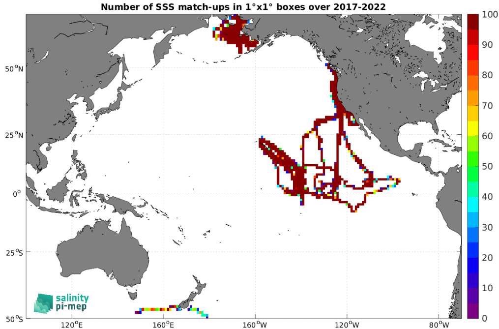
Figure 4: Number of SSS match-ups between Saildrone SSS and the SMOS SSS L3 v8 - 18 Days (CATDS-CEC-LOCEAN) SSS product for the Pacific Ocean Pi-MEP region over 1^\circ \times 1^\circ boxes and for the full satellite product period.
