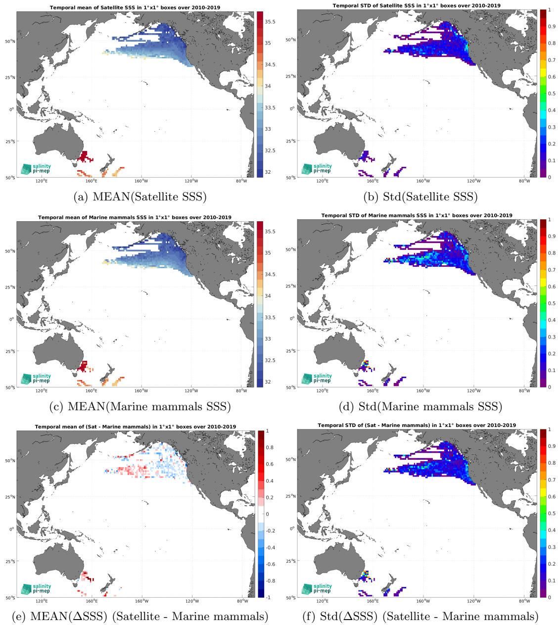
Figure 6: Temporal mean (left) and Std (right) of SSS from SMOS SSS L3 v8 - 18 Days (CATDS-CEC-LOCEAN) (top), Marine mammals (middle), and of \Delta SSS (Satellite - Marine mammals). Only match-up pairs are used to generate these maps.
