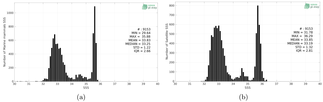
Figure 2: Histograms of SSS from Marine mammals (a) and SMOS SSS L3 v8 - 18 Days (CATDS-CECOS-LOCEAN) (b) considering all match-up pairs per bins of 0.1 over the Pacific Ocean Pi-MEP region and for the full satellite product period.
