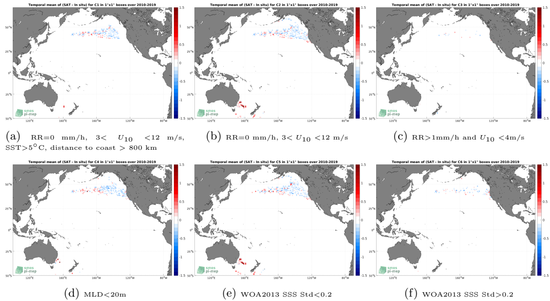
Figure 12: Temporal mean gridded over spatial boxes of size 1^{\circ}\times 1^{\circ} of \Delta\text{SSS} (SMOS SSS L3 v8 - 18 Days (CATDS-CECOS-LOCEAN) - Marine mammals) for 6 different subdatasets corresponding to:RR=0 mm/h, 3 < U_{10} < 12 m/s, SST > 5^{\circ}\text{C} , distance to coast > 800 km (a), RR=0 mm/h, 3 < U_{10} < 12 m/s (b), RR > 1\text{mm/h} and U_{10} < 4\text{m/s} (c),MLD < 20\text{m} (d),WOA2013 SSS Std < 0.2 (e),WOA2013 SSS Std > 0.2 (f).
