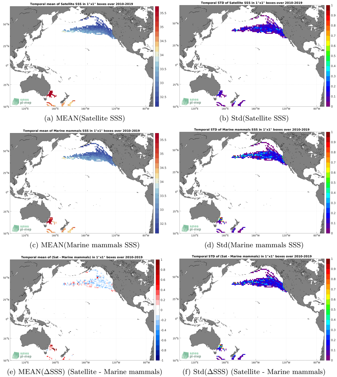
Figure 6: Temporal mean (left) and Std (right) of SSS from SMOS SSS L3 v8 - 18 Days (CATDS-CECOS-LOCEAN) (top), Marine mammals (middle), and of \Delta SSS (Satellite - Marine mammals). Only match-up pairs are used to generate these maps.
