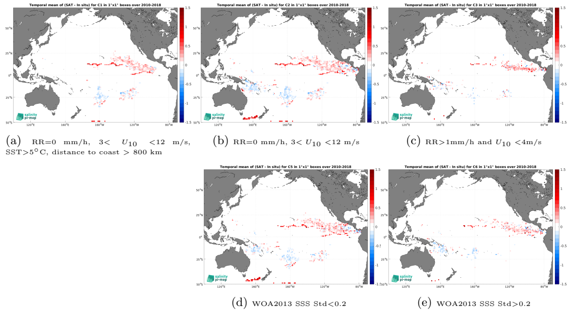
Figure 11: Temporal mean gridded over spatial boxes of size 1^\circ \times 1^\circ of \Delta SSS (SMOS SSS L3 v8 - 18 Days (CATDS-CEC-LOCEAN) - Surface drifters) for 5 different subdatasets corresponding to:RR=0 mm/h, 3 < U_{10} < 12 m/s, SST >5^\circ C, distance to coast > 800 km (a), RR=0 mm/h, 3 < U_{10} < 12 m/s (b), RR >1 mm/h and U_{10} < 4 m/s (c), WOA2013 SSS Std <0.2 (d), WOA2013 SSS Std >0.2 (e).
