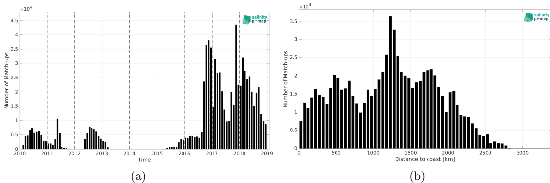
Figure 1: Number of match-ups between Surface drifters and SMOS SSS L3 v8 - 18 Days (CATDS-CEC-LOCEAN) SSS as a function of time (a) and as function of the distance to coast (b) over the Pacific Ocean Pi-MEP region and for the full satellite product period.
