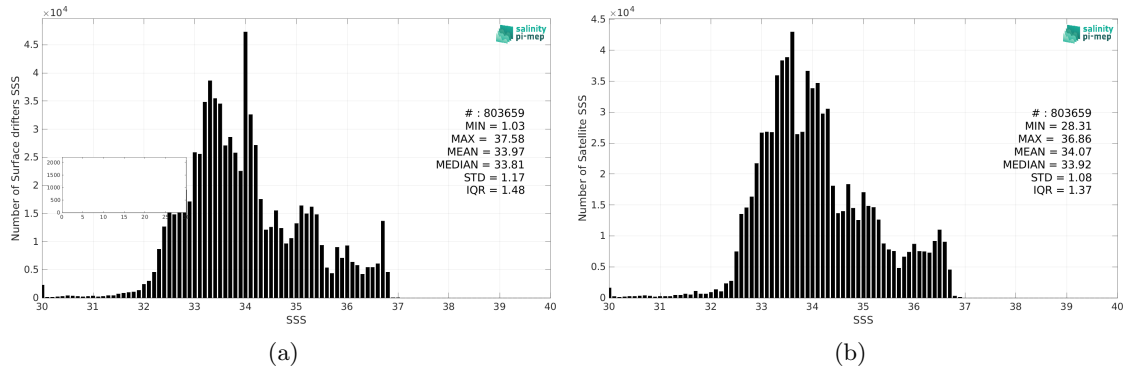
Figure 2: Histograms of SSS from Surface drifters (a) and SMOS SSS L3 v8 - 18 Days (CATDS-CEC-LOCEAN) (b) considering all match-up pairs per bins of 0.1 over the Pacific Ocean Pi-MEP region and for the full satellite product period.
