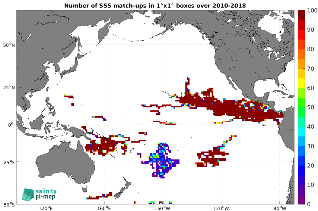
Figure 3: Number of SSS match-ups between Surface drifters SSS and the SMOS SSS L3 v8 - 18 Days (CATDS-CEC-LOCEAN) SSS product for the Pacific Ocean Pi-MEP region over 1^\circ \times 1^\circ boxes and for the full satellite product period.
