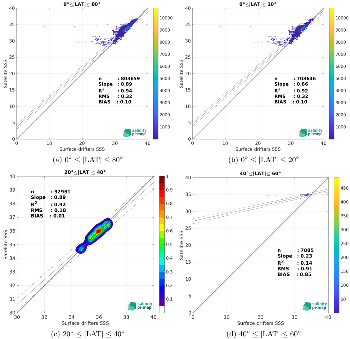
Figure 8: Contour maps of the concentration of SMOS SSS L3 v8 - 18 Days (CATDS-CEC-LOCEAN) SSS (y-axis) versus Surface drifters SSS (x-axis) at match-up pairs for different latitude bands. For each plot, the red line shows x=y . The black thin and dashed lines indicate a linear fit through the data cloud and the \pm 95\% confidence levels, respectively. The number match-up pairs n , the slope and R^2 coefficient of the linear fit, the root mean square (RMS) and the mean bias between satellite and in situ data are indicated for each latitude band in each plots.
