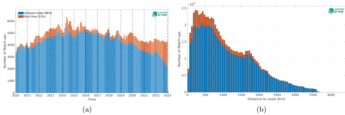
Figure 1: Number of match-ups between Argo and SMOS SSS L3 v8 - 18 Days (CATDS-CEC-LOCEAN) SSS as a function of time (a) and as function of the distance to coast (b) over the Pacific Ocean Pi-MEP region and for the full satellite product period.
