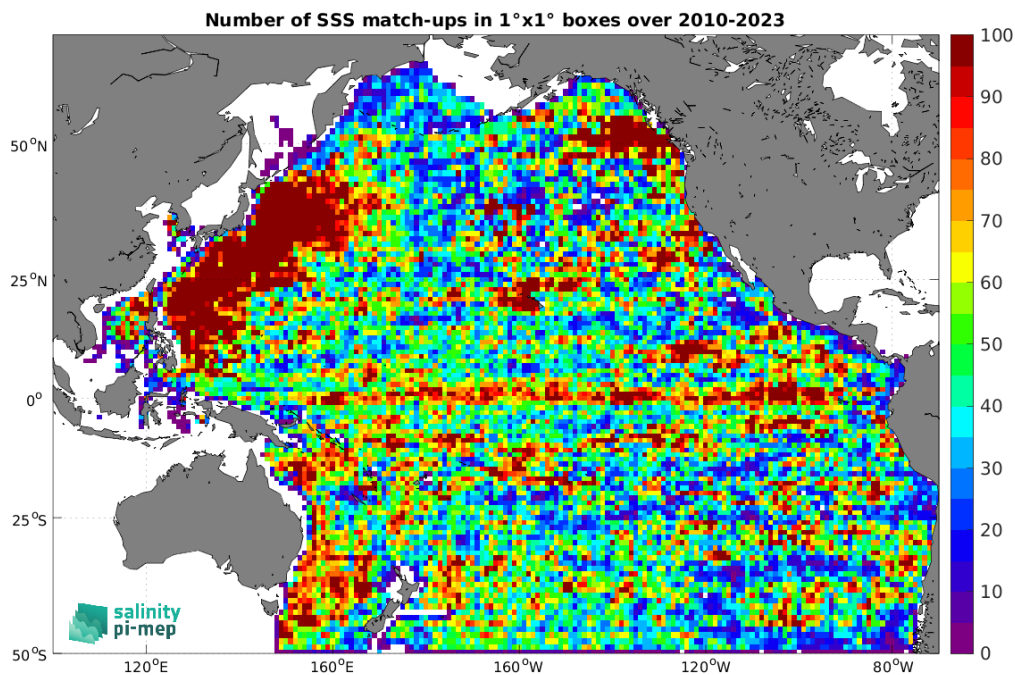
Figure 4: Number of SSS match-ups between Argo SSS and the SMOS SSS L3 v8 - 18 Days (CATDS-CEC-LOCEAN) SSS product for the Pacific Ocean Pi-MEP region over 1^\circ \times 1^\circ boxes and for the full satellite product period.
