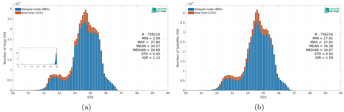
Figure 2: Histograms of SSS from Argo (a) and SMOS SSS L3 v8 - 18 Days (CATDS-CEC-LOCEAN) (b) considering all match-up pairs per bins of 0.1 over the Pacific Ocean Pi-MEP region and for the full satellite product period.
