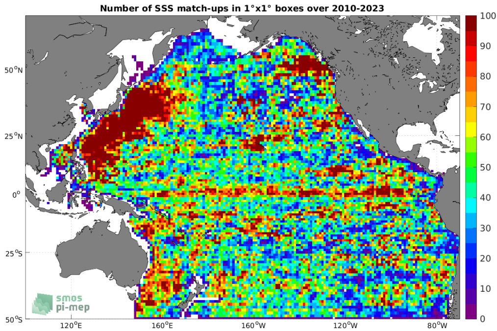
Figure 4: Number of SSS match-ups between Argo SSS and the SMOS SSS L3 v8 - 18 Days (CATDS-CECOS-LOCEAN) SSS product for the Pacific Ocean Pi-MEP region over 1^\circ \times 1^\circ boxes and for the full satellite product period.
