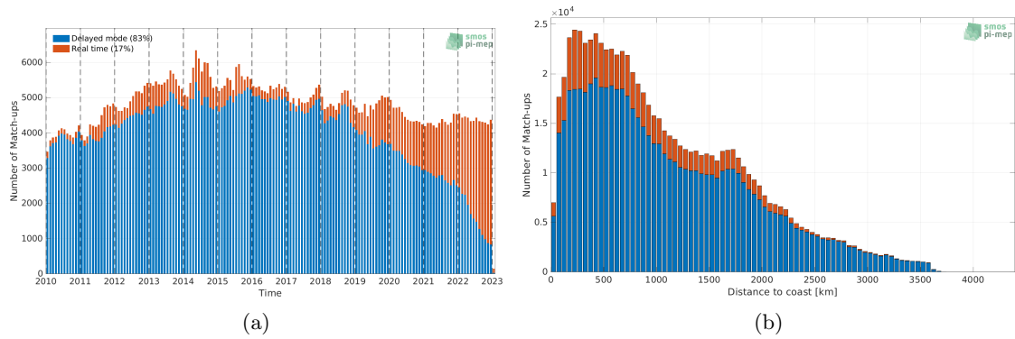
Figure 1: Number of match-ups between Argo and SMOS SSS L3 v8 - 18 Days (CATDS-CECOS-LOCEAN) SSS as a function of time (a) and as function of the distance to coast (b) over the Pacific Ocean Pi-MEP region and for the full satellite product period.
