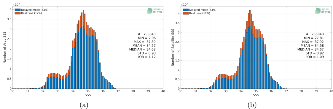
Figure 2: Histograms of SSS from Argo (a) and SMOS SSS L3 v8 - 18 Days (CATDS-CECOS-LOCEAN) (b) considering all match-up pairs per bins of 0.1 over the Pacific Ocean Pi-MEP region and for the full satellite product period.
