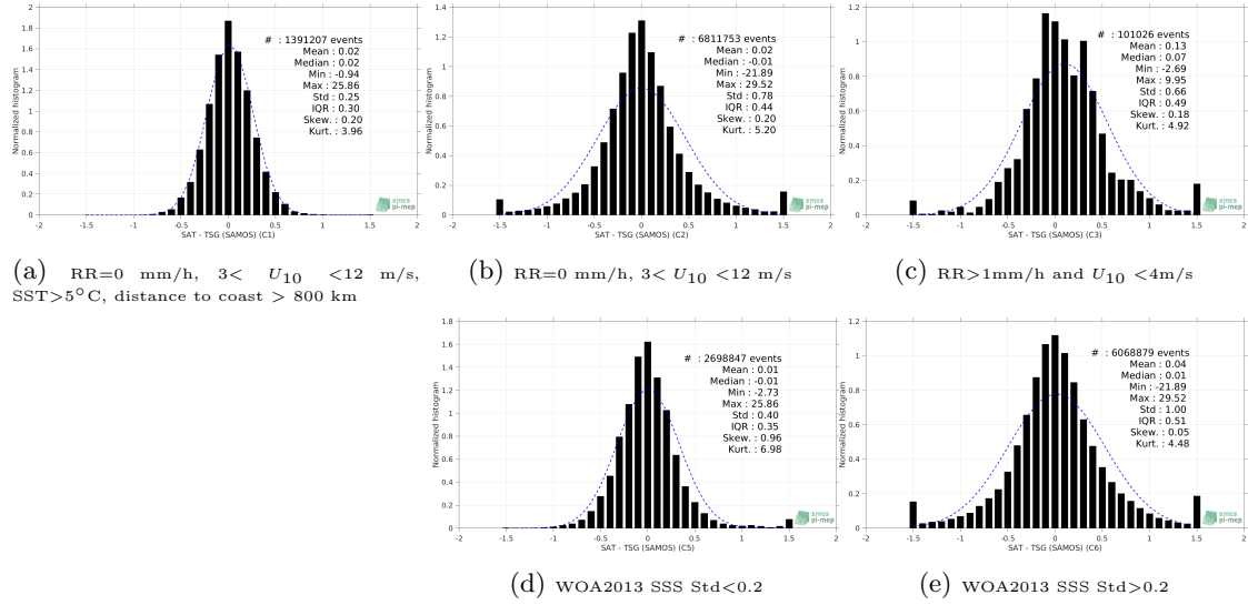
Figure 13: Normalized histogram of \Delta\text{SSS} (SMOS SSS L3 v7 - 9 Days (CATDS-CECOS-LOCEAN) - TSG (SAMOS)) for 5 different subdatasets corresponding to: RR=0 mm/h, 3 < U_{10} < 12 m/s, SST>5°C, distance to coast > 800 km (a), RR=0 mm/h, 3 < U_{10} < 12 m/s (b), RR>1mm/h and U_{10} < 4 m/s (c), WOA2013 SSS Std<0.2 (d), WOA2013 SSS Std>0.2 (e).
