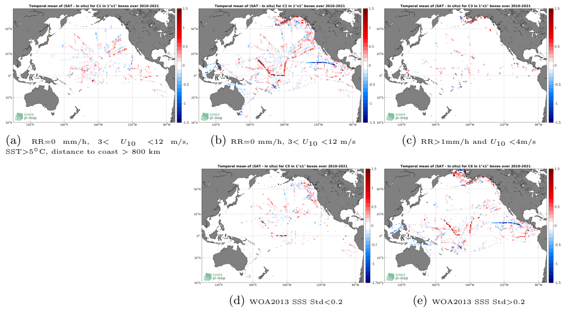
Figure 12: Temporal mean gridded over spatial boxes of size 1^\circ \times 1^\circ of \Delta SSS (SMOS SSS L3 v7 - 9 Days (CATDS-CECOS-LOCEAN) - TSG (SAMOS)) for 5 different subdatasets corresponding to:RR=0 mm/h, 3 < U_{10} < 12 m/s, SST > 5°C, distance to coast > 800 km (a), RR=0 mm/h, 3 < U_{10} < 12 m/s (b), RR > 1mm/h and U_{10} < 4 m/s (c), WOA2013 SSS Std < 0.2 (d), WOA2013 SSS Std > 0.2 (e).
