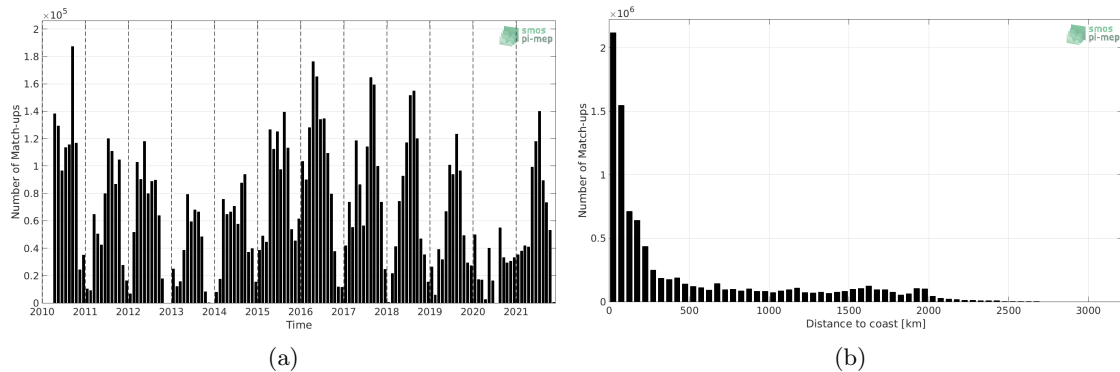
Figure 1: Number of match-ups between TSG (SAMOS) and SMOS SSS L3 v7 - 9 Days (CATDS-CECOS-LOCEAN) SSS as a function of time (a) and as function of the distance to coast (b) over the Pacific Ocean Pi-MEP region and for the full satellite product period.
