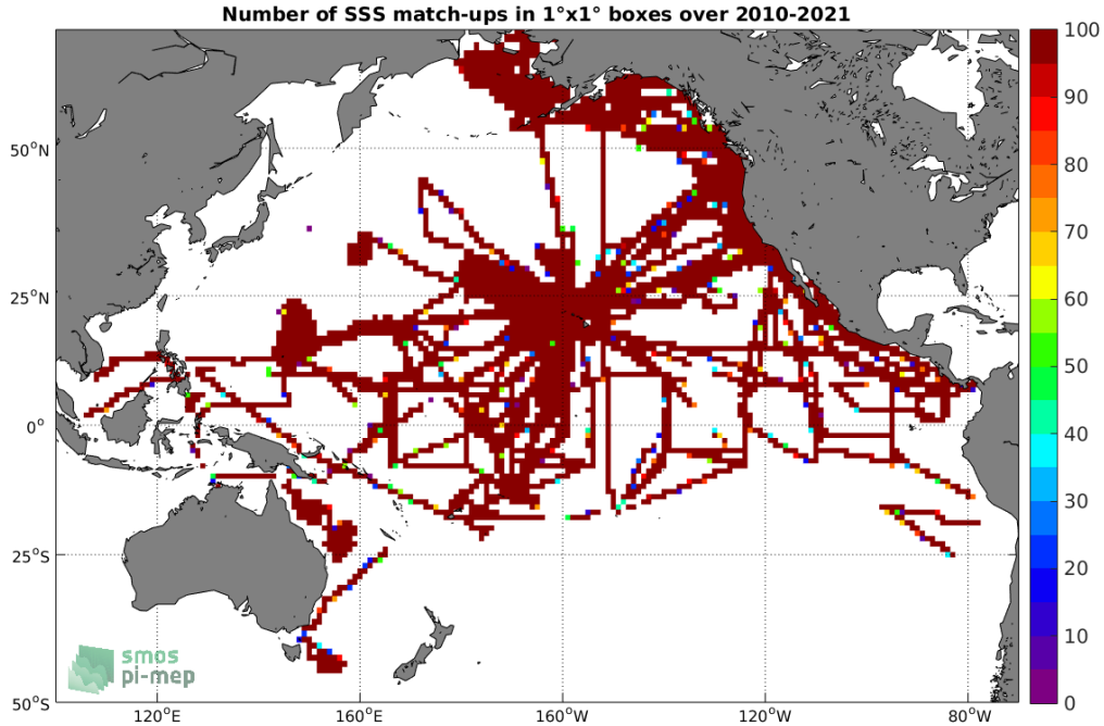
Figure 4: Number of SSS match-ups between TSG (SAMOS) SSS and the SMOS SSS L3 v7 - 9 Days (CATDS-CECOS-LOCEAN) SSS product for the Pacific Ocean Pi-MEP region over 1^\circ \times 1^\circ boxes and for the full satellite product period.
