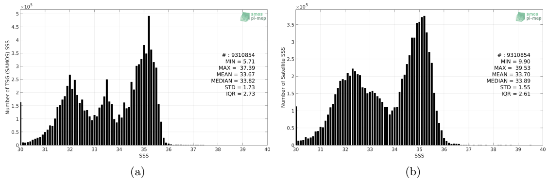
Figure 2: Histograms of SSS from TSG (SAMOS) (a) and SMOS SSS L3 v7 - 9 Days (CATDS-CECOS-LOCEAN) (b) considering all match-up pairs per bins of 0.1 over the Pacific Ocean Pi-MEP region and for the full satellite product period.
