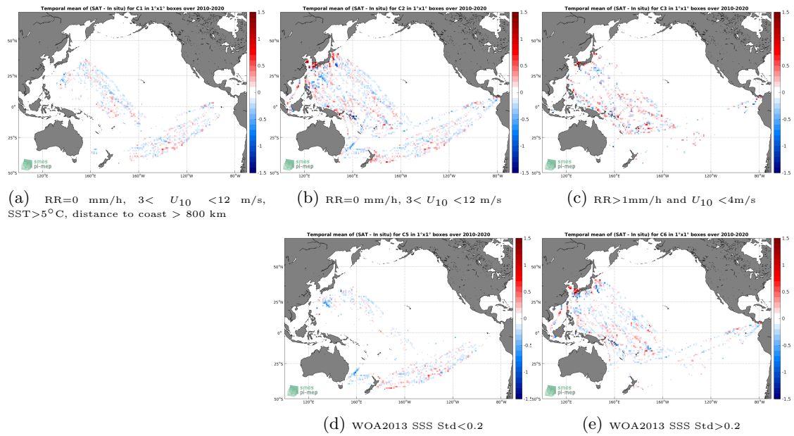
Figure 12: Temporal mean gridded over spatial boxes of size 1^\circ \times 1^\circ of \Delta\text{SSS} (SMOS SSS L3 v7 - 9 Days (CATDS-CECOS-LOCEAN) - TSG (LEGOS-DM)) for 5 different subdatasets corresponding to:RR=0 mm/h, 3 < U_{10} < 12 m/s, SST >5^\circ\text{C} , distance to coast > 800 km (a), RR=0 mm/h, 3 < U_{10} < 12 m/s (b), RR >1 mm/h and U_{10} < 4 m/s (c), WOA2013 SSS Std <0.2 (d), WOA2013 SSS Std >0.2 (e).
