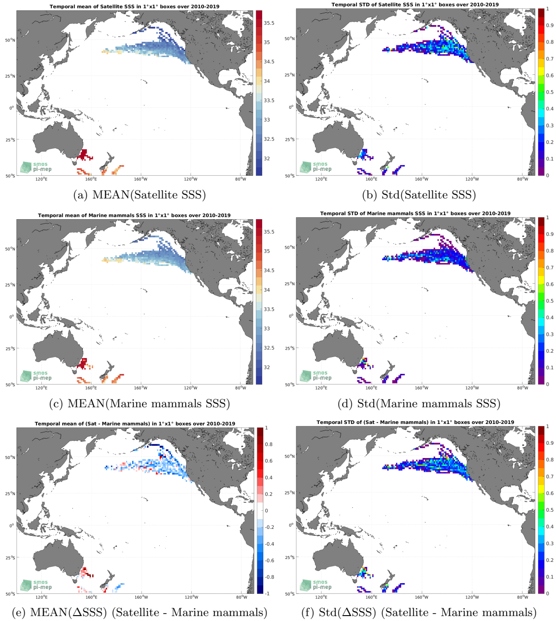
Figure 6: Temporal mean (left) and Std (right) of SSS from SMOS SSS L3 v7 - 9 Days (CATDS-CECOS-LOCEAN) (top), Marine mammals (middle), and of \Delta SSS (Satellite - Marine mammals). Only match-up pairs are used to generate these maps.
