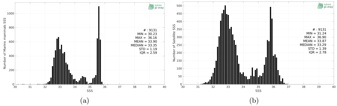
Figure 2: Histograms of SSS from Marine mammals (a) and SMOS SSS L3 v7 - 9 Days (CATDS-CECOS-LOCEAN) (b) considering all match-up pairs per bins of 0.1 over the Pacific Ocean Pi-MEP region and for the full satellite product period.
