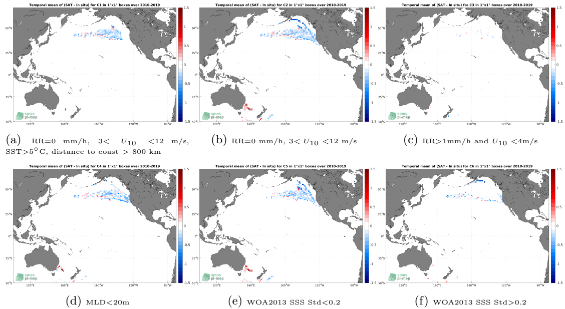
Figure 12: Temporal mean gridded over spatial boxes of size 1^{\circ}\times 1^{\circ} of \Delta\text{SSS} (SMOS SSS L3 v7 - 9 Days (CATDS-CECOS-LOCEAN) - Marine mammals) for 6 different subdatasets corresponding to: RR=0 mm/h, 3 < U_{10} < 12 m/s, SST > 5^{\circ}\text{C} , distance to coast > 800 km (a), RR=0 mm/h, 3 < U_{10} < 12 m/s (b), RR > 1\text{mm/h} and U_{10} < 4\text{m/s} (c), MLD < 20\text{m} (d), WOA2013 SSS Std < 0.2 (e), WOA2013 SSS Std > 0.2 (f).
