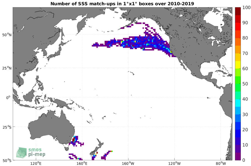
Figure 4: Number of SSS match-ups between Marine mammals SSS and the SMOS SSS L3 v7 - 9 Days (CATDS-CECOS-LOCEAN) SSS product for the Pacific Ocean Pi-MEP region over 1^\circ \times 1^\circ boxes and for the full satellite period.
