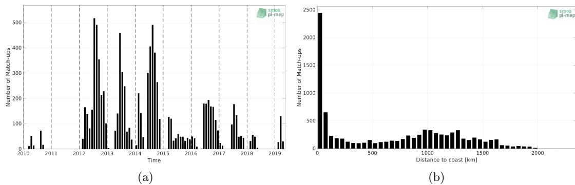
Figure 1: Number of match-ups between Marine mammals and SMOS SSS L3 v7 - 9 Days (CATDS-CECOS-LOCEAN) SSS as a function of time (a) and as function of the distance to coast (b) over the Pacific Ocean Pi-MEP region and for the full satellite product period.
