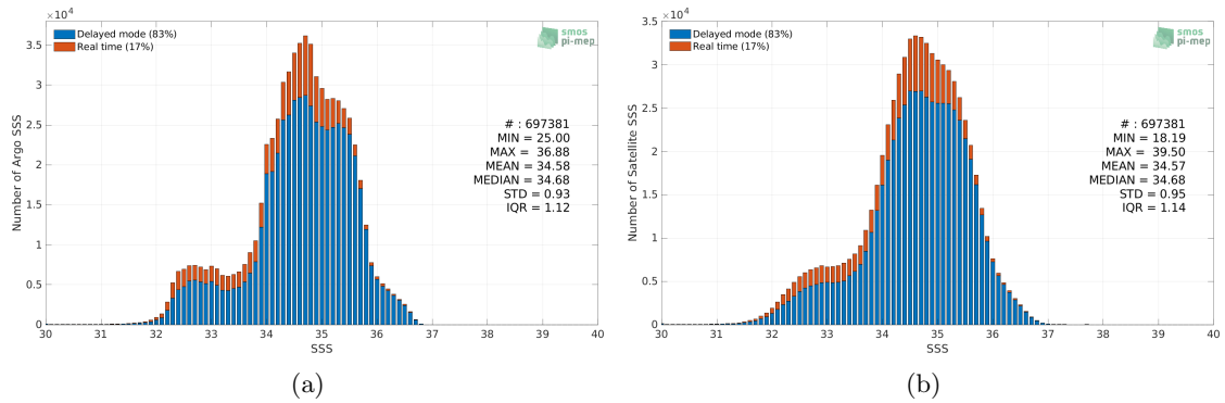
Figure 2: Histograms of SSS from Argo (a) and SMOS SSS L3 v7 - 9 Days (CATDS-CECOS-LOCEAN) (b) considering all match-up pairs per bins of 0.1 over the Pacific Ocean Pi-MEP region and for the full satellite product period.
