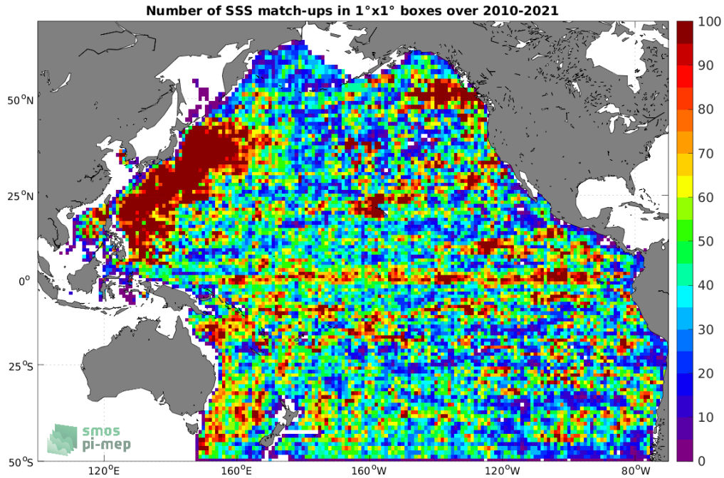
Figure 4: Number of SSS match-ups between Argo SSS and the SMOS SSS L3 v7 - 9 Days (CATDS-CECOS-LOCEAN) SSS product for the Pacific Ocean Pi-MEP region over 1^\circ \times 1^\circ boxes and for the full satellite product period.
