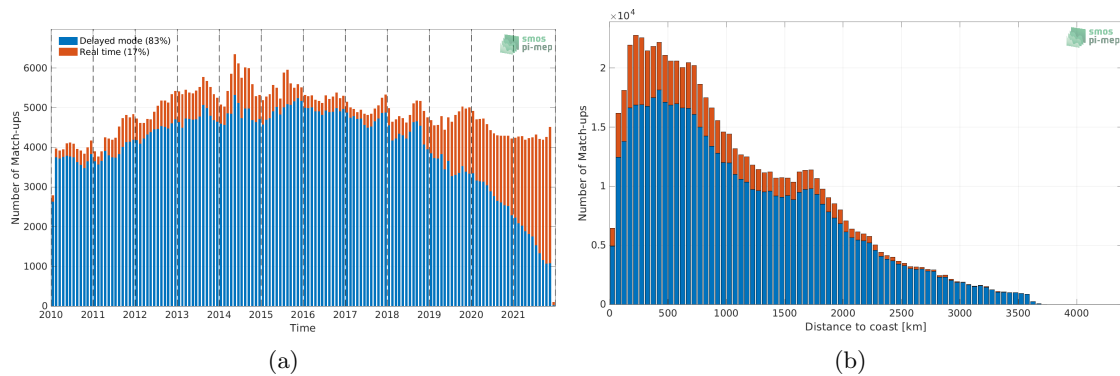
Figure 1: Number of match-ups between Argo and SMOS SSS L3 v7 - 9 Days (CATDS-CECOS-LOCEAN) SSS as a function of time (a) and as function of the distance to coast (b) over the Pacific Ocean Pi-MEP region and for the full satellite product period.
