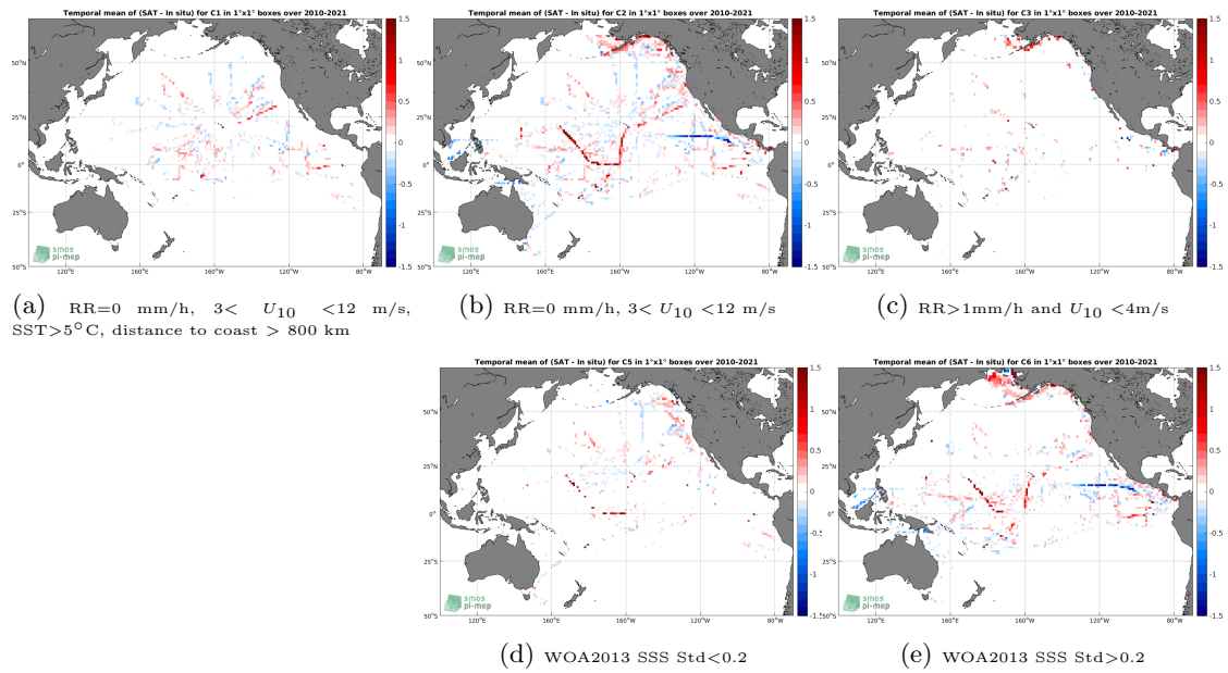
Figure 12: Temporal mean gridded over spatial boxes of size 1^\circ \times 1^\circ of \Delta SSS (SMOS SSS L3 v7 - 18 Days (CATDS-CECOS-LOCEAN) - TSG (SAMOS)) for 5 different subdatasets corresponding to:RR=0 mm/h, 3 < U_{10} < 12 m/s, SST>5°C, distance to coast > 800 km (a), RR=0 mm/h, 3 < U_{10} < 12 m/s (b), RR>1mm/h and U_{10} < 4 m/s (c), WOA2013 SSS Std<0.2 (d), WOA2013 SSS Std>0.2 (e).
