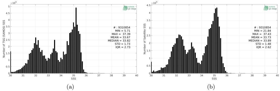
Figure 2: Histograms of SSS from TSG (SAMOS) (a) and SMOS SSS L3 v7 - 18 Days (CATDS-CECOS-LOCEAN) (b) considering all match-up pairs per bins of 0.1 over the Pacific Ocean Pi-MEP region and for the full satellite product period.
