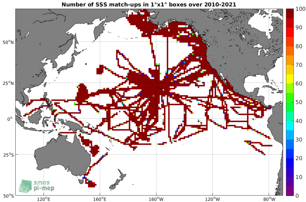
Figure 4: Number of SSS match-ups between TSG (SAMOS) SSS and the SMOS SSS L3 v7 - 18 Days (CATDS-CECOS-LOCEAN) SSS product for the Pacific Ocean Pi-MEP region over 1^\circ \times 1^\circ boxes and for the full satellite product period.
