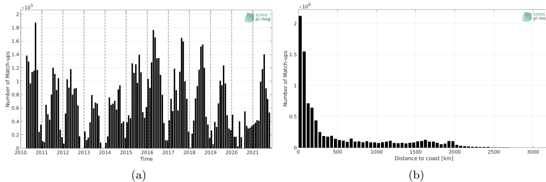
Figure 1: Number of match-ups between TSG (SAMOS) and SMOS SSS L3 v7 - 18 Days (CATDS-CECOS-LOCEAN) SSS as a function of time (a) and as function of the distance to coast (b) over the Pacific Ocean Pi-MEP region and for the full satellite product period.
