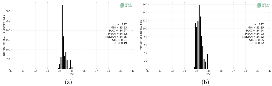
Figure 2: Histograms of SSS from TSG (Polarstern) (a) and SMOS SSS L3 v7 - 18 Days (CATDS-CECOS-LOCEAN) (b) considering all match-up pairs per bins of 0.1 over the Pacific Ocean Pi-MEP region and for the full satellite product period.
