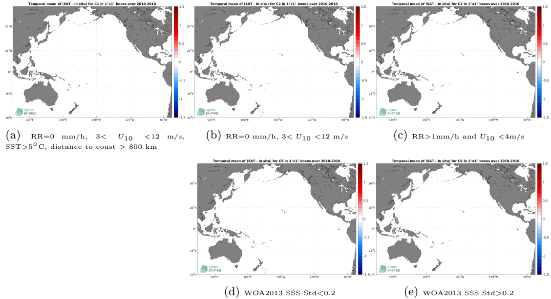
Figure 12: Temporal mean gridded over spatial boxes of size 1^{\circ}\times 1^{\circ} of \Delta\text{SSS} (SMOS SSS L3 v7 - 18 Days (CATDS-CECOS-LOCEAN) - TSG (Polarstern)) for 5 different subdatasets corresponding to:RR=0 mm/h, 3 < U_{10} < 12 m/s, SST >5^{\circ}\text{C} , distance to coast > 800 km (a), RR=0 mm/h, 3 < U_{10} < 12 m/s (b), RR >1 mm/h and U_{10} < 4 m/s (c), WOA2013 SSS Std <0.2 (d), WOA2013 SSS Std >0.2 (e).
