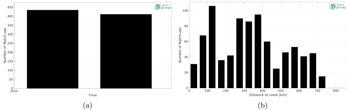
Figure 1: Number of match-ups between TSG (Polarstern) and SMOS SSS L3 v7 - 18 Days (CATDS-CECOS-LOCEAN) SSS as a function of time (a) and as function of the distance to coast (b) over the Pacific Ocean Pi-MEP region and for the full satellite product period.
