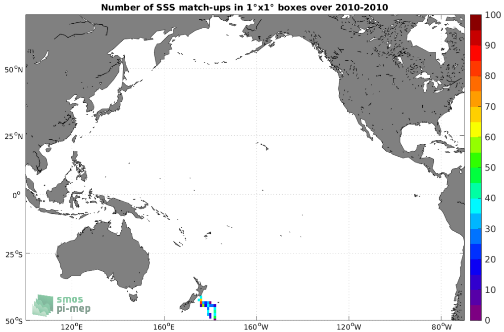
Figure 4: Number of SSS match-ups between TSG (Polarstern) SSS and the SMOS SSS L3 v7 - 18 Days (CATDS-CECOS-LOCEAN) SSS product for the Pacific Ocean Pi-MEP region over 1^\circ \times 1^\circ boxes and for the full satellite product period.
