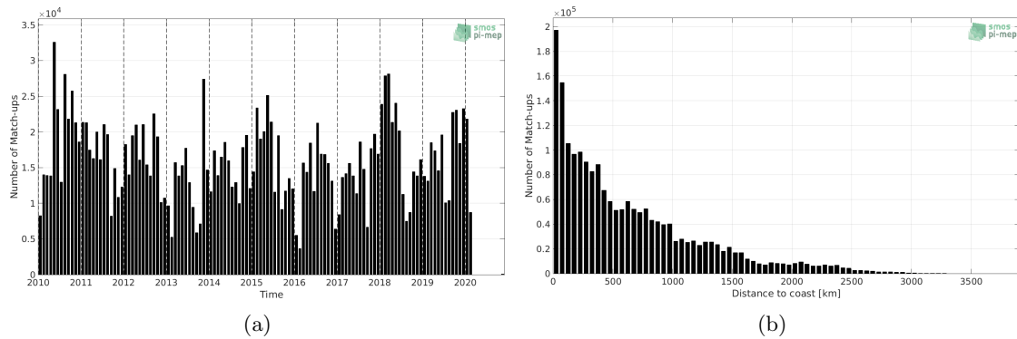
Figure 1: Number of match-ups between TSG (LEGOS-DM) and SMOS SSS L3 v7 - 18 Days (CATDS-CECOS-LOCEAN) SSS as a function of time (a) and as function of the distance to coast (b) over the Pacific Ocean Pi-MEP region and for the full satellite product period.
