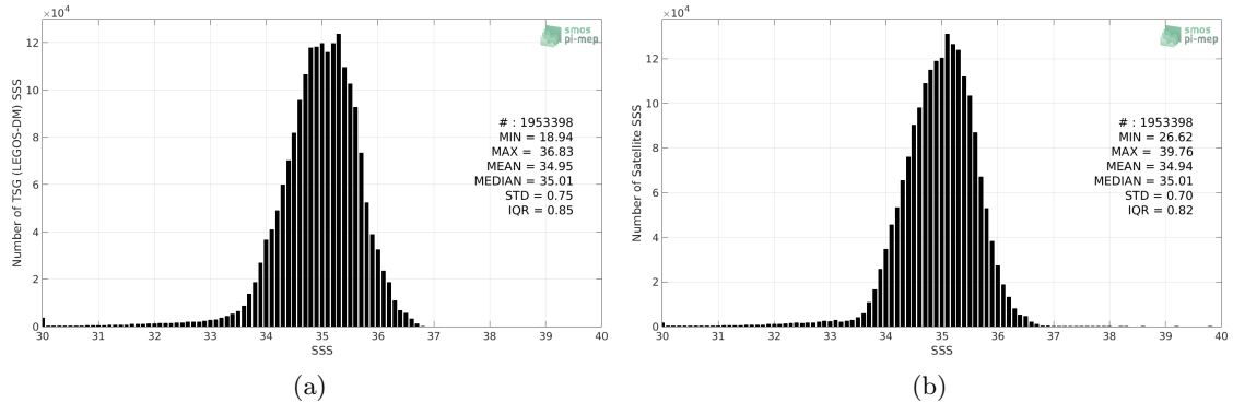
Figure 2: Histograms of SSS from TSG (LEGOS-DM) (a) and SMOS SSS L3 v7 - 18 Days (CATDS-CECOS-LOCEAN) (b) considering all match-up pairs per bins of 0.1 over the Pacific Ocean Pi-MEP region and for the full satellite product period.
