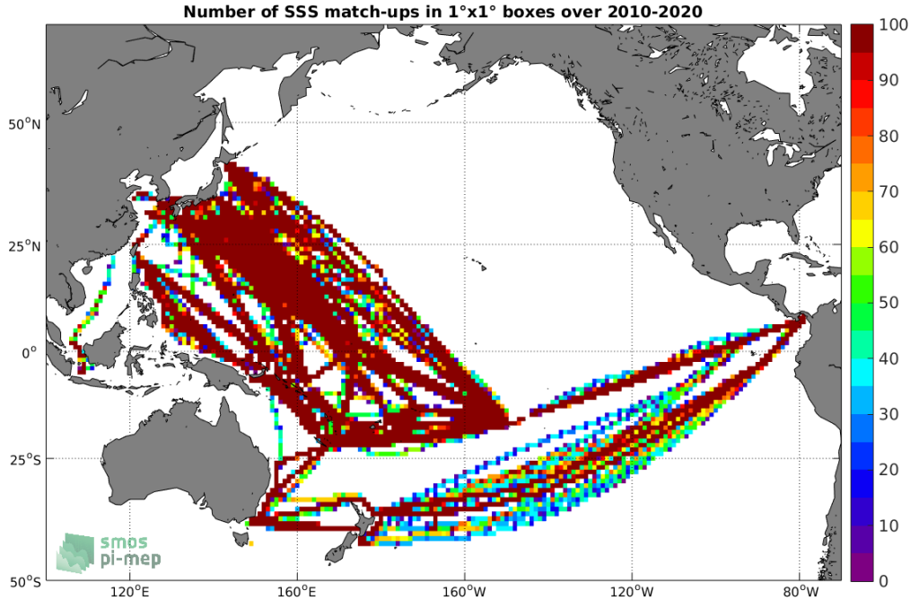
Figure 4: Number of SSS match-ups between TSG (LEGOS-DM) SSS and the SMOS SSS L3 v7 - 18 Days (CATDS-CECOS-LOCEAN) SSS product for the Pacific Ocean Pi-MEP region over 1^\circ \times 1^\circ boxes and for the full satellite product period.
