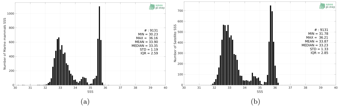
Figure 2: Histograms of SSS from Marine mammals (a) and SMOS SSS L3 v7 - 18 Days (CATDS-CECOS-LOCEAN) (b) considering all match-up pairs per bins of 0.1 over the Pacific Ocean Pi-MEP region and for the full satellite product period.
