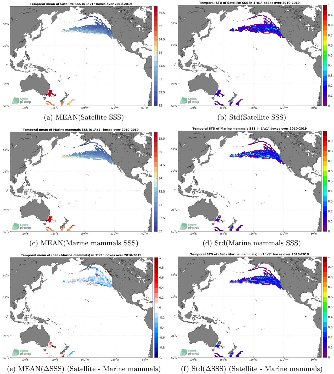
Figure 6: Temporal mean (left) and Std (right) of SSS from SMOS SSS L3 v7 - 18 Days (CATDS-CECOS-LOCEAN) (top), Marine mammals (middle), and of \Delta SSS (Satellite - Marine mammals). Only match-up pairs are used to generate these maps.
