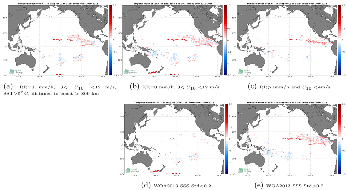
Figure 11: Temporal mean gridded over spatial boxes of size 1^\circ \times 1^\circ of \Delta\text{SSS} (SMOS SSS L3 v7 - 18 Days (CATDS-CECOS-LOCEAN) - Surface drifters) for 5 different subdatasets corresponding to:RR=0 mm/h, 3 < U_{10} < 12 m/s, SST >5^\circ\text{C} , distance to coast > 800 km (a), RR=0 mm/h, 3 < U_{10} < 12 m/s (b), RR >1 mm/h and U_{10} < 4 m/s (c), WOA2013 SSS Std <0.2 (d), WOA2013 SSS Std >0.2 (e).
