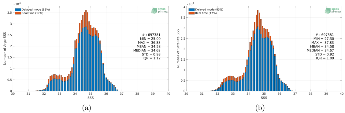
Figure 2: Histograms of SSS from Argo (a) and SMOS SSS L3 v7 - 18 Days (CATDS-CECOS-LOCEAN) (b) considering all match-up pairs per bins of 0.1 over the Pacific Ocean Pi-MEP region and for the full satellite product period.
