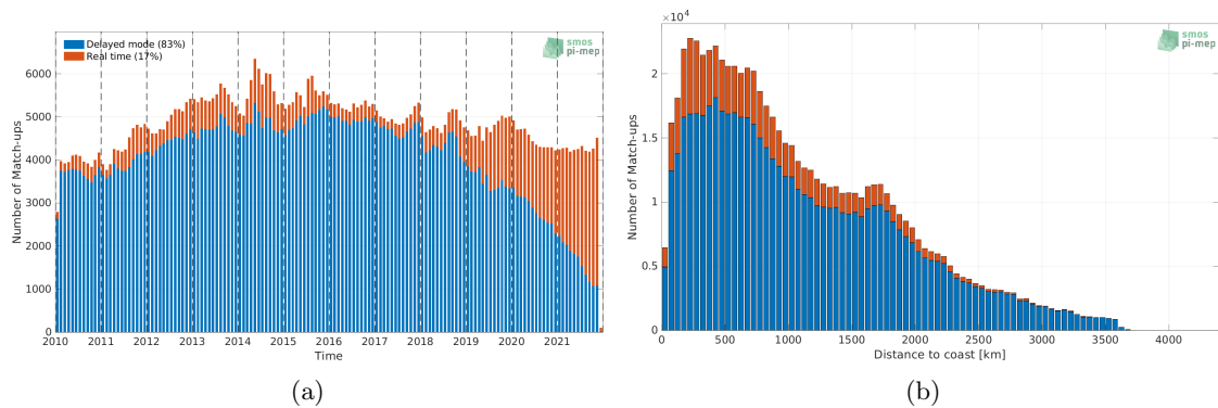
Figure 1: Number of match-ups between Argo and SMOS SSS L3 v7 - 18 Days (CATDS-CECOS-LOCEAN) SSS as a function of time (a) and as function of the distance to coast (b) over the Pacific Ocean Pi-MEP region and for the full satellite product period.
