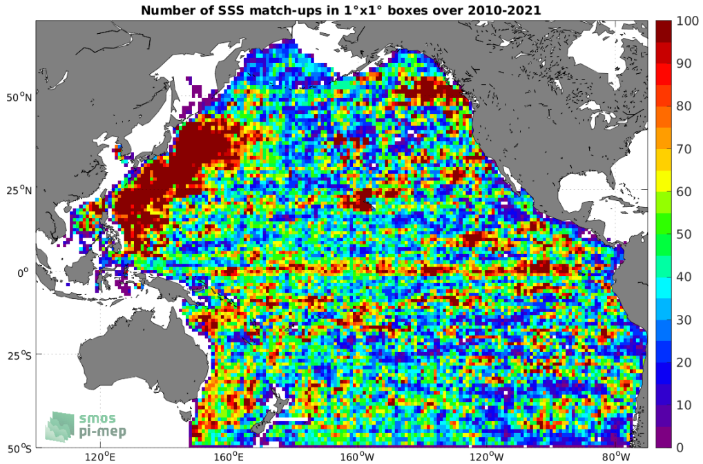
Figure 4: Number of SSS match-ups between Argo SSS and the SMOS SSS L3 v7 - 18 Days (CATDS-CECOS-LOCEAN) SSS product for the Pacific Ocean Pi-MEP region over 1^\circ \times 1^\circ boxes and for the full satellite product period.
