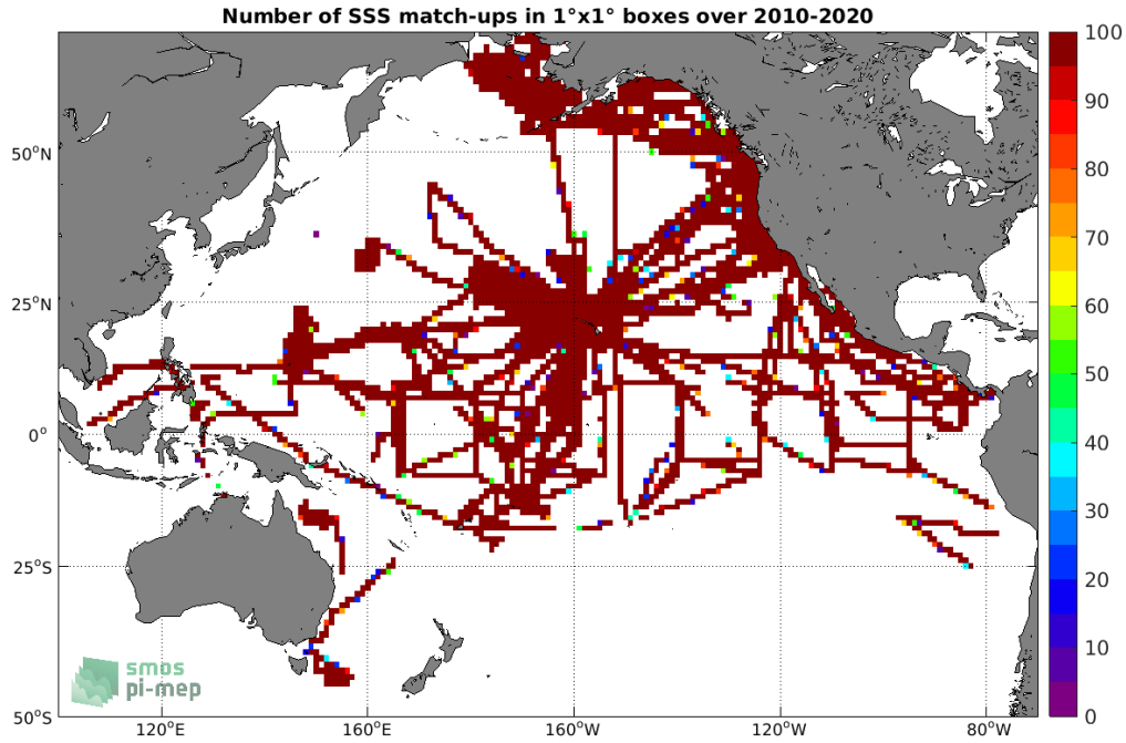
Figure 4: Number of SSS match-ups between TSG (SAMOS) SSS and the SMOS SSS L3 v5 - 9 Days (CATDS-CECOS-LOCEAN) SSS product for the Pacific Ocean Pi-MEP region over 1°x1° boxes and for the full satellite product period.
