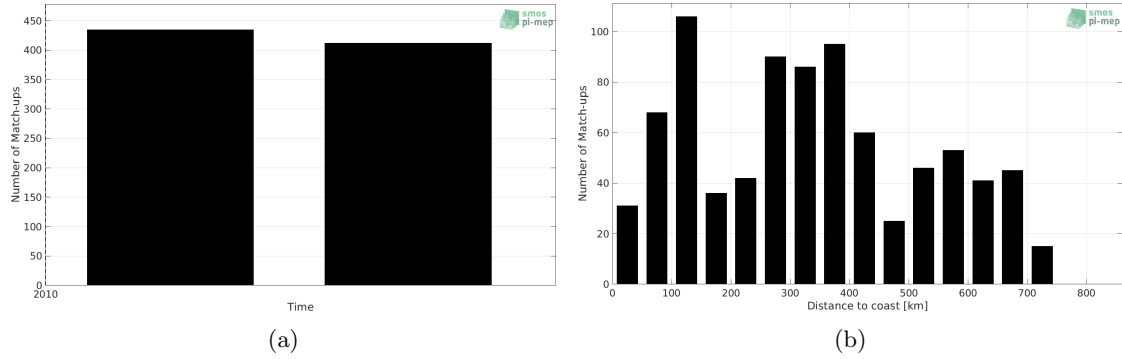
Figure 1: Number of match-ups between TSG (Polarstern) and SMOS SSS L3 v5 - 9 Days (CATDS-CECOS-LOCEAN) SSS as a function of time (a) and as function of the distance to coast (b) over the Pacific Ocean Pi-MEP region and for the full satellite product period.
