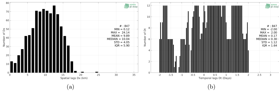
Figure 5: Histograms of the spatial (a) and temporal (b) lags between the location/time of the TSG (Polarstern) measurement and the date of the corresponding SMOS SSS L3 v5 - 9 Days (CATDS-CECOS-LOCEAN) SSS pixel.
