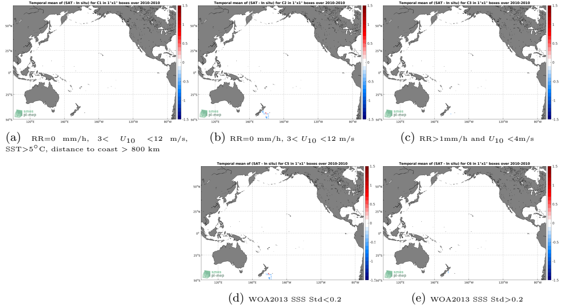
Figure 12: Temporal mean gridded over spatial boxes of size 1^{\circ}\times 1^{\circ} of \Delta\text{SSS} (SMOS SSS L3 v5 - 9 Days (CATDS-CECOS-LOCEAN) - TSG (Polarstern)) for 5 different subdatasets corresponding to: \text{RR}=0 mm/h, 3 < U_{10} < 12 m/s, \text{SST} > 5^{\circ}\text{C} , distance to coast > 800 km (a), \text{RR}=0 mm/h, 3 < U_{10} < 12 m/s (b), \text{RR} > 1 mm/h and U_{10} < 4 m/s (c), WOA2013 SSS Std < 0.2 (d), WOA2013 SSS Std > 0.2 (e).
