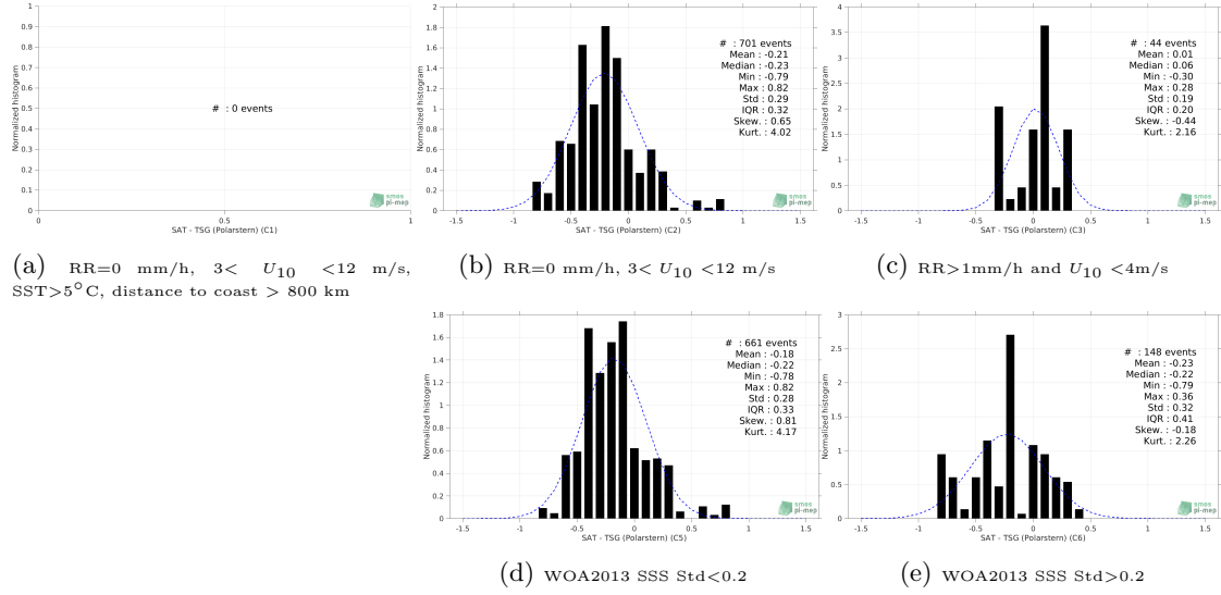
Figure 13: Normalized histogram of \Delta\text{SSS} (SMOS SSS L3 v5 - 9 Days (CATDS-CECOS-LOCEAN) - TSG (Polarstern)) for 5 different subdatasets corresponding to: RR=0 mm/h, 3 < U_{10} < 12 m/s, SST > 5^\circ\text{C} , distance to coast > 800 km (a), RR=0 mm/h, 3 < U_{10} < 12 m/s (b), RR > 1\text{mm/h} and U_{10} < 4\text{m/s} (c), WOA2013 SSS Std < 0.2 (d), WOA2013 SSS Std > 0.2 (e).
