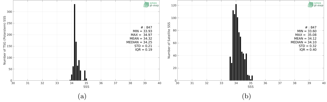
Figure 2: Histograms of SSS from TSG (Polarstern) (a) and SMOS SSS L3 v5 - 9 Days (CATDS-CECOS-LOCEAN) (b) considering all match-up pairs per bins of 0.1 over the Pacific Ocean Pi-MEP region and for the full satellite product period.
