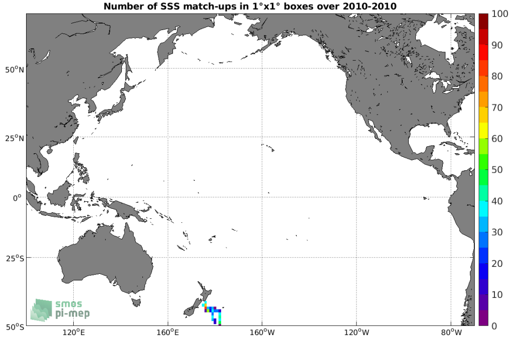
Figure 4: Number of SSS match-ups between TSG (Polarstern) SSS and the SMOS SSS L3 v5 - 9 Days (CATDS-CECOS-LOCEAN) SSS product for the Pacific Ocean Pi-MEP region over 1^\circ \times 1^\circ boxes and for the full satellite product period.
