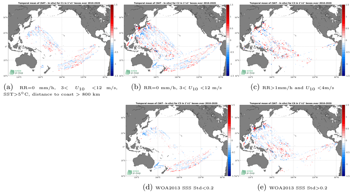
Figure 12: Temporal mean gridded over spatial boxes of size 1^\circ \times 1^\circ of \Delta SSS (SMOS SSS L3 v5 - 9 Days (CATDS-CECOS-LOCEAN) - TSG (LEGOS-DM)) for 5 different subdatasets corresponding to: RR=0 mm/h, 3 < U_{10} < 12 m/s, SST >5^\circ\text{C} , distance to coast > 800 km (a), RR=0 mm/h, 3 < U_{10} < 12 m/s (b), RR >1 mm/h and U_{10} < 4 m/s (c), WOA2013 SSS Std <0.2 (d), WOA2013 SSS Std >0.2 (e).
