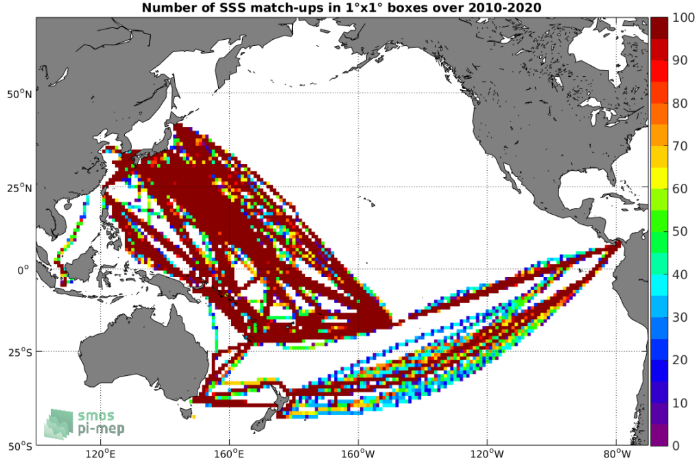
Figure 4: Number of SSS match-ups between TSG (LEGOS-DM) SSS and the SMOS SSS L3 v5 - 9 Days (CATDS-CECOS-LOCEAN) SSS product for the Pacific Ocean Pi-MEP region over 1^\circ \times 1^\circ boxes and for the full satellite product period.
