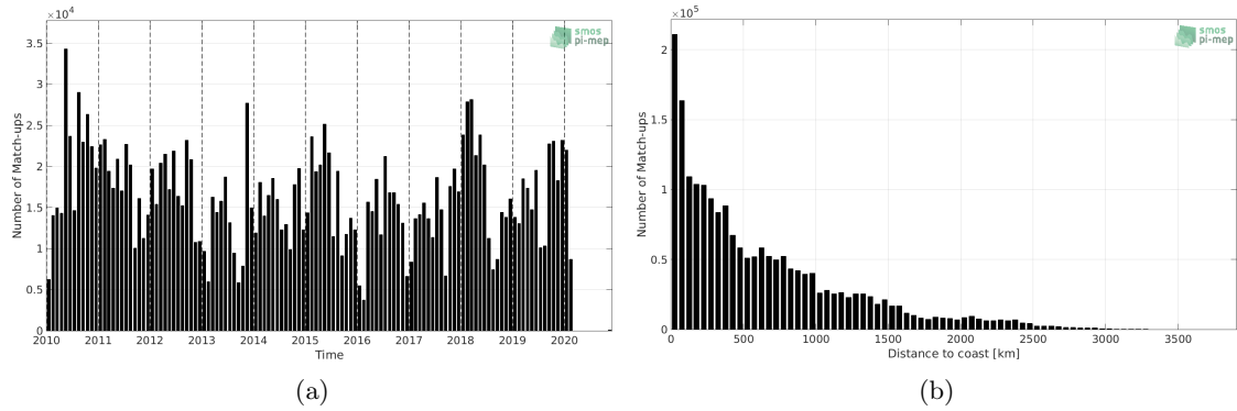
Figure 1: Number of match-ups between TSG (LEGOS-DM) and SMOS SSS L3 v5 - 9 Days (CATDS-CECOS-LOCEAN) SSS as a function of time (a) and as function of the distance to coast (b) over the Pacific Ocean Pi-MEP region and for the full satellite product period.
