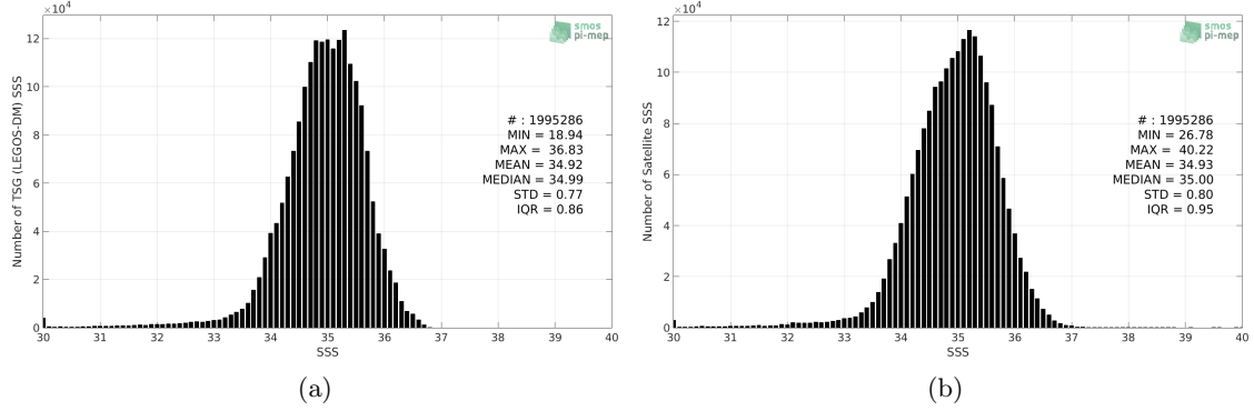
Figure 2: Histograms of SSS from TSG (LEGOS-DM) (a) and SMOS SSS L3 v5 - 9 Days (CATDS-CECOS-LOCEAN) (b) considering all match-up pairs per bins of 0.1 over the Pacific Ocean Pi-MEP region and for the full satellite product period.
