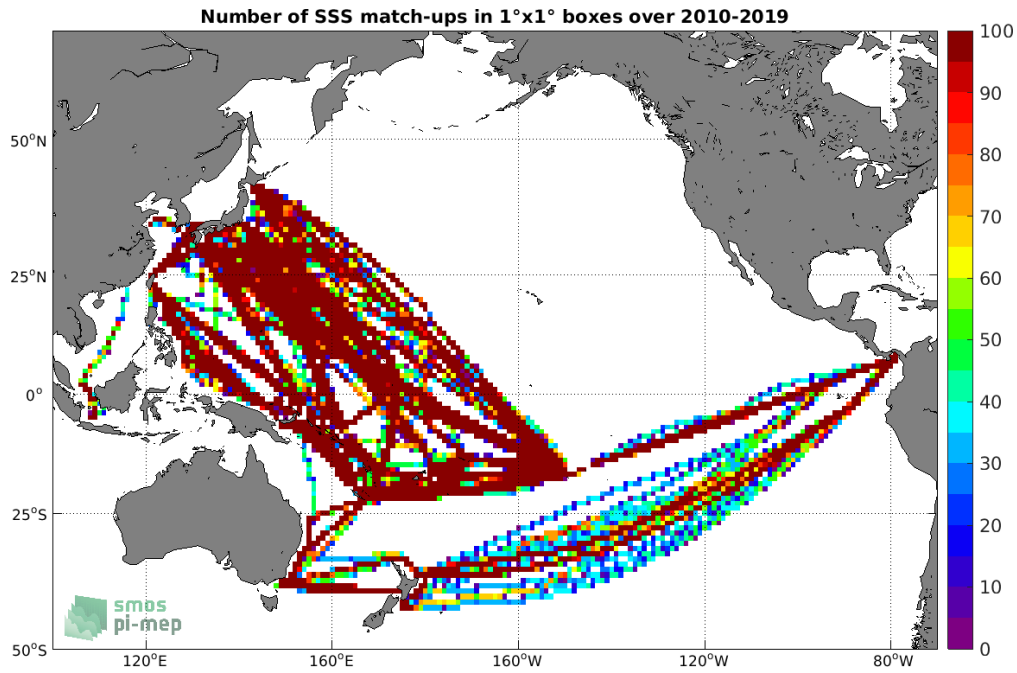
Figure 4: Number of SSS match-ups between TSG (LEGOS-DM) SSS and the SMOS SSS L3 v5 - 9 Days (CATDS-CECOS-LOCEAN) SSS product for the Pacific Ocean Pi-MEP region over 1°x1° boxes and for the full satellite product period.
