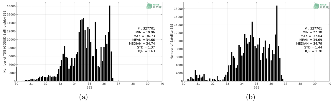
Figure 2: Histograms of SSS from TSG (GOSUD-Sailing-ship) (a) and SMOS SSS L3 v5 - 9 Days (CATDS-CECOS-LOCEAN) (b) considering all match-up pairs per bins of 0.1 over the Pacific Ocean Pi-MEP region and for the full satellite product period.
