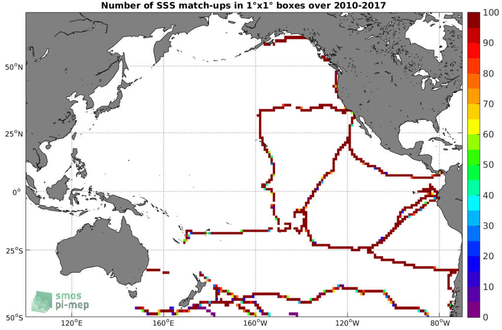
Figure 4: Number of SSS match-ups between TSG (GOSUD-Sailing-ship) SSS and the SMOS SSS L3 v5 - 9 Days (CATDS-CECOS-LOCEAN) SSS product for the Pacific Ocean Pi-MEP region over 1^\circ \times 1^\circ boxes and for the full satellite product period.
