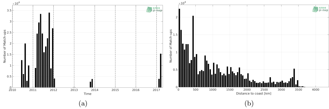
Figure 1: Number of match-ups between TSG (GOSUD-Sailing-ship) and SMOS SSS L3 v5 - 9 Days (CATDS-CECOS-LOCEAN) SSS as a function of time (a) and as function of the distance to coast (b) over the Pacific Ocean Pi-MEP region and for the full satellite product period.
