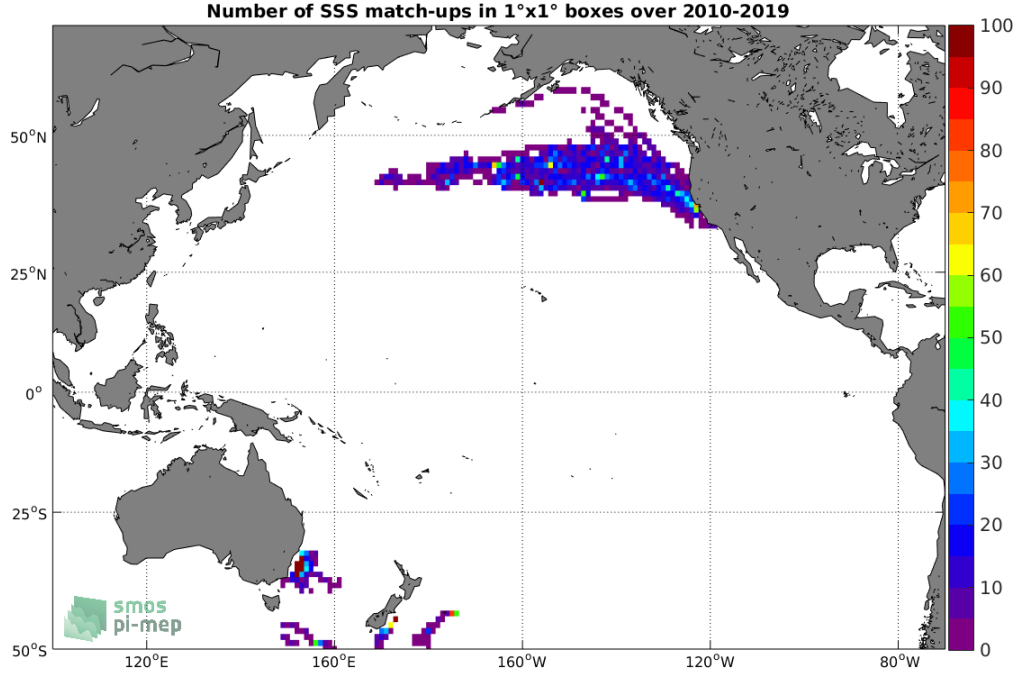
Figure 4: Number of SSS match-ups between Marine mammals SSS and the SMOS SSS L3 v5 - 9 Days (CATDS-CECOS-LOCEAN) SSS product for the Pacific Ocean Pi-MEP region over 1^\circ \times 1^\circ boxes and for the full satellite product period.
