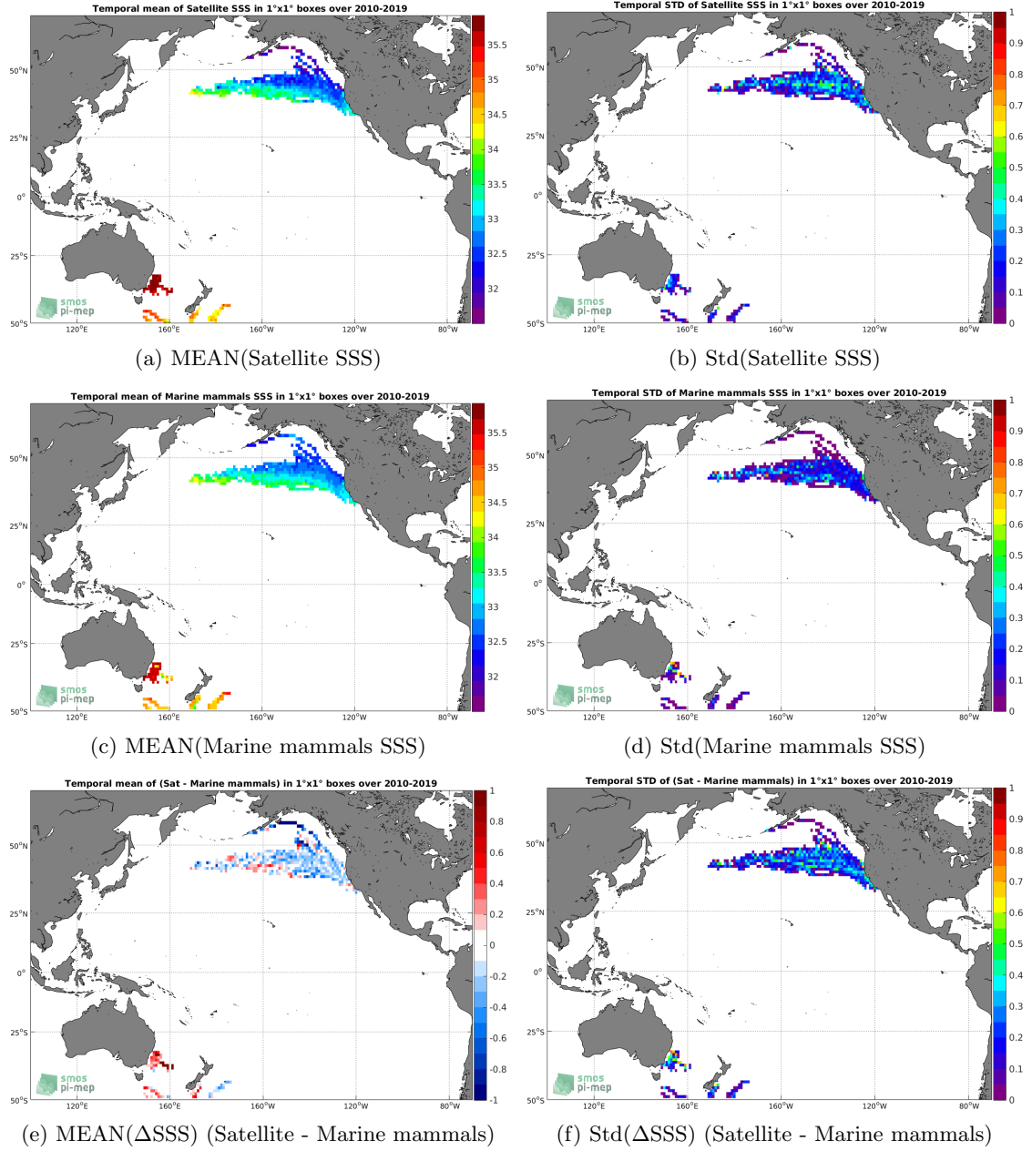
Figure 6: Temporal mean (left) and Std (right) of SSS from SMOS SSS L3 v5 - 9 Days (CATDS-CECOS-LOCEAN) (top), Marine mammals (middle), and of \Delta SSS (Satellite - Marine mammals). Only match-up pairs are used to generate these maps.
