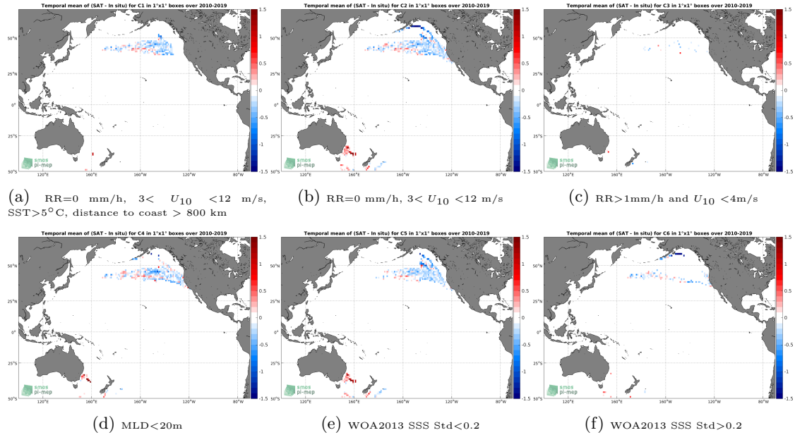
Figure 12: Temporal mean gridded over spatial boxes of size 1^{\circ} \times 1^{\circ} of \Delta\text{SSS} (SMOS SSS L3 v5 - 9 Days (CATDS-CECOS-LOCEAN) - Marine mammals) for 6 different subdatasets corresponding to: \text{RR}=0 mm/h, 3 < U_{10} < 12 m/s, \text{SST} > 5^{\circ}\text{C} , distance to coast > 800 km (a), \text{RR}=0 mm/h, 3 < U_{10} < 12 m/s (b), \text{RR} > 1\text{mm/h} and U_{10} < 4\text{m/s} (c), \text{MLD} < 20\text{m} (d), \text{WOA2013 SSS Std} < 0.2 (e), \text{WOA2013 SSS Std} > 0.2 (f).
