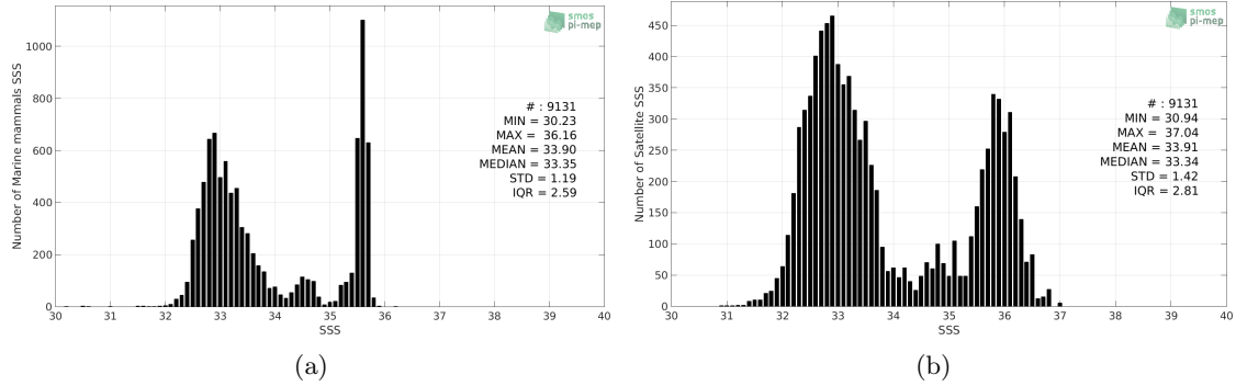
Figure 2: Histograms of SSS from Marine mammals (a) and SMOS SSS L3 v5 - 9 Days (CATDS-CECOS-LOCEAN) (b) considering all match-up pairs per bins of 0.1 over the Pacific Ocean Pi-MEP region and for the full satellite product period.
