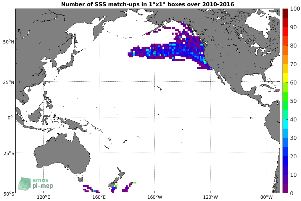
Figure 4: Number of SSS match-ups between Sea mammals SSS and the SMOS SSS L3 v5 - 9 Days (CATDS-CECOS-LOCEAN) SSS product for the Pacific Ocean Pi-MEP region over 1^\circ \times 1^\circ boxes and for the full satellite product period.
