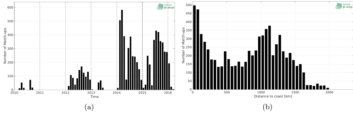
Figure 1: Number of match-ups between Sea mammals and SMOS SSS L3 v5 - 9 Days (CATDS-CECOS-LOCEAN) SSS as a function of time (a) and as function of the distance to coast (b) over the Pacific Ocean Pi-MEP region and for the full satellite product period.
