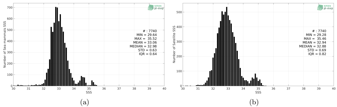
Figure 2: Histograms of SSS from Sea mammals (a) and SMOS SSS L3 v5 - 9 Days (CATDS-CECOS-LOCEAN) (b) considering all match-up pairs per bins of 0.1 over the Pacific Ocean Pi-MEP region and for the full satellite product period.
