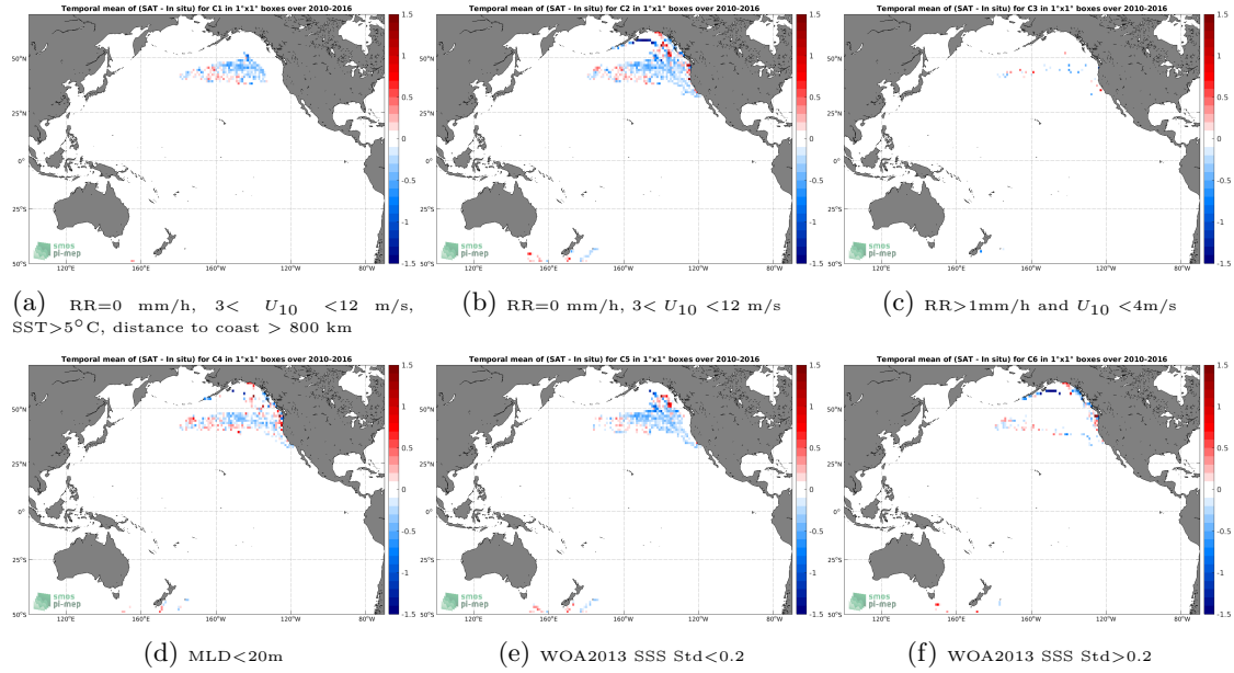
Figure 12: Temporal mean gridded over spatial boxes of size 1^\circ \times 1^\circ of \Delta SSS (SMOS SSS L3 v5 - 9 Days (CATDS-CECOS-LOCEAN) - Sea mammals) for 6 different subdatasets corresponding to: RR=0 mm/h, 3 < U_{10} < 12 m/s, SST > 5^\circ C , distance to coast > 800 km (a), RR=0 mm/h, 3 < U_{10} < 12 m/s (b), RR > 1 mm/h and U_{10} < 4 m/s (c), MLD < 20 m (d), WOA2013 SSS Std < 0.2 (e), WOA2013 SSS Std > 0.2 (f).
