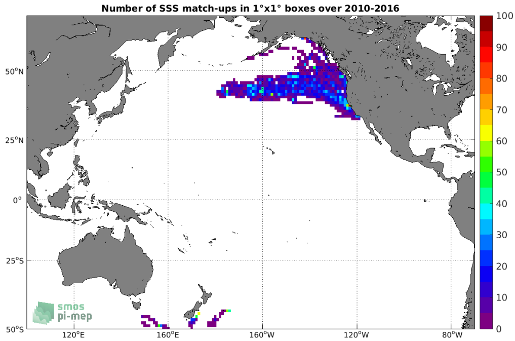
Figure 4: Number of SSS match-ups between Sea mammals SSS and the SMOS SSS L3 v5 - 9 Days (CATDS-CECOS-LOCEAN) SSS product for the Pacific Ocean Pi-MEP region over 1°x1° boxes and for the full satellite product period.
