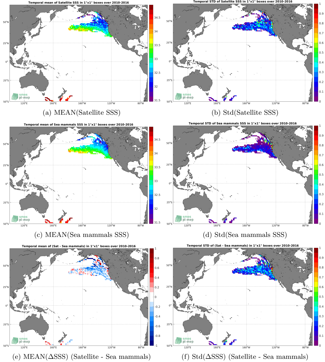
Figure 6: Temporal mean (left) and Std (right) of SSS from SMOS SSS L3 v5 - 9 Days (CATDS-CECOS-LOCEAN) (top), Sea mammals (middle), and of \Delta SSS (Satellite - Sea mammals). Only match-up pairs are used to generate these maps.
