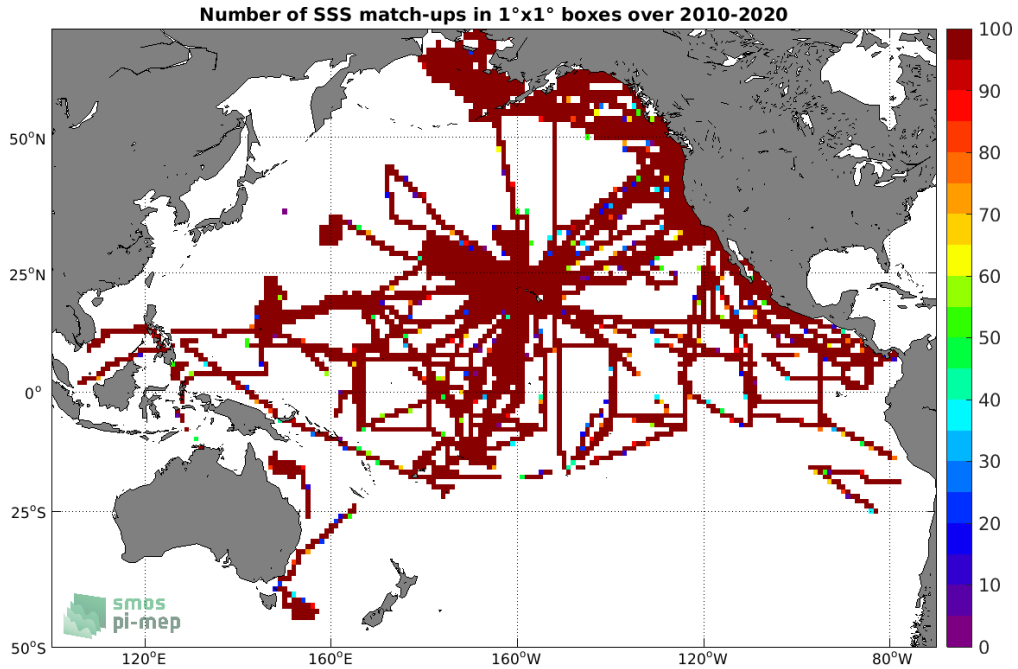
Figure 4: Number of SSS match-ups between TSG (SAMOS) SSS and the SMOS SSS L3 v5 - 18 Days (CATDS-CECOS-LOCEAN) SSS product for the Pacific Ocean Pi-MEP region over 1°x1° boxes and for the full satellite product period.
