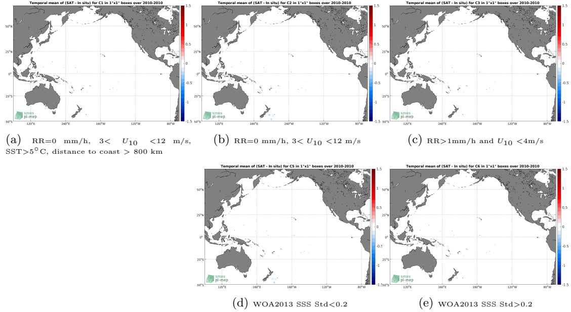
Figure 12: Temporal mean gridded over spatial boxes of size 1^{\circ}\times 1^{\circ} of \Delta\text{SSS} (SMOS SSS L3 v5 - 18 Days (CATDS-CECOS-LOCEAN) - TSG (Polarstern)) for 5 different subdatasets corresponding to: \text{RR}=0 mm/h, 3 < U_{10} < 12 m/s, \text{SST} > 5^{\circ}\text{C} , distance to coast > 800 km (a), \text{RR}=0 mm/h, 3 < U_{10} < 12 m/s (b), \text{RR} > 1 mm/h and U_{10} < 4 m/s (c), WOA2013 SSS Std < 0.2 (d), WOA2013 SSS Std > 0.2 (e).
