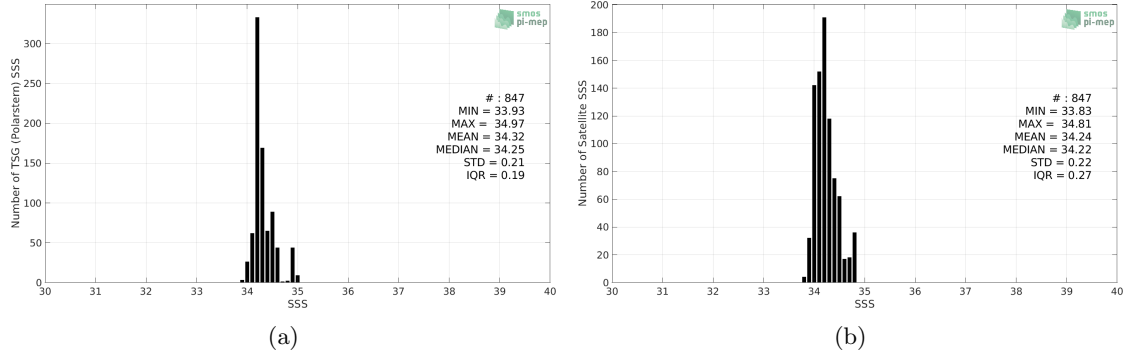
Figure 2: Histograms of SSS from TSG (Polarstern) (a) and SMOS SSS L3 v5 - 18 Days (CATDS-CECOS-LOCEAN) (b) considering all match-up pairs per bins of 0.1 over the Pacific Ocean Pi-MEP region and for the full satellite product period.
