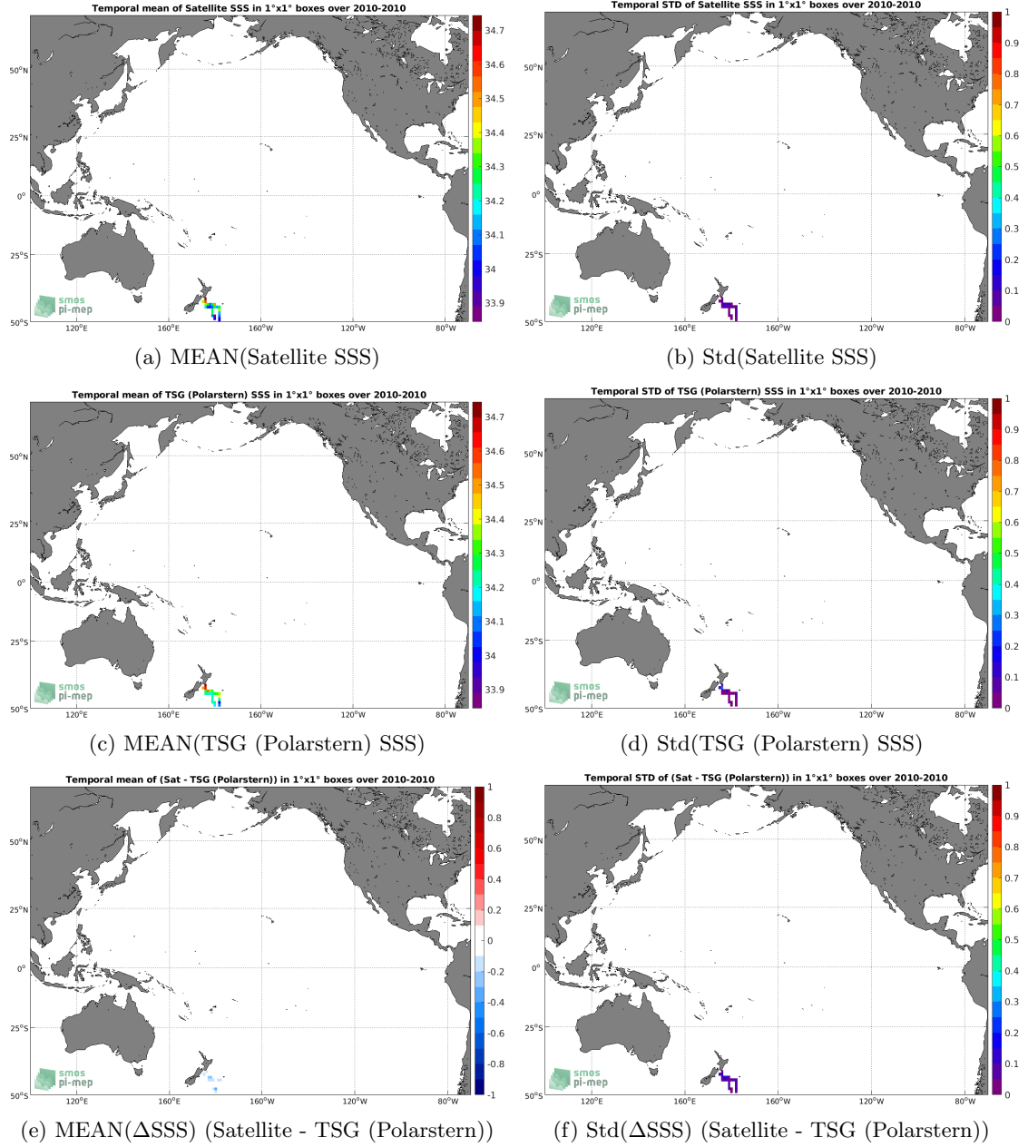
Figure 6: Temporal mean (left) and Std (right) of SSS from SMOS SSS L3 v5 - 18 Days (CATDS-CECOS-LOCEAN) (top), TSG (Polarstern) (middle), and of ΔSSS (Satellite - TSG (Polarstern)). Only match-up pairs are used to generate these maps.
