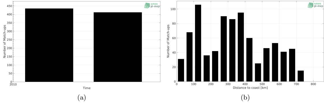
Figure 1: Number of match-ups between TSG (Polarstern) and SMOS SSS L3 v5 - 18 Days (CATDS-CECOS-LOCEAN) SSS as a function of time (a) and as function of the distance to coast (b) over the Pacific Ocean Pi-MEP region and for the full satellite product period.
