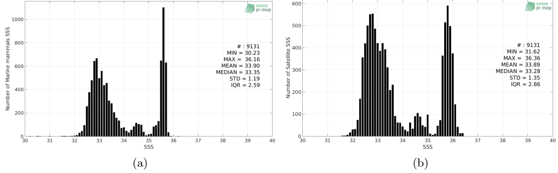
Figure 2: Histograms of SSS from Marine mammals (a) and SMOS SSS L3 v5 - 18 Days (CATDS-CECOS-LOCEAN) (b) considering all match-up pairs per bins of 0.1 over the Pacific Ocean Pi-MEP region and for the full satellite product period.
