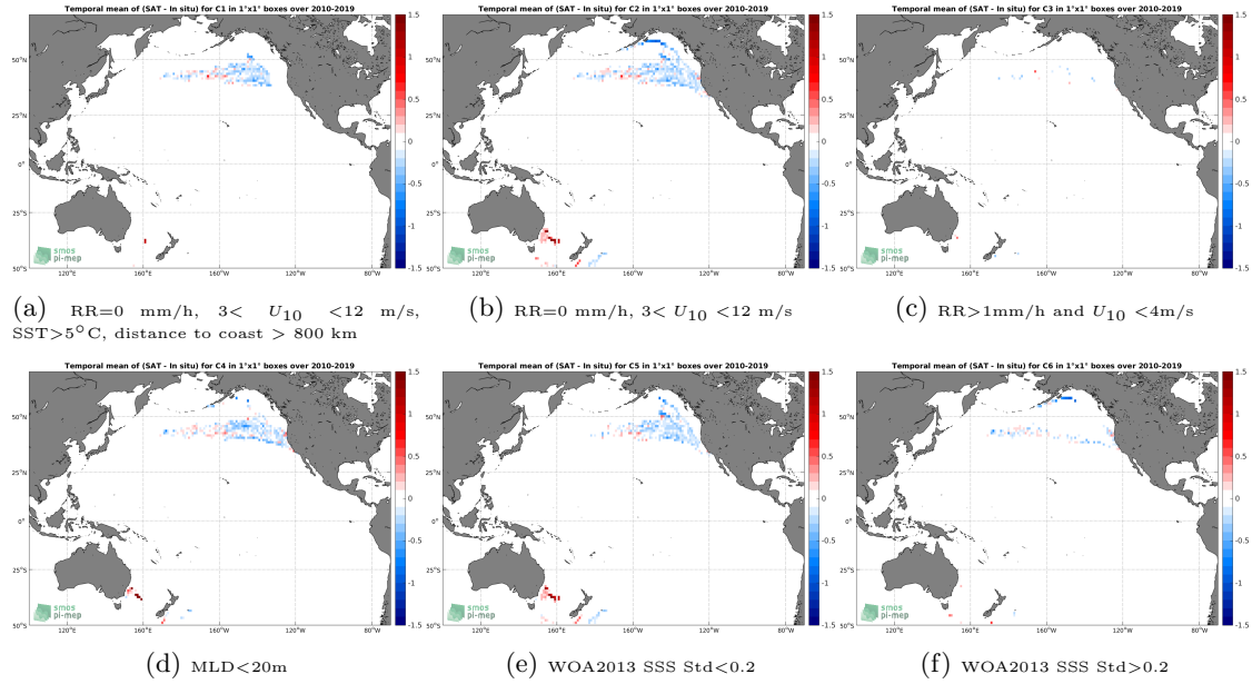
Figure 12: Temporal mean gridded over spatial boxes of size 1^{\circ} \times 1^{\circ} of \Delta\text{SSS} (SMOS SSS L3 v5 - 18 Days (CATDS-CECOS-LOCEAN) - Marine mammals) for 6 different subdatasets corresponding to: \text{RR}=0 mm/h, 3 < U_{10} < 12 m/s, \text{SST} > 5^{\circ}\text{C} , distance to coast > 800 km (a), \text{RR}=0 mm/h, 3 < U_{10} < 12 m/s (b), \text{RR} > 1\text{mm/h} and U_{10} < 4\text{m/s} (c), \text{MLD} < 20\text{m} (d), \text{WOA2013 SSS Std} < 0.2 (e), \text{WOA2013 SSS Std} > 0.2 (f).
