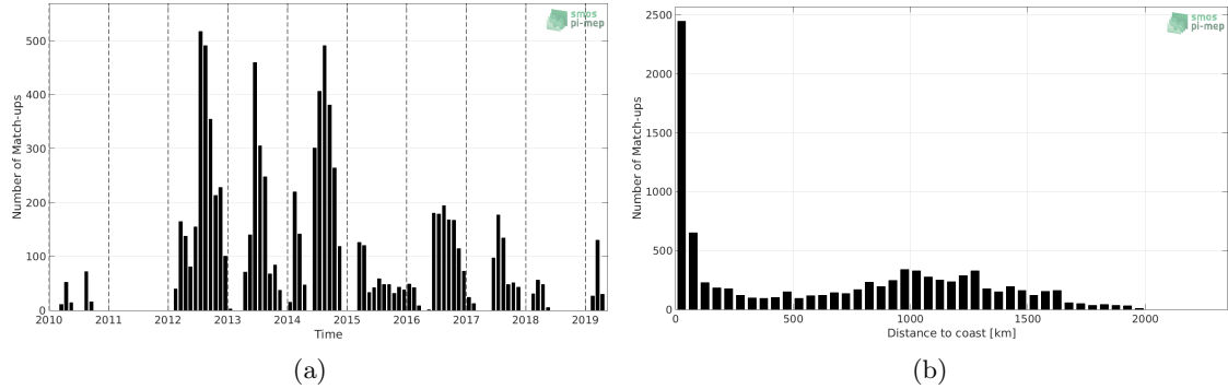
Figure 1: Number of match-ups between Marine mammals and SMOS SSS L3 v5 - 18 Days (CATDS-CECOS-LOCEAN) SSS as a function of time (a) and as function of the distance to coast (b) over the Pacific Ocean Pi-MEP region and for the full satellite product period.
