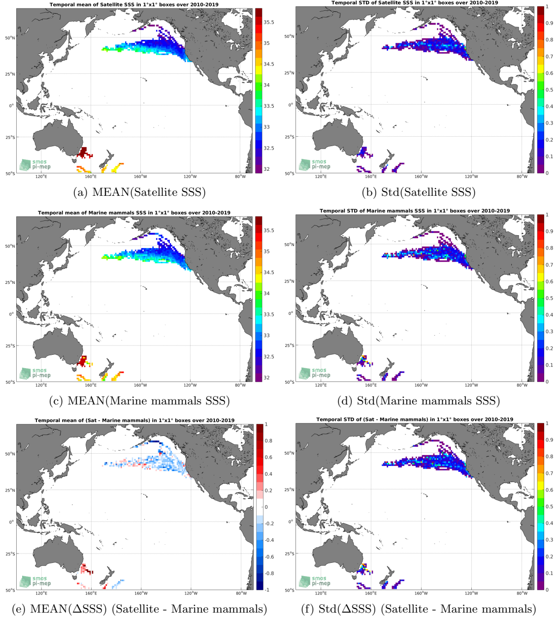
Figure 6: Temporal mean (left) and Std (right) of SSS from SMOS SSS L3 v5 - 18 Days (CATDS-CECOS-LOCEAN) (top), Marine mammals (middle), and of \Delta SSS (Satellite - Marine mammals). Only match-up pairs are used to generate these maps.
