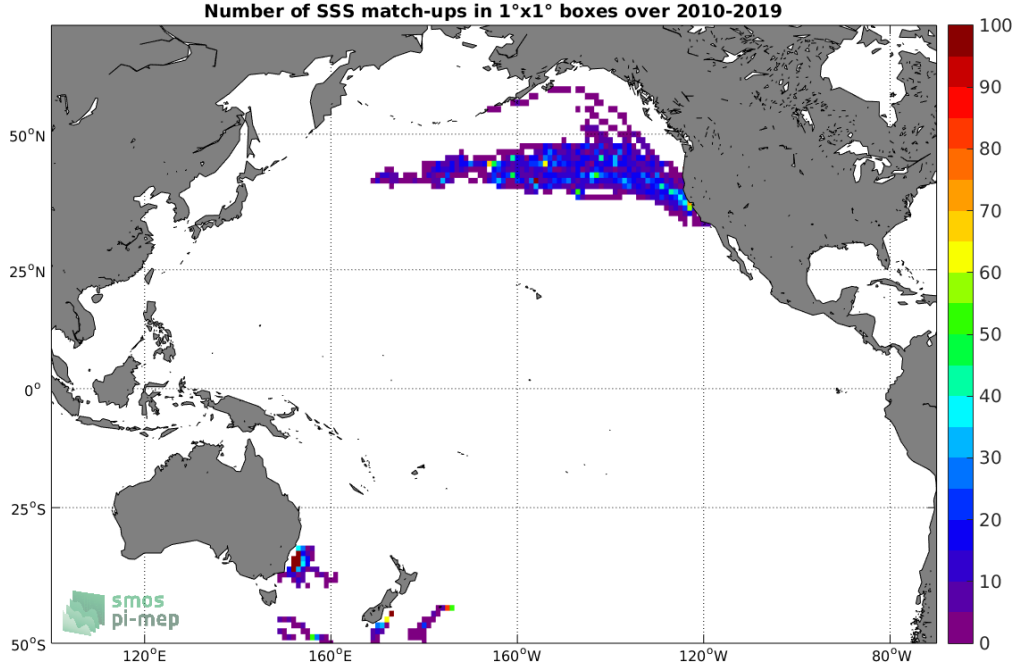
Figure 4: Number of SSS match-ups between Marine mammals SSS and the SMOS SSS L3 v5 - 18 Days (CATDS-CECOS-LOCEAN) SSS product for the Pacific Ocean Pi-MEP region over 1^\circ \times 1^\circ boxes and for the full satellite product period.
