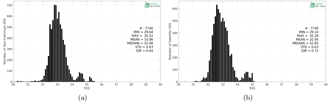
Figure 2: Histograms of SSS from Sea mammals (a) and SMOS SSS L3 v5 - 18 Days (CATDS-CECOS-LOCEAN) (b) considering all match-up pairs per bins of 0.1 over the Pacific Ocean Pi-MEP region and for the full satellite product period.
