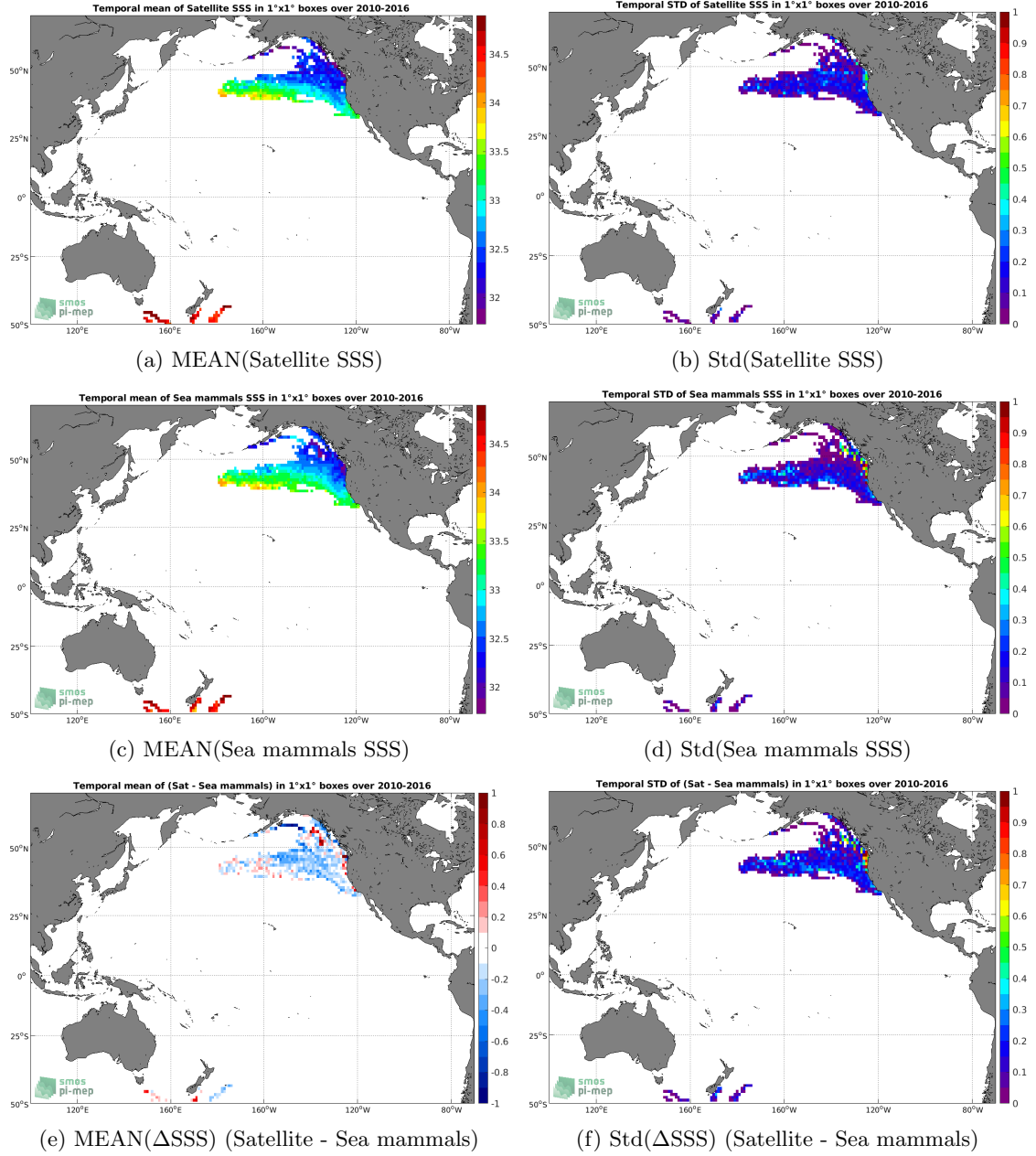
Figure 6: Temporal mean (left) and Std (right) of SSS from SMOS SSS L3 v5 - 18 Days (CATDS-CECOS-LOCEAN) (top), Sea mammals (middle), and of \Delta SSS (Satellite - Sea mammals). Only match-up pairs are used to generate these maps.
