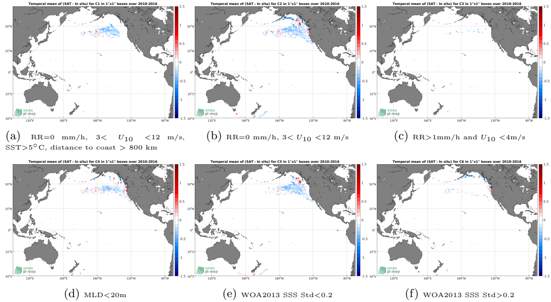
Figure 12: Temporal mean gridded over spatial boxes of size 1^\circ \times 1^\circ of \Delta SSS (SMOS SSS L3 v5 - 18 Days (CATDS-CECOS-LOCEAN) - Sea mammals) for 6 different subdatasets corresponding to: RR=0 mm/h, 3 < U_{10} < 12 m/s, SST > 5^\circ C , distance to coast > 800 km (a), RR=0 mm/h, 3 < U_{10} < 12 m/s (b), RR > 1 mm/h and U_{10} < 4 m/s (c), MLD < 20 m (d), WOA2013 SSS Std < 0.2 (e), WOA2013 SSS Std > 0.2 (f).
