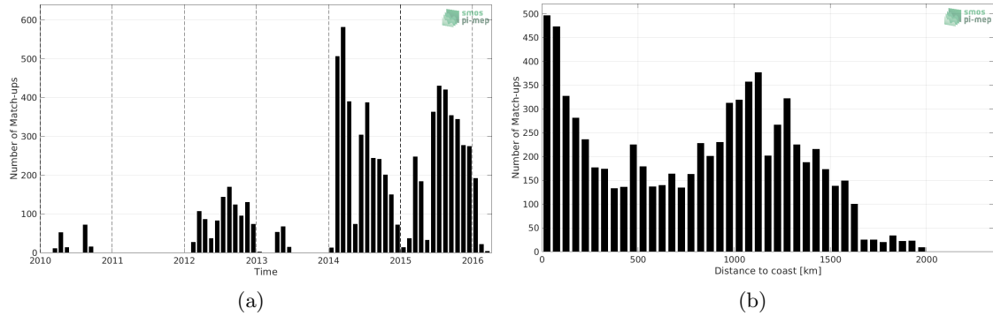
Figure 1: Number of match-ups between Sea mammals and SMOS SSS L3 v5 - 18 Days (CATDS-CECOS-LOCEAN) SSS as a function of time (a) and as function of the distance to coast (b) over the Pacific Ocean Pi-MEP region and for the full satellite product period.
