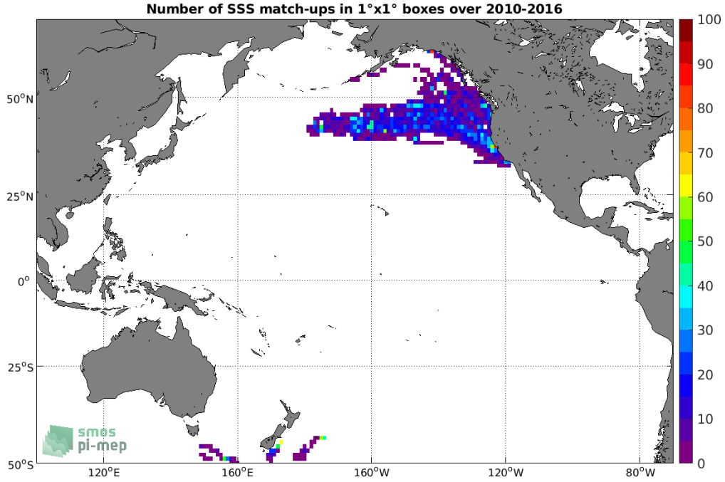
Figure 4: Number of SSS match-ups between Sea mammals SSS and the SMOS SSS L3 v5 - 18 Days (CATDS-CECOS-LOCEAN) SSS product for the Pacific Ocean Pi-MEP region over 1^\circ \times 1^\circ boxes and for the full satellite product period.
