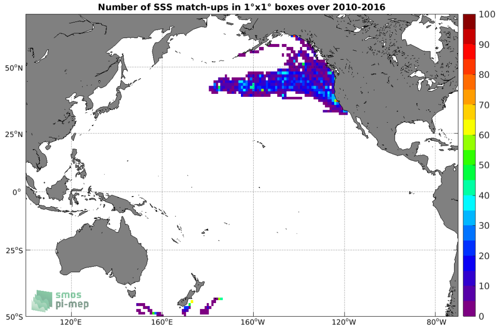
Figure 4: Number of SSS match-ups between Sea mammals SSS and the SMOS SSS L3 v5 - 18 Days (CATDS-CECOS-LOCEAN) SSS product for the Pacific Ocean Pi-MEP region over 1°x1° boxes and for the full satellite product period.
