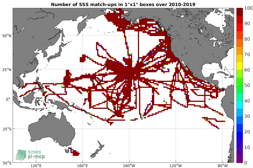
Figure 4: Number of SSS match-ups between TSG (SAMOS) SSS and the SMOS SSS L3 v4 - 9 Days (CATDS-CECOS-LOCEAN) SSS product for the Pacific Ocean Pi-MEP region over 1^\circ \times 1^\circ boxes and for the full satellite product period.
