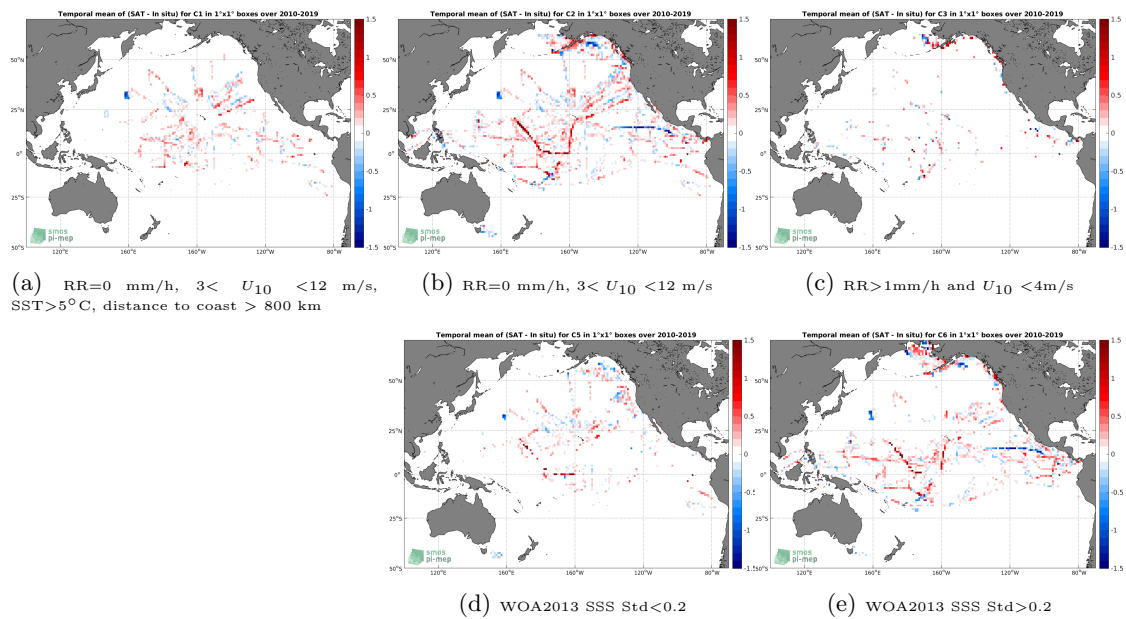
Figure 12: Temporal mean gridded over spatial boxes of size 1^\circ \times 1^\circ of \Delta SSS (SMOS SSS L3 v4 - 9 Days (CATDS-CECOS-LOCEAN) - TSG (SAMOS)) for 5 different subdatasets corresponding to: RR=0 mm/h, 3 < U_{10} < 12 m/s, SST > 5°C, distance to coast > 800 km (a), RR=0 mm/h, 3 < U_{10} < 12 m/s (b), RR > 1mm/h and U_{10} < 4 m/s (c), WOA2013 SSS Std < 0.2 (d), WOA2013 SSS Std > 0.2 (e).
