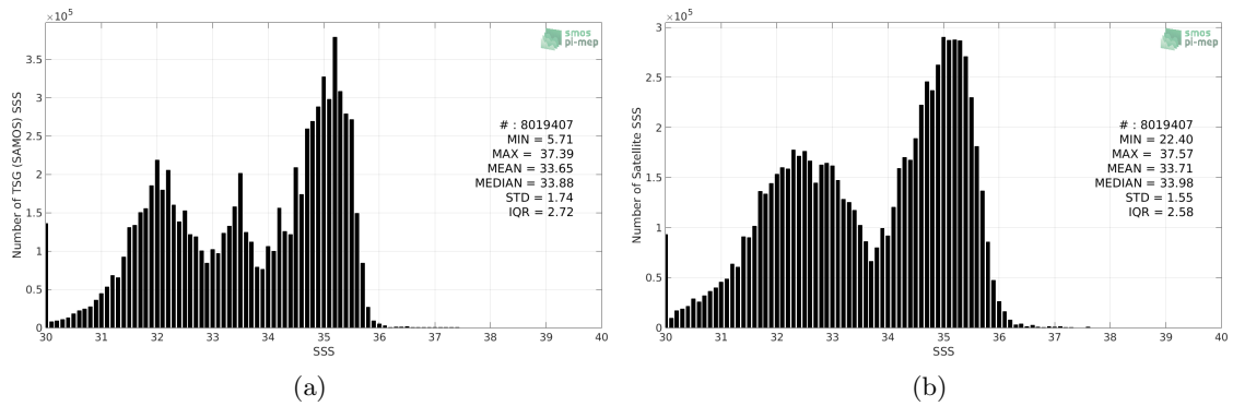
Figure 2: Histograms of SSS from TSG (SAMOS) (a) and SMOS SSS L3 v4 - 9 Days (CATDS-CECOS-LOCEAN) (b) considering all match-up pairs per bins of 0.1 over the Pacific Ocean Pi-MEP region and for the full satellite product period.
