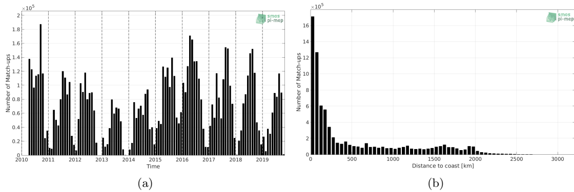
Figure 1: Number of match-ups between TSG (SAMOS) and SMOS SSS L3 v4 - 9 Days (CATDS-CECOS-LOCEAN) SSS as a function of time (a) and as function of the distance to coast (b) over the Pacific Ocean Pi-MEP region and for the full satellite product period.
