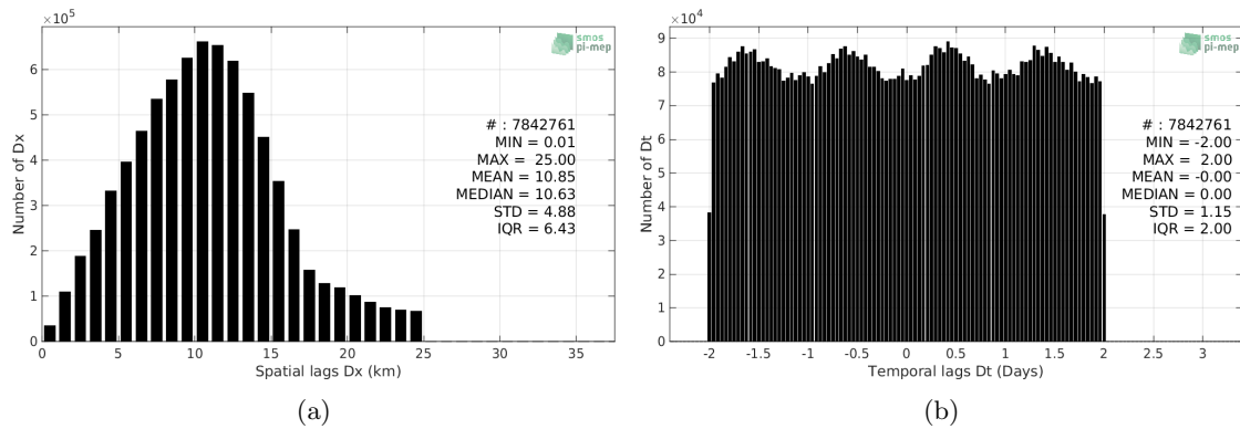
Figure 5: Histograms of the spatial (a) and temporal (b) lags between the time of the TSG-SAMOS measurements and the date of the corresponding SMOS-L3-CATDS-CECOS-LOCEAN-V4-9DAYS-25KM SSS product.
