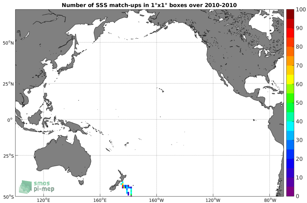
Figure 4: Number of SSS match-ups between TSG-POLARSTERN SSS and the SMOS-L3-CATDS-CECOS-LOCEAN-V4-9DAYS-25KM SSS product for the Pacific Ocean Pi-MEP region over 1^\circ \times 1^\circ boxes and for the full satellite product period.
