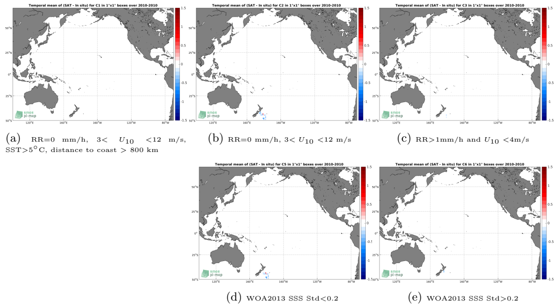
Figure 12: Temporal mean gridded over spatial boxes of size 1^{\circ}\times 1^{\circ} of \Delta\text{SSS} (SMOS-L3-CATDS-CECOS-LOCEAN-V4-9DAYS-25KM - TSG-POLARSTERN) for 5 different subdatasets corresponding to:RR=0 mm/h, 3 < U_{10} < 12 m/s, SST >5^{\circ}\text{C} , distance to coast > 800 km (a), RR=0 mm/h, 3 < U_{10} < 12 m/s (b), RR >1 mm/h and U_{10} < 4 m/s (c), WOA2013 SSS Std <0.2 (d), WOA2013 SSS Std >0.2 (e).
